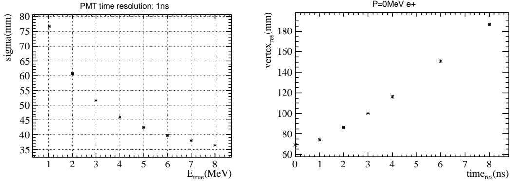
Figure 13-4: Vertex resolution as a function of energy (left) and PMT time resolution (right).
