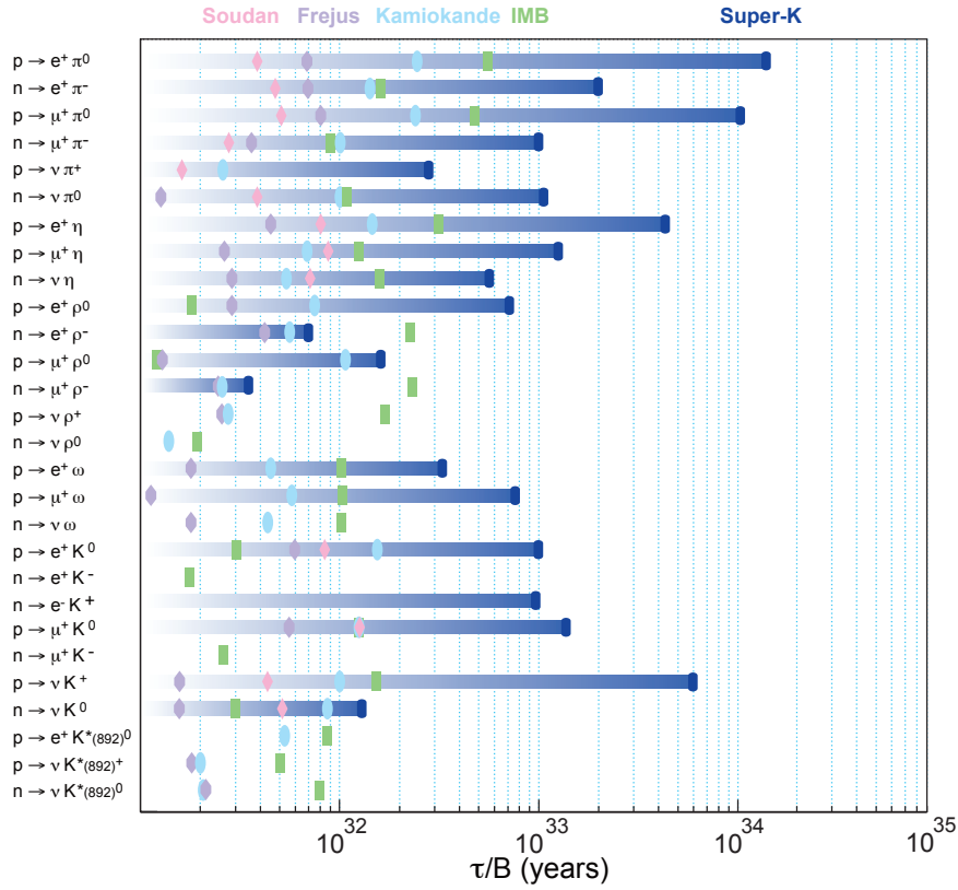
Figure 10-1: The 90% C.L. limits on the nucleon lifetimes in a variety of two-body decay modes of the nucleons [401]. Today’s best limits are mostly from the Super-Kamiokande experiment using the water Cherenkov detector.
