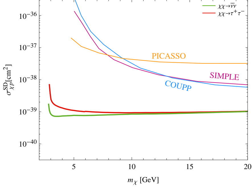
Figure 11-3: The JUNO 2\sigma sensitivity in 5 years to the spin-dependent cross section \sigma_{\chi p}^{\text{SD}} in \text{cm}^2 . The constraints from the direct detection experiments are also shown for comparison.
