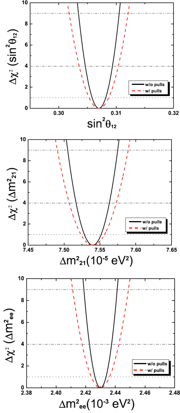
Figure 3-4: Expected accuracy for \sin^2\theta_{12} , \Delta m_{21}^2 and \Delta m_{ee}^2 after 6 years of running at JUNO (i.e., \mathcal{O}(100\text{k}) events). The solid curves are obtained with all other oscillation parameters fixed, while the parameters are set free for the dashed curves.
