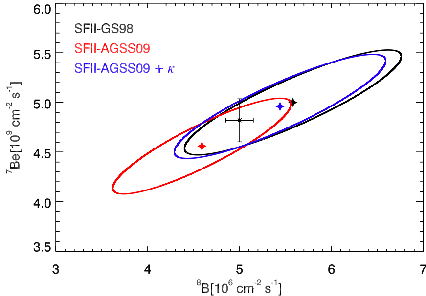
Figure 6-1: Comparison between theoretical predictions and experimental results for the fluxes of ^8\text{B} ( x -axis) and ^7\text{Be} ( y -axis) solar neutrinos. The black, red, and blue ellipses represent the 1\sigma allowed regions, respectively in the high- Z , low- Z and low- Z with increased opacity versions of the SSM. The 1\sigma experimental results for the two fluxes correspond to the horizontal and vertical black bars. Updated version of the figure from [289]. See also [290] and [291].
