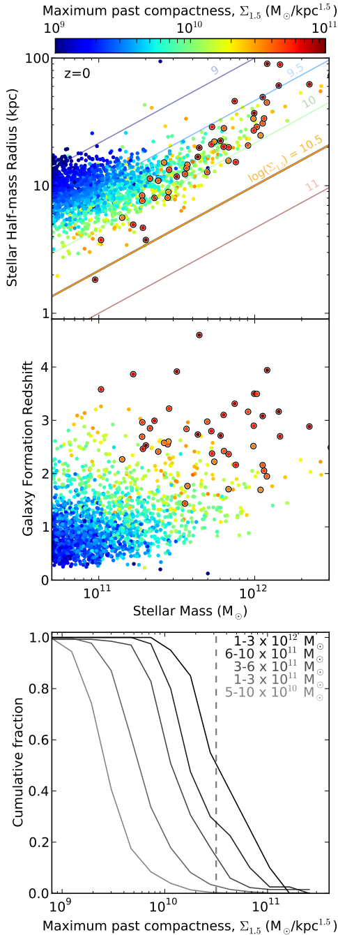
Figure 7. Top panel: Mass-size plane at z = 0 for Illustris galaxies. Color indicates the maximum compactness ( \Sigma_{1.5} ) of all the galaxy’s progenitors along the main branch of its merger tree above 10^{10} M_{\odot} . Solid colored lines mark a constant value of \Sigma_{1.5} . Galaxies which have satisfied \log(\Sigma_{\text{max}}) > 10.5 (the compactness criterion employed in this paper) at any redshift are marked with black circles. (Over half of these are the same 35 which were compact at precisely z = 2 .) Middle panel: Same as above, but with the y-axis indicating the galaxies’ formation redshifts, defined as the median formation redshift over all in-situ stars. Lower panel: Cumulative distribution of \Sigma_{\text{max}} for all galaxies, binned by stellar mass and normalized against the number of galaxies in each bin. Thus, given a value of \Sigma_{1.5} (e.g. 10^{10.5} , marked with a vertical dashed line), one can determine what fraction of galaxies at a given stellar mass have ever achieved that level of compactness. There is a clear relationship between stellar mass and past
