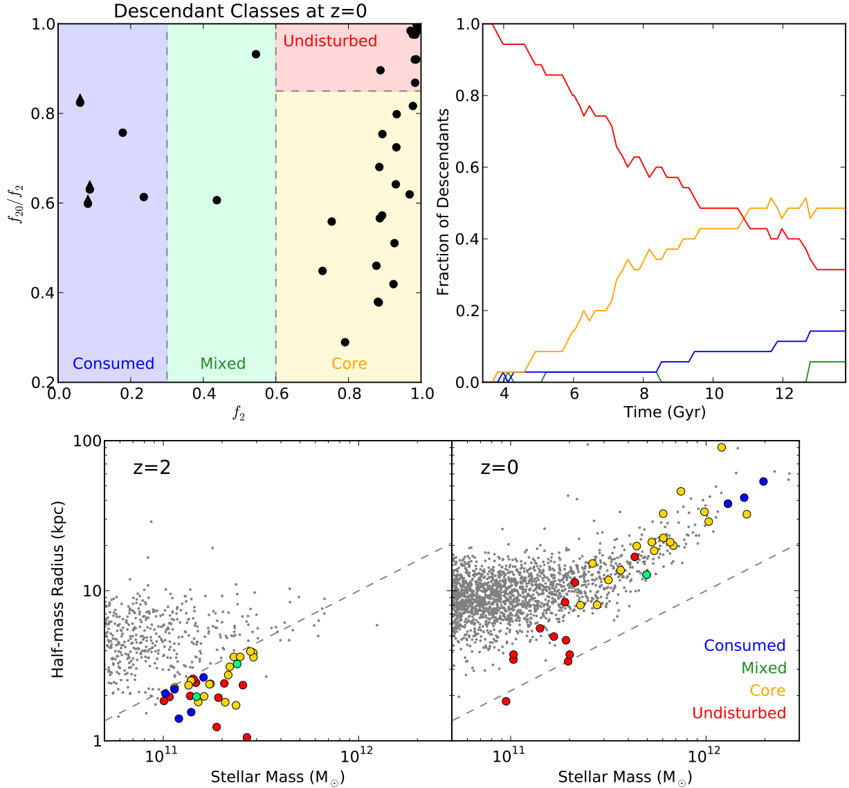
Figure 4. Classification scheme for the descendants of the compact galaxies, as described in Section 4.1, where f_r is the fraction of stars within r kpc that belong to the original z = 2 compact progenitor. Top left: Values of f_2 and f_{20}/f_2 for the final descendants at z = 0 , with grey dashed lines and shaded regions showing how they are classified. An upward-pointing triangle indicates that f_{20}/f_2 > 1 , so the point has been moved down by a factor of two (which does not affect the classification). Top right: The fraction of descendants in each class as a function of time, applying the same scheme to the descendants of the z = 2 compact galaxy population at each redshift. By definition, the galaxies are all initially “undisturbed” at z = 2 , and fall into other classes as they acquire additional stellar mass. Bottom: The compact population at z = 2 ( left ) and their z = 0 descendants ( right ) on the size-mass plane, colored according to final descendant class. In every panel, the color blue indicates galaxies which were “consumed” by a larger galaxy, green indicates galaxies which were “mixed” in major mergers, gold indicates galaxies which are the “core” of a more massive descendant, and red indicates galaxies which survive “undisturbed” to the present day. (Note that there are fewer colored points at z = 0 because some of the compact galaxies have merged together.) The grey dashed line indicates our compactness criterion, \log(\Sigma_{1.5}) > 10.5 .
