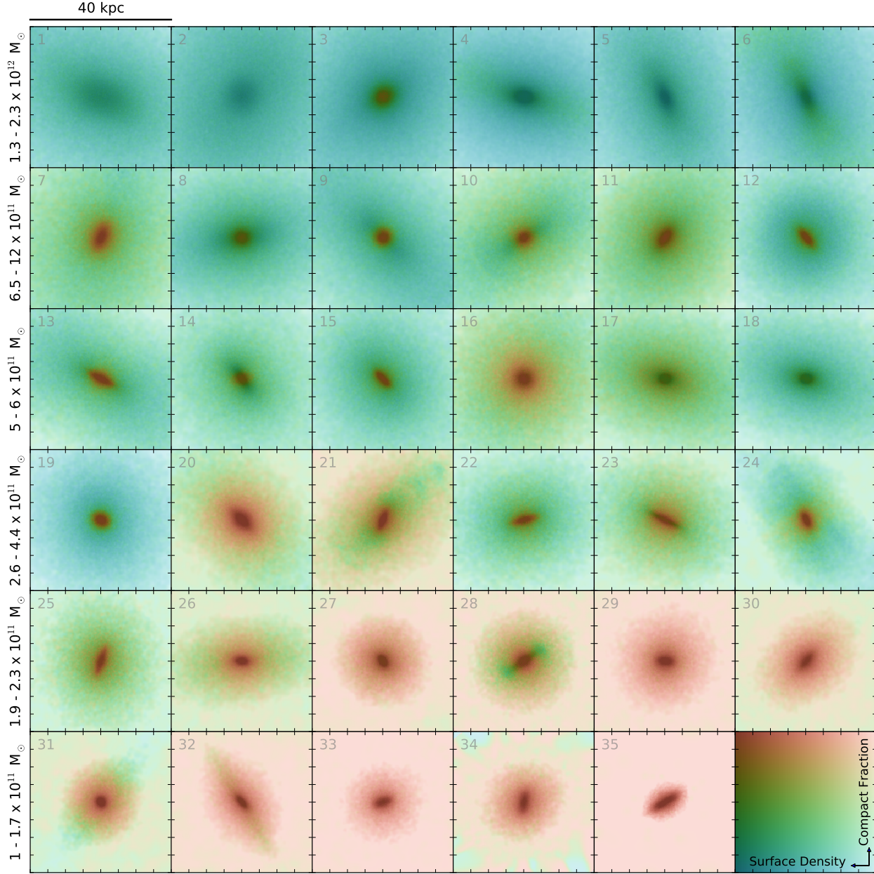
Figure 3. Images of the z = 0 descendants of each of the z = 2 compact galaxies, ordered by descendant mass. A color's intensity is determined by stellar surface density, and its hue by what fraction of the stars along the line of sight belong to the compact progenitor at z = 2 (legend in bottom right). Thus the least massive descendants which have primarily preserved their compact identity appear red, while the most massive descendants which are dominated by other stars appear blue. In many cases, there is a color gradient of red to blue from the inner to outer regions of the galaxy indicating that the compact galaxy is concentrated at the core of its more massive descendant.
