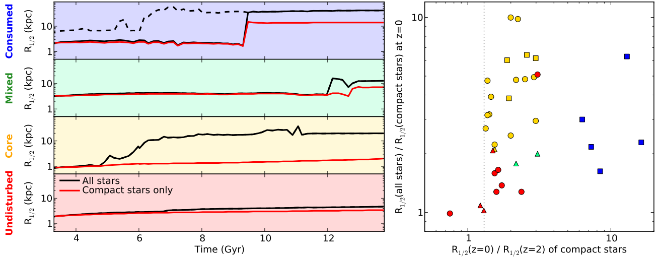
Figure 8. Compact galaxies’ size evolution from z = 2 - 0 . Left panels: Size evolution of the same four galaxies shown in Fig. 5, one from each descendant group. Black lines track the half-mass radius of the descendants’ entire stellar distribution, while the red lines track the half-mass radius of only those stars which were part of the z = 2 compact progenitor. In the “consumed” and “mixed” cases, disruptive mergers increase the compact half-mass radius along with the overall half-mass radius. In the “core” case the compact galaxy remains essentially the same size while the overall half-mass radius increases due to a buildup of additional stellar mass at larger radii, and in the “undisturbed” case the compact galaxy changes very little, having accreted or formed a very small amount of stellar mass since z = 2 . Right panel: For each of the descendants of the 35 compact galaxies, x-axis: Growth in half-mass radius of the compact progenitor’s stars, i.e. the ratio between the value of the red line at z = 0 and z = 2 . The vertical dashed line shows the estimated 30% growth from mass loss and numerical effects (see Appendix). y-axis: Half-mass radius of all stars relative to the half-mass radius of compact stars, i.e. the ratio between the black and red lines at z = 0 . Higher values in the x -direction indicate disruption of the compact core, while higher values in the y -direction indicate the presence of ex-situ stars at large radii. Symbol shapes and colors are the same as in Figs. 4 and 6.
