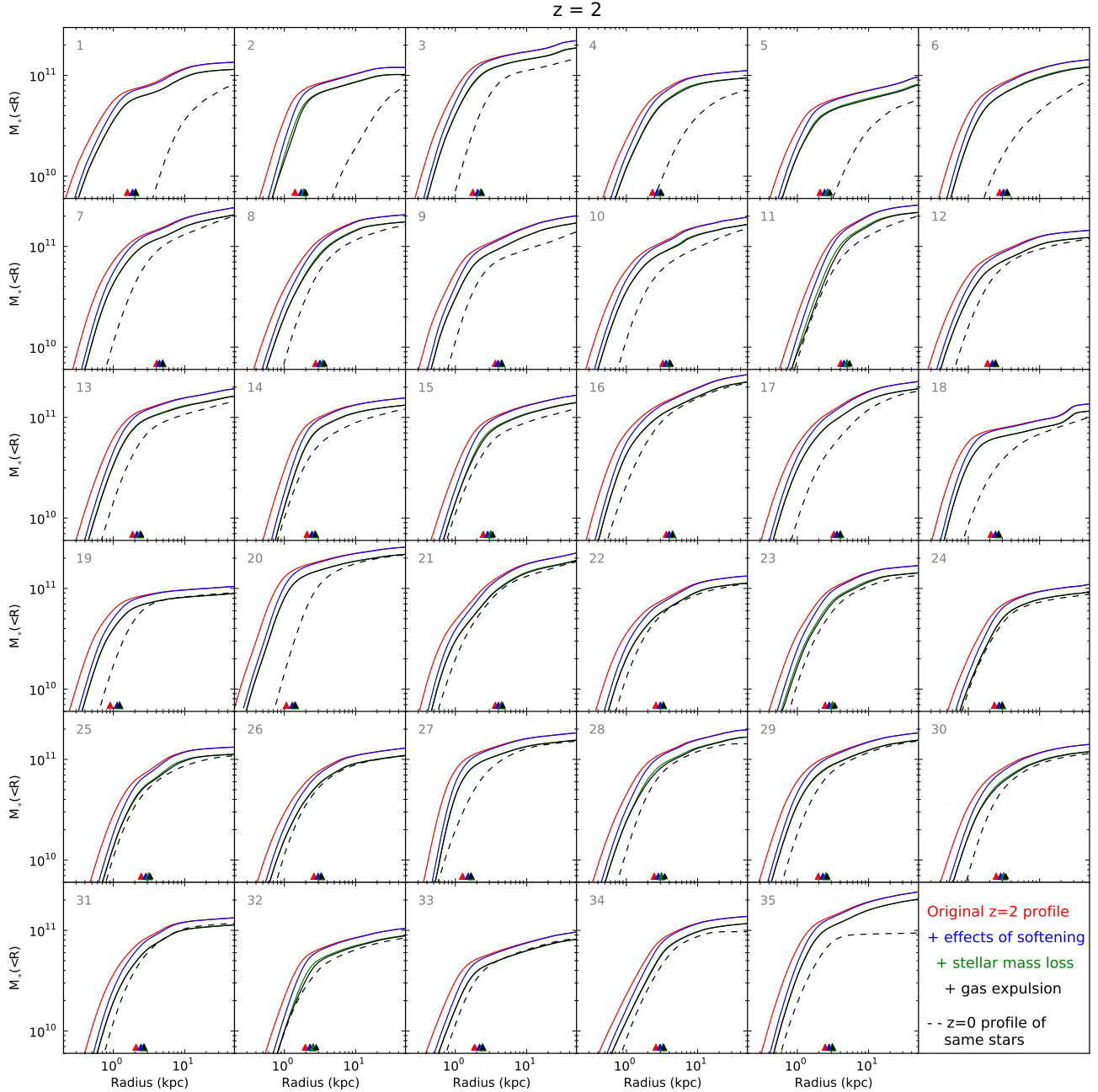
Figure A2. Cumulative stellar mass profiles of compact galaxies at z = 2 , arranged in the same manner as in Fig. A1. In each panel, the red line shows the stellar mass profile of the z = 2 compact galaxy. Each of the other solid lines show the cumulative effect on that original profile when ( blue ) the stellar and dark matter gravitational softening lengths are changed to their z = 0 values, ( green ) the stars lose 15% of their mass, and ( black ) any gas in the galaxy is expelled, assuming that the adiabatic invariant rM_{\text{eff}}(r, \epsilon) is preserved. Triangles at the bottom of each panel mark the half-mass radii corresponding to these profiles. On average, changing the softening length increases the half-mass radius by about 15%, stellar mass loss then increases it by 12%, and gas expulsion by another 3%. The dashed black line in each panel shows the actual stellar profile of these stars within their descendant at z = 0 . In several cases, the dashed and solid black lines are very similar, showing that the aforementioned effects are responsible for the change in the galaxy’s shape. In most cases, however, the compact galaxy is disturbed in some way (through e.g. mergers).
