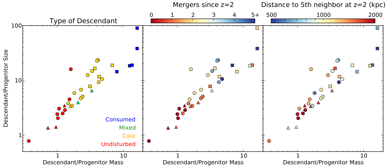
Figure 6. Growth in size and mass among the compact galaxy population from z = 2 - 0 . In all three panels, the x-axis shows the mass growth (ratio of a galaxy’s stellar mass at z = 0 and z = 2 ) and the y-axis shows the size growth (ratio of the stellar half-mass radii). As in Figure 1, triangles indicate that a galaxy is a satellite at z = 0 and squares indicate that the compact galaxy does not lie along the main progenitor branch of its descendant. Left panel: color refers to the type of descendant, as defined in Section 4.1. Middle panel: color indicates the number of mergers since z = 2 with stellar mass ratios of <10:1 . Right panel: color indicates z = 2 environment, i.e. the distance to the 5th nearest neighbor with an r-band magnitude of at least -19.5 (about 10^9 M_{\odot} ). The most isolated galaxies (red on the rightmost panel) tend to experience fewer mergers (red on the middle panel) and thus experience little mass growth and are essentially undisturbed. Two notable exceptions are satellite galaxies, which fell into another DM halo in the intervening time period but have not merged with the central galaxy.
