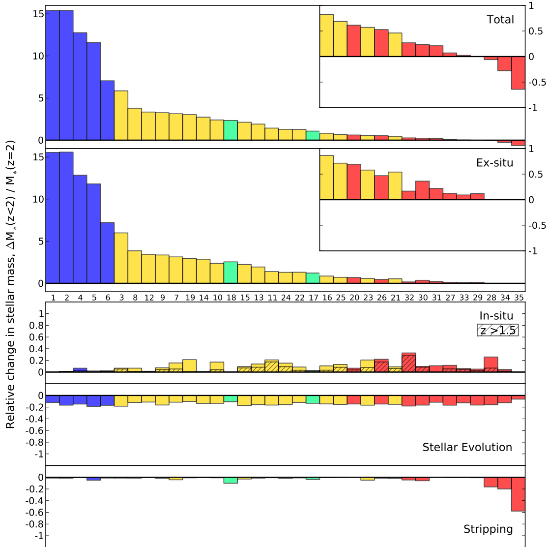
Figure 2. The amount by which each compact galaxy’s stellar mass changes between z = 2 and z = 0 relative to its z = 2 mass ( top panel ), broken down into the contributions from ex-situ (i.e. accreted) stars ( second panel ), in-situ star formation ( third panel ), stellar mass loss ( fourth panel ), and stripping ( bottom panel ). In the third panel, in-situ star formation which occurred between our selection redshift of z = 2 and z = 1.5 is indicated by hashed regions. The galaxies are ordered by decreasing change in stellar mass, and their index in Figure 3 is noted in the middle of the figure. Colors indicate the descendant class from Section 4.1. Note that the top two panels are scaled differently from the bottom three, with insets on a comparable scale when the change in mass drops below 100%. In general the change in mass is dominated by ex-situ stars, but at the low-mass end where the galaxies change their mass by less than 50%, other effects become significant.
