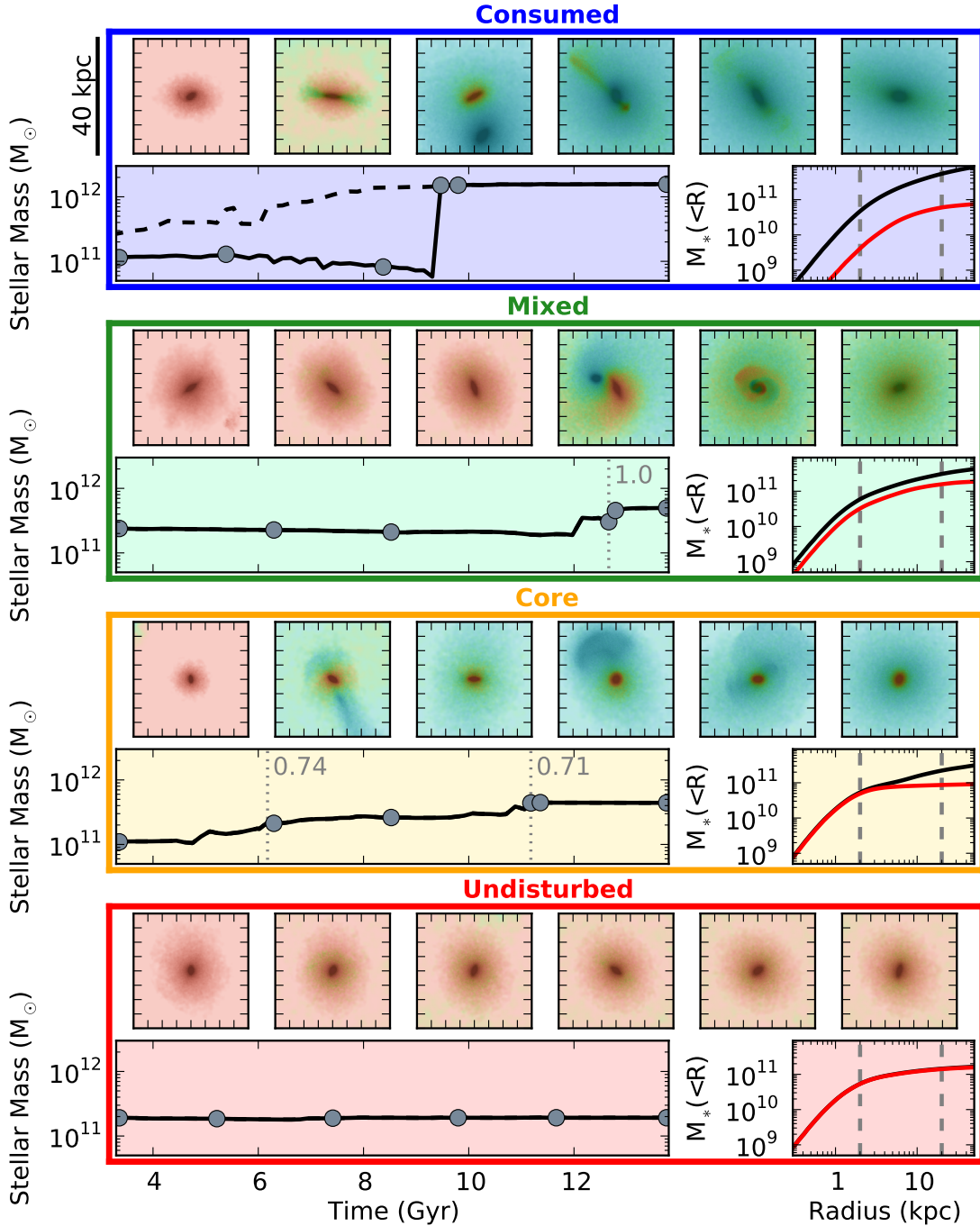
Figure 5. Evolution of an individual galaxy from each of the four descendant types. (From top to bottom, these are galaxies 4, 17, 19, and 29.) For each of these examples, the panel on the left shows the evolution of stellar mass with time in a solid black line, with dashed lines drawn for merger partners where applicable. Large grey points mark the times corresponding to the six images directly above, which have the same color scheme as in Figure 3. The rightmost panels show the cumulative stellar mass profiles for the final z = 0 descendants. Black lines include all stellar mass, while the red lines only include star particles that were present in the compact progenitor at z = 2 . The ratio of these two lines is the f_r discussed in Section 4.1 used to classify the descendants, and grey dashed lines show where f_2 and f_{20} were measured. Each of these examples is demonstrative of the kind of events (or lack thereof) that characterize each descendant type.
