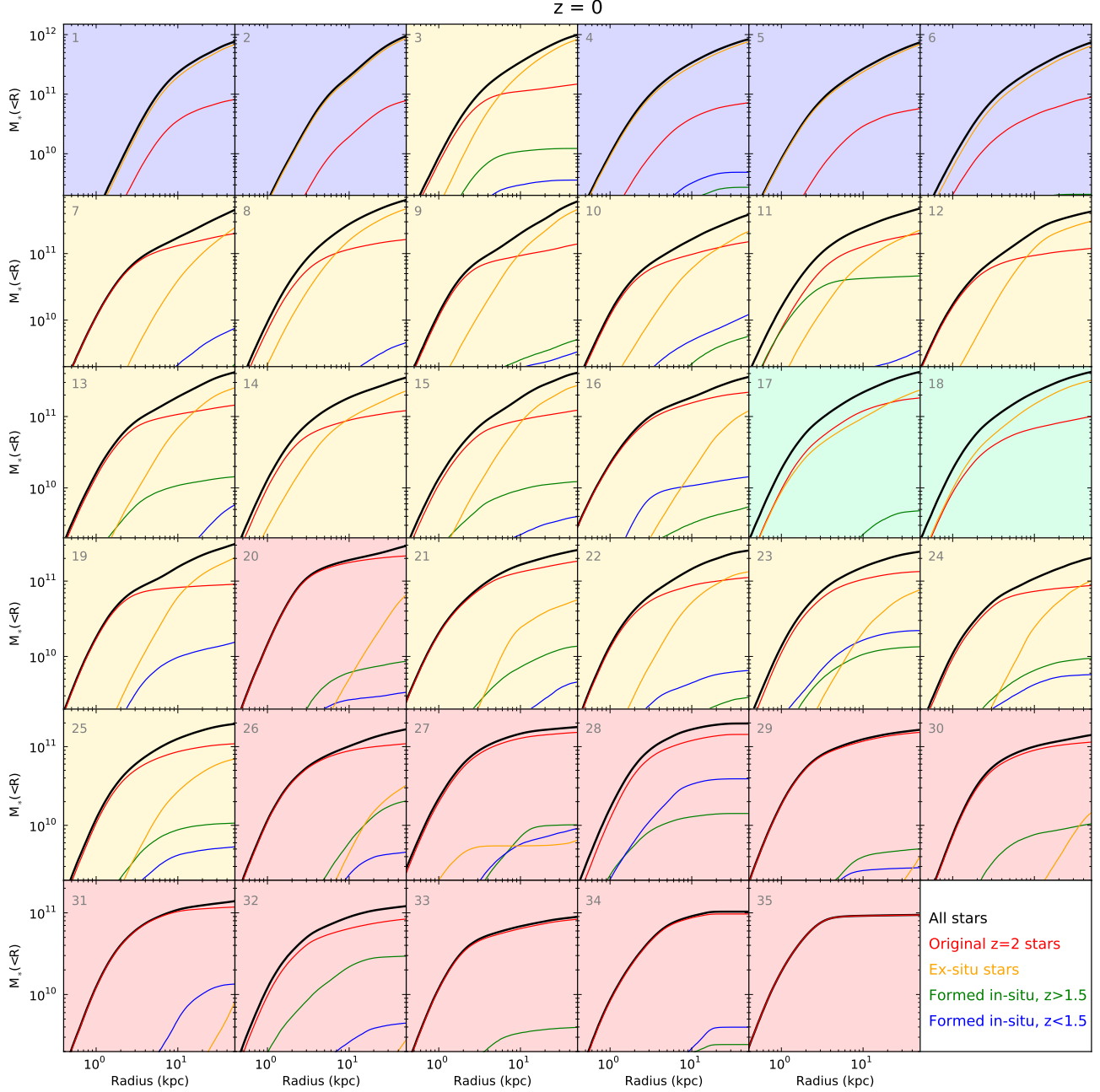
Figure A1. Cumulative stellar mass profiles for the descendants of the compact galaxies at z = 0 . Galaxies are ordered by decreasing stellar mass, as in Figure 3. The total profiles are shown in black, and the colored lines separate the stars into ( red ) the original stars which were present in the z = 2 compact progenitor, ( orange ) ex-situ stars acquired after z = 2 , ( green ) stars formed in-situ between z = 2 and z = 1.5 , and ( blue ) stars formed in-situ after z = 1.5 . Background shading indicates the descendant type as in Fig. 4.
