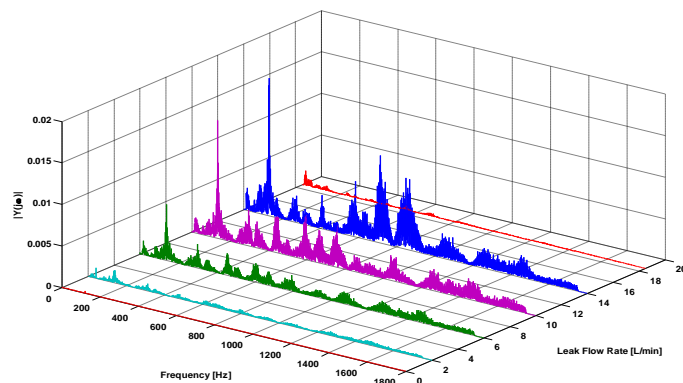
Figure 4: Effect of leak flow rate on frequency spectrum; DPT-no pipe flow
