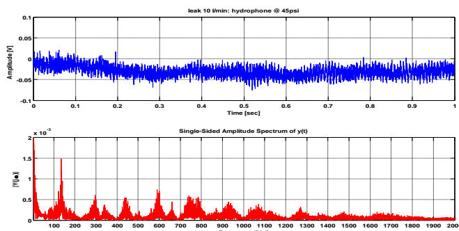
(b) Hydrophone
