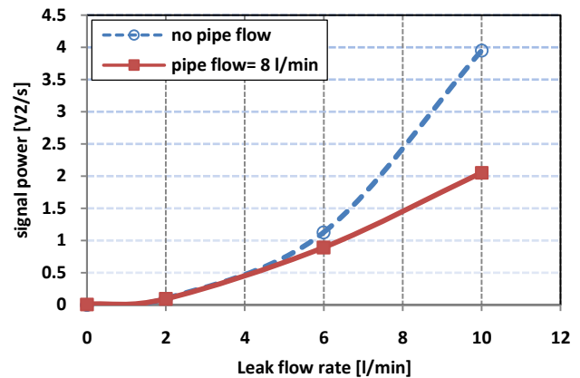
Figure 8: Calculated power of leak time signal with and without pipe flow-hydrophone
