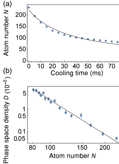
FIG. 3. (a) Atom number extracted from the total scattering rate into the cavity. The solid line is a two-body loss model fitted to the experimental data with a fitted two-body loss coefficient of 0.12(1) 1/s . (b) Phase space density D as a function of the remaining atom number. A linear fit between \ln(D) and \ln(N) is plotted as a solid line. The fit gives \gamma = 5.0(3) .
