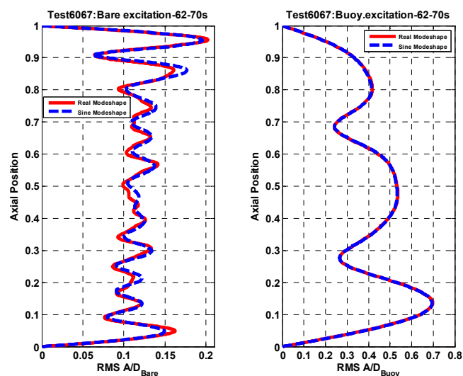
Figure 13. An example comparison of reconstructed displacements with sinusoidal and real mode shapes. The data is from Test 6067 with L_c/L_b = 2/2 at 1.0m/s uniform flow. Band-pass filter in frequency for the bare excitation and the buoyancy excitation is from 0.5 \times \text{Freq}_{\text{Bare}} to 1.5 \times \text{Freq}_{\text{Bare}} and 0.5 \times \text{Freq}_{\text{Buoy}} to 1.5 \times \text{Freq}_{\text{Buoy}} , respectively; And filter bandpass values are \pi/L to 29\pi/L in wave number for both excitations.
