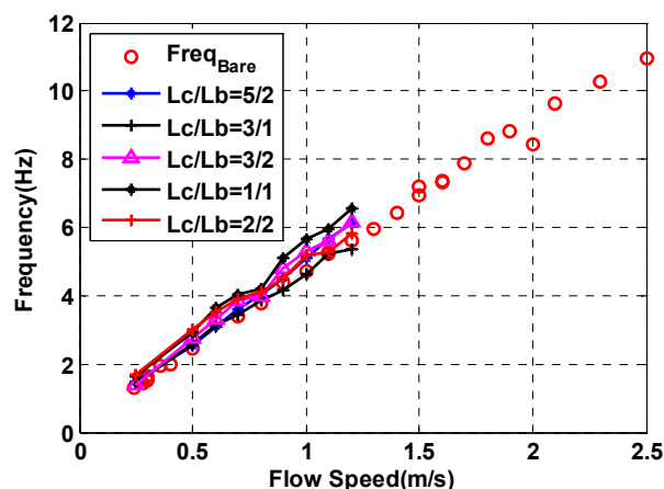
Figure 12. Excitation frequencies associated with smaller diameter in both bare medium pipe (red circle) and five buoyancy configurations (line+symbols) are plotted against flow speed.
