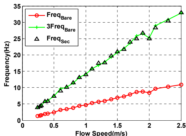
Figure 3. Bare excitation ( Freq_{Bare} ) and secondary frequencies ( Freq_{Sec} ) are plotted against flow speed for uniform flow for the bare medium pipe ( D=30\text{mm} ). The green line represents the theoretical value of three times of the excitation frequency for bare medium pipe and black triangle represents the secondary peak frequency measured in the experiment.
