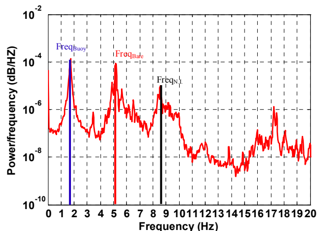
Figure 5. An example curvature power spectrum for the medium pipe with staggered buoyancy modules. The data is the averaged spectrum of 30 curvatures at 1.0m/s uniform flow, corresponding to Test 6067 with L_c/L_b=2/2 .
