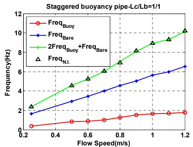
Figure 9. Buoyancy excitation frequency, bare excitation frequency and nonlinear interaction frequency in the curvature power spectrum are plotted against flow speed. The data is the averaged spectrum of 30 curvatures, corresponding to the buoyancy configuration L_c/L_b = 1/1 . The green line represents the theoretical value of 2\text{Freq}_{\text{Buoy}} + \text{Freq}_{\text{Bare}} and black triangle represents the nonlinear interaction frequency measured in the experiment.
