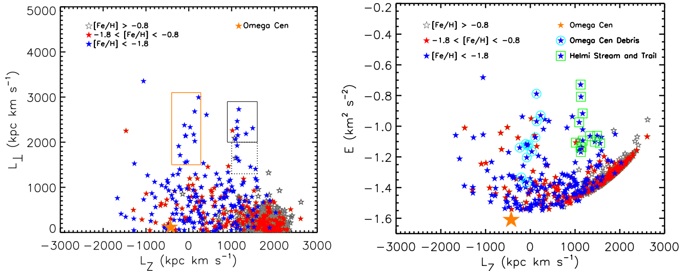
Figure 12. Left panel: distribution of the angular momentum components L_{\perp} and L_z for the combined sample of stars over three ranges of metallicity, as shown in the legend. The solid and dotted black boxes denote the region of the clumps that are likely associated with the Helmi et al. stream and trail, respectively. The orange box represents the region of the putative debris stream associated with the \omega Cen globular cluster. The position of this cluster in this diagram is indicated by the large orange star. Stars with errors exceeding 50 \text{ km s}^{-1} in any of the individual derived components of motion are excluded. Right panel: Lindblad diagram of the distribution of the total energy E (in units of 10^5 ) as a function of the vertical angular momentum L_z over three ranges of metallicity, as shown in the legend. Likely members of the Helmi et al. stream and its trail are highlighted with light-blue circles; stars that are likely members of the putative \omega Cen debris stream are indicated by light-green squares. The position of this cluster in this diagram is indicated by the large orange star. Stars with errors exceeding 50 \text{ km s}^{-1} in any of the individual derived components of motion are excluded.
