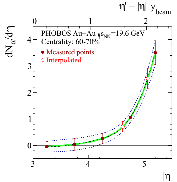
FIG. 12. Spline polynomial fits (lines) to \alpha yields from Au+Au peripheral (60%–70%) data (filled circles). Interpolated points at \eta' = 1.57 and \eta' = 2.02 are shown as open circles. The scale on the upper x axis shows \eta' \equiv |\eta| - y_{beam} . The dashed and green lines show fits using polynomials of different order. The outer dotted lines represent a fit to points at the extreme of the systematic uncertainty bands.
