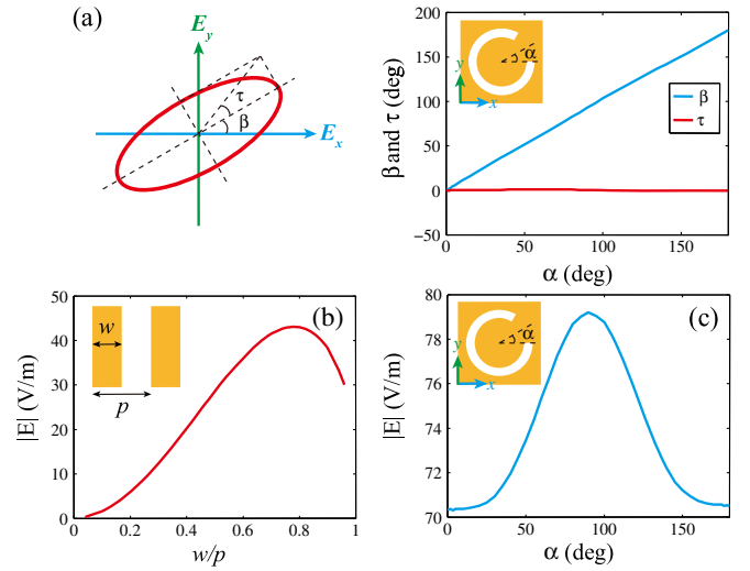
FIG. 4. (a) Illustration of the polarization ellipse (left panel) and the calculated orientation angle \beta and ellipticity angle \tau of the emitted light (right panel). (b),(c) The amplitude of Smith-Purcell emission from 1D metallic gratings and C -aperture metasurfaces, respectively. The periodicity of the grating is the same as the metasurface ( p = 50 \mu\text{m} ).
