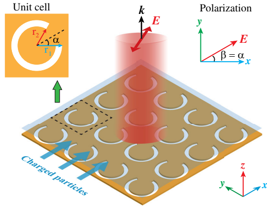
FIG. 1. Schematic of the Smith-Purcell emission from a Babinet metasurface. A uniform sheet of charged particles moves closely parallel to the metasurface along the +x axis. The Babinet metasurface generates linearly polarized radiation, propagating along the surface normal in the +z direction. The direction of the electric field has an angle \beta with respect to the +x axis, which is determined by the azimuthal rotating angle \alpha of the C -aperture resonators.
