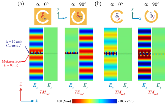
FIG. 3. Electric field distributions of the Smith-Purcell emission from (a) C -aperture and (b) C -ring metasurfaces. A sheet current with the parameters v_0 = c/4 , I_0 = 1 A/m described by Eq. (1) acts as the source in simulation. The sheet current is located at 10 \mu\text{m} above the metasurface.
