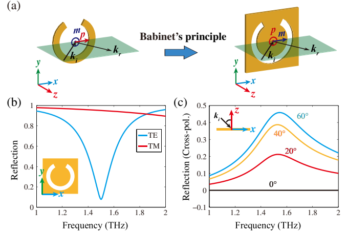
FIG. 2. The responses of the C -ring and C -aperture metasurfaces under illumination of propagating waves. (a) Illustration of the dipolar behaviors of a C -ring resonator and of its complementary structure, namely, a C -aperture resonator. (b) Reflection coefficients of the C -aperture metasurface at normal incidence. TE and TM modes correspond to the incident fields of E_y and H_y , respectively. (c) Cross-polarization reflection coefficients ( r_{12} ) of the C -aperture metasurface at oblique incidence of TM waves.
