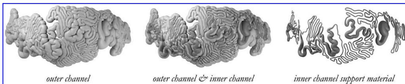
FIG. 8. Visualization of smaller scale test piece used. The image on the left shows the actual shape of the printed piece. The image in the middle and the image on the right visualize how the support material ( blue ) is distributed and printed inside the wearable to achieve a hollow channel.
