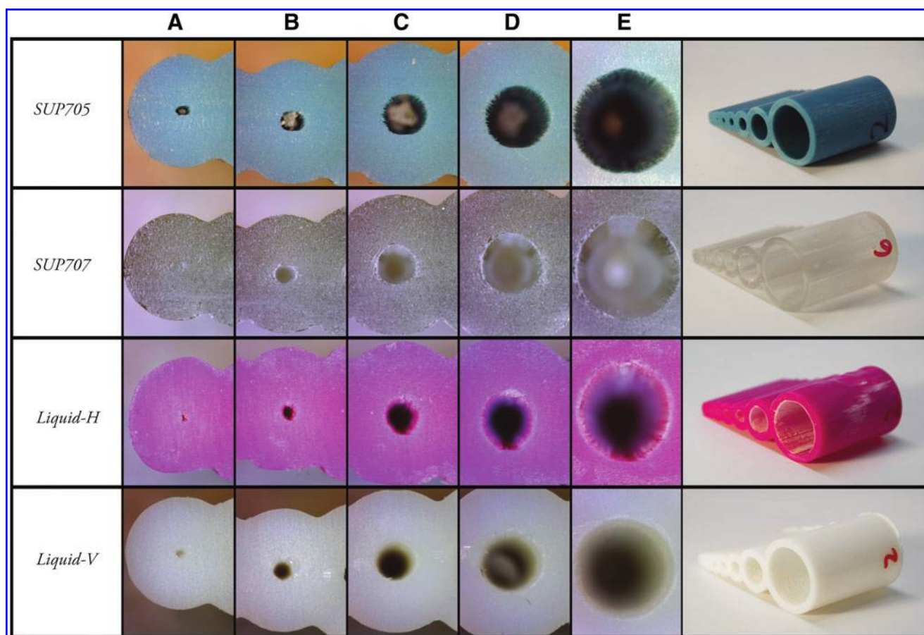
FIG. 7. Representative optical images of test piece cross sections that were printed using the three support material methods. Color images available online at www.liebertpub.com/3dp
