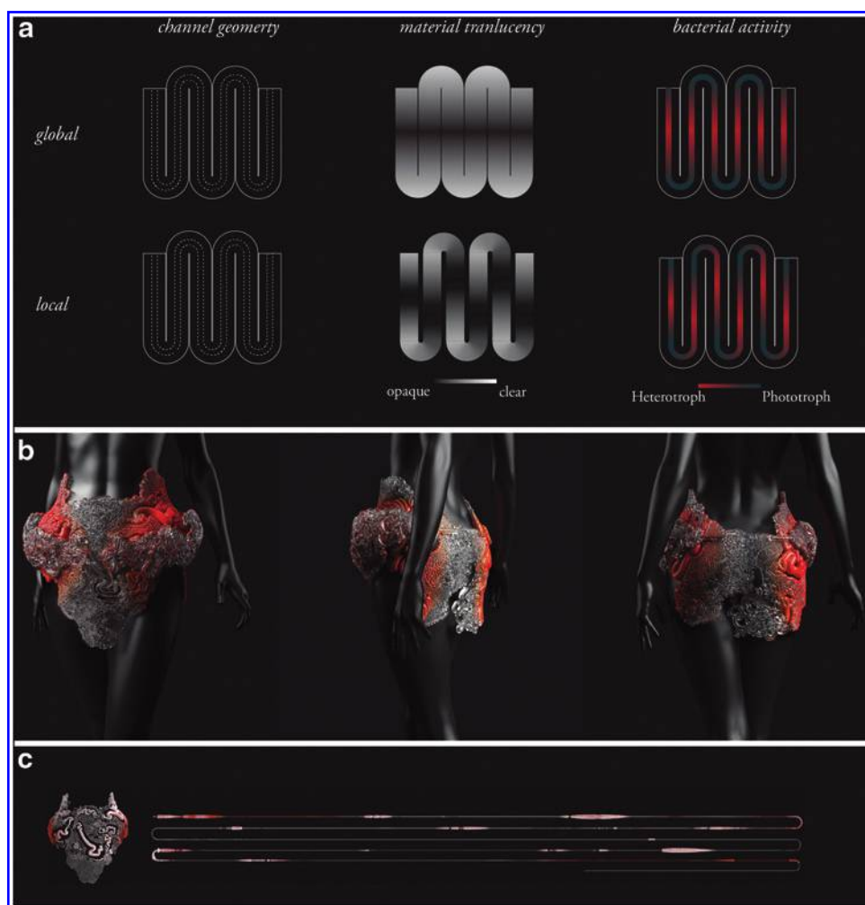
FIG. 5. (a) The desired effect of material transparency on microbial activity. In translucent regions, the coculture receives light, increasing phototrophic activity (right column). In opaque regions, the coculture is dark and the heterotrophs would consume the photosynthates, thus increasing their metabolic activity. Transparency can be controlled globally, as shown in the upper middle column, independently of the strand, or locally, shown in the lower middle column, using path-length parameterization as a guide for material distributions. (b) Implementation of the global heterogeneous modeling approach on the wearable. (c) Visualization of the unfolded strand showing how the overall (“global”) source-based approach influences local changes in opacity along the strand Figure 6. Color images available online at www.liebertpub.com/3dp
