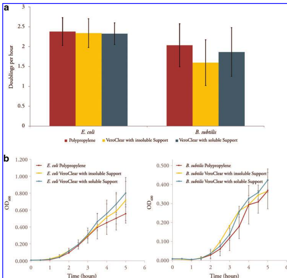
FIG. 9. (a) Comparison of growth rates (doublings per hour) of Escherichia coli and Bacillus subtilis in various tube materials. Error bars represent the standard deviation between at least six biological replicates. Representative growth of E. coli (b, left) and B. subtilis (b, right) in different tubes. Error bars represent the standard deviation among three biological replicates grown on the same day. Color images available online at www.liebertpub.com/3dp
