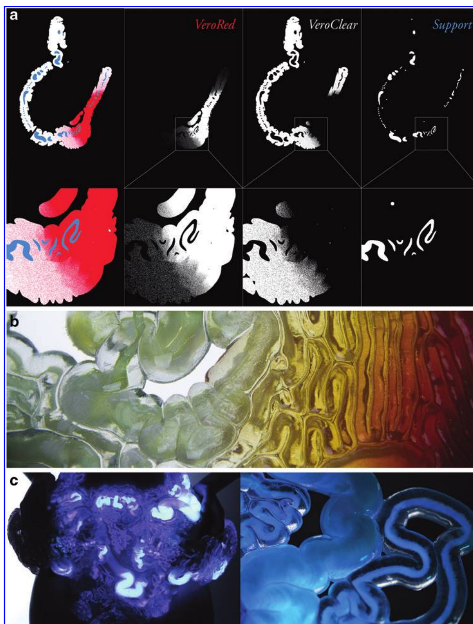
FIG. 6. (a) A single layer of the 3D material deposition description ( top ) highlighting areas where optical gradients are modeled ( bottom ). (b) Actual fabricated optical gradients with filled internal channels. (c) Hollow channels filled with chemiluminescent liquid for the purpose of visualization. Color images available online at www.liebertpub.com/3dp
