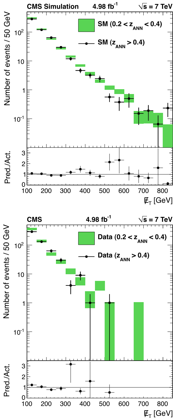
Fig. 12 The \cancel{E}_T distributions of events in the z_{ANN} signal region (solid circles) and sideband (green bars) for simulated SM (top) and data (bottom) events. The distributions are normalized in the \cancel{E}_T sideband, 150 < \cancel{E}_T < 350 GeV (regions A and C for the two distributions respectively). The rightmost histogram bin includes overflow. The small lower plots show the ratio of normalized sideband to signal yields (Color figure online)
