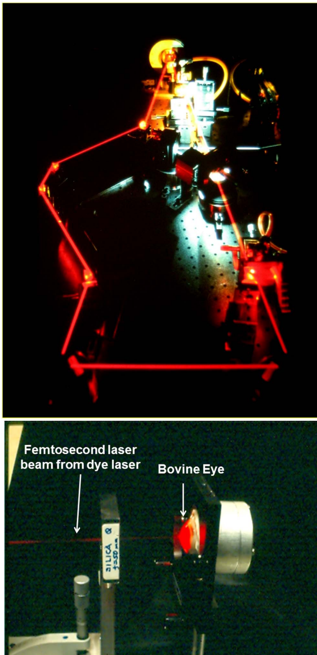
FIGURE 2. (Top) The colliding pulse femtosecond dye laser was state of the art in the 1980s and could generate record pulse durations of less than 100 fs. This technology enabled fundamental studies of ultrafast phenomena in physics, chemistry, and photobiology. We began to explore biomedical applications at MIT in the mid-1980s. (Bottom) Early experiment measuring femtosecond light echoes in an ex vivo bovine eye.
