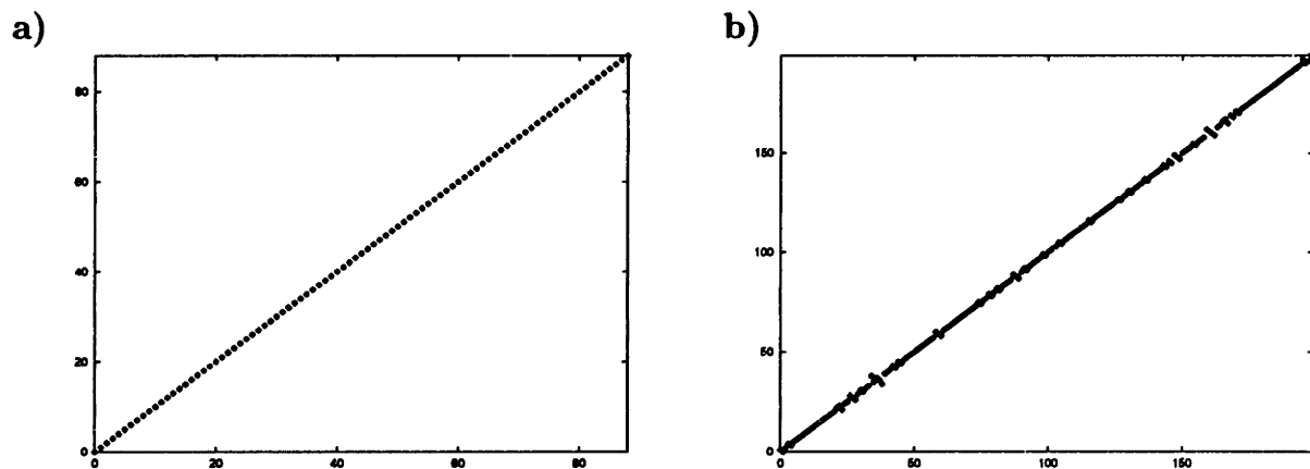
Figure 4.11: Test of the framework and placement map construction algorithms on a 200-marker simulated data set. a) Comparison of our 89-marker framework map to the correct order of the same markers. b) Comparison of the 200-marker placement map (including the framework map from a) to the “true” order of the markers along the simulated chromosome. Each placement marker is shown in its most-likely map position; other positions may be nearly-equally likely.
