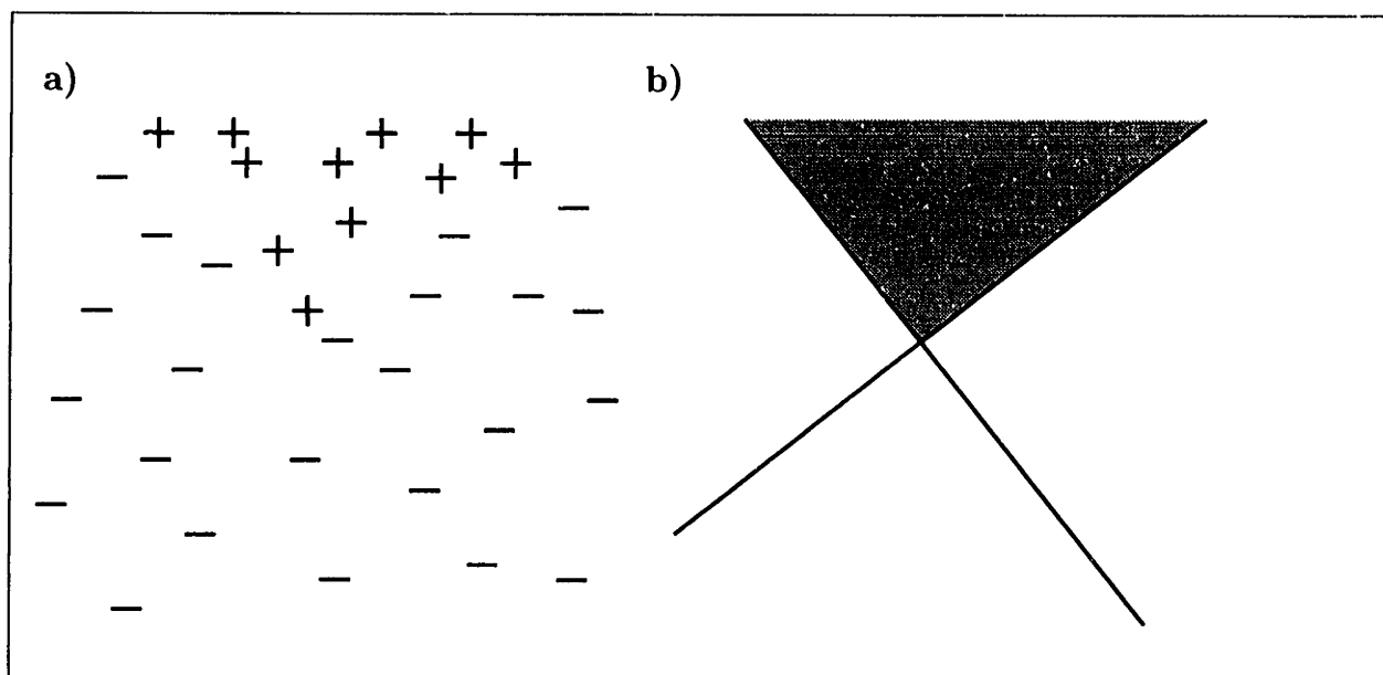
Figure 1.1: Learning the intersection of two halfspaces in the plane. a) The learner sees only labeled examples chosen at random from the domain of points in the plane. b) The learner’s goal is to determine the underlying target concept, shown here. All positive examples are chosen from the shaded region.
