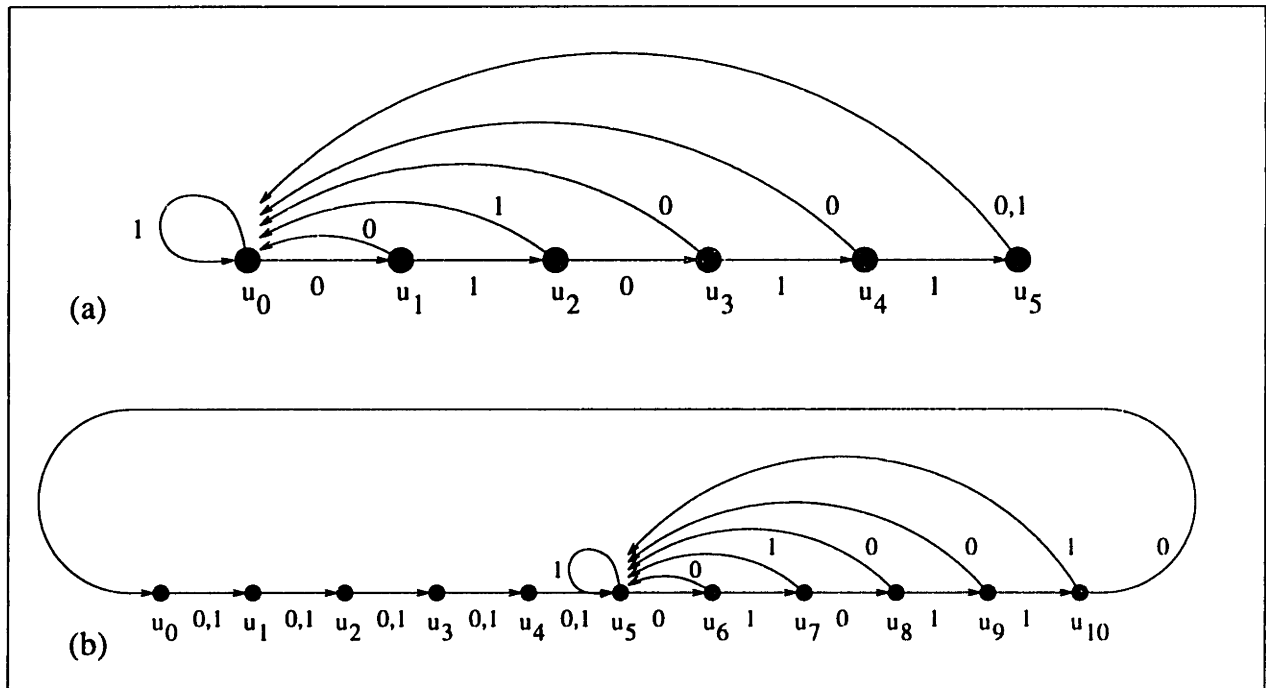
Figure 3.3: (a) A combination-lock, whose combination is 0, 1, 0, 1, 1. (b) A graph in \mathcal{R}_{11} . Graphs in \mathcal{R} = \cup_{n=1}^{\infty} \mathcal{R}_n cannot be learned by one robot with a constant number of pebbles.
