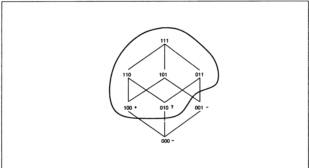
Figure 2.3: The +, −, and ? symbols respectively indicate positive, negative, and “I don’t know” answers to membership queries. The first positive counterexample is 110 ; vectors 010 , 100 , and 000 are queried. If the second counterexample is 011 , vector 010 would be queried again.
