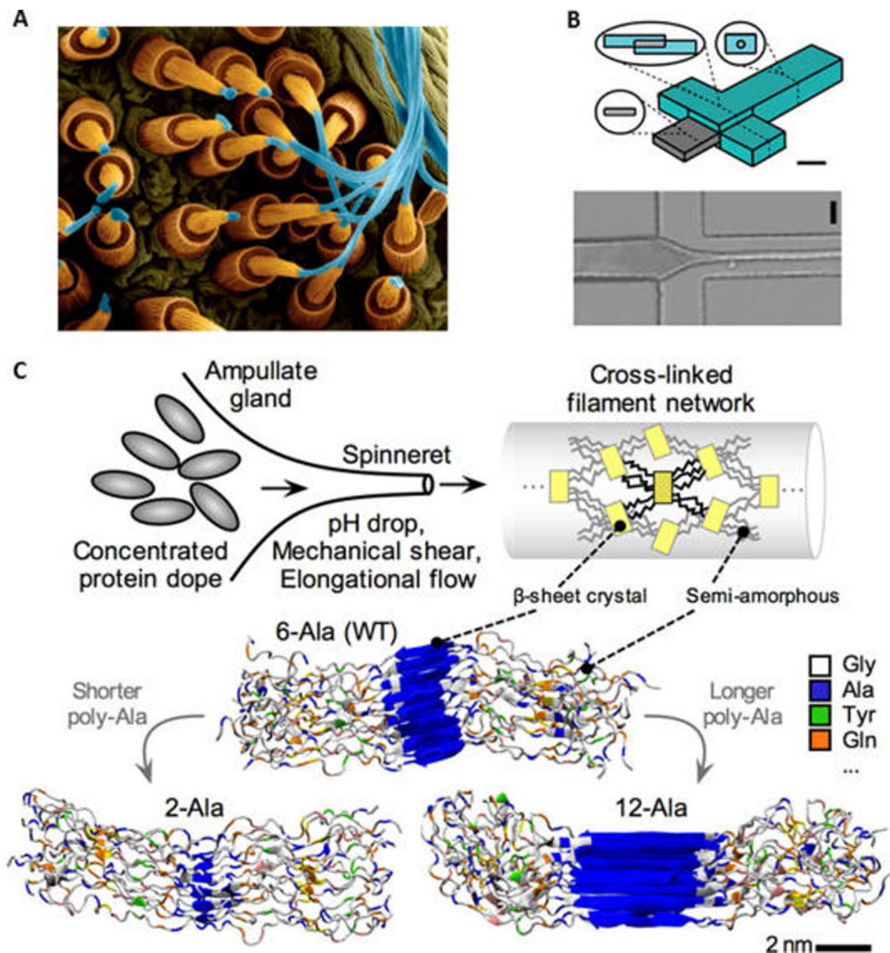
Figure 6. Fiber formation from spider silk proteins upward: (A) Natural. Copyright Dennis Kunkel Microscopy, Inc./Visuals Unlimited/Corbis. (B) Bioinspired microfluidic process, which used microfluidic for silk worm silk. (Adapted with permission from ref 103. Copyright 2011 American Chemical Society.) Similar principles apply to the production of spider silk. (C) Detailed molecular view. (B) Regenerated silk fibroin (RSF) solution flows through the central channel while acidic poly(ethylene-oxide) (PEO) solution flows through the side channels. As these solutions combine and flow in the device, the PEO solution surrounds the
