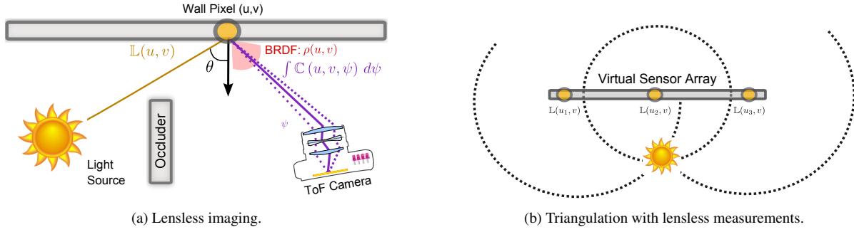
Fig. 2: Recasting time of flight cameras into a (virtual) sensor array. (a) Mapping out the transport paths from a light source to coordinates (u, v) on the wall. The wall serves as a virtual sensor array (VSA). By taking a picture of the virtual sensor we obtain the measurement model. The goal of Section 4.1 is to extract \mathbb{L}(u, v) from the ToF camera measurements. (b) Given such measurements, a reasonable next step is to use backprojection to localize the source. This second step connects to lensless transient imaging, as introduced in [Wu et al. 2014].
