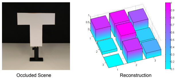
Fig. 7: Imaging around the corner. (left) We use the same scene from Figure 6a but replace the moving ping pong ball with a “T” shaped object. (right) Using pseudoinverse beamforming, we are able to recover the hidden image. The height represents confidence in a given voxel.
