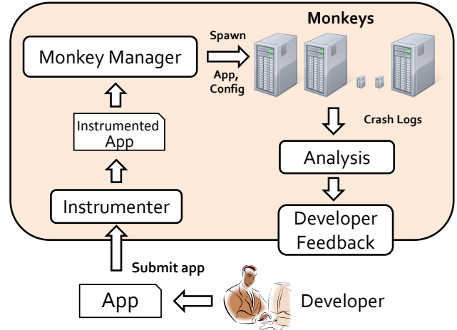
Figure 8: VanarSena Architecture.
