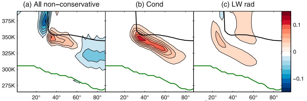
FIG. 8. The total nonconservative contribution to the eddy enstrophy budget, -\overline{Q^*}_{\partial_\theta \overline{P}^{2*}}/2 + \overline{S \overline{P}^*} - \overline{Q \overline{P}^*}_{\partial_\theta \overline{P}^*} - \overline{\rho_\theta^{-1} \partial_\theta \rho_\theta \overline{Q \overline{P}^*}}/2 , for (a) all nonconservative processes, (b) large-scale condensation only, and (c) longwave radiation only. The total diabatic contribution in (a) includes the processes in (b) and (c), as well as moist convection, shortwave radiation, hyperdiffusion of temperature, boundary layer diffusion, and hyperviscosity. The contour interval and black and green lines are as in Fig. 7.
