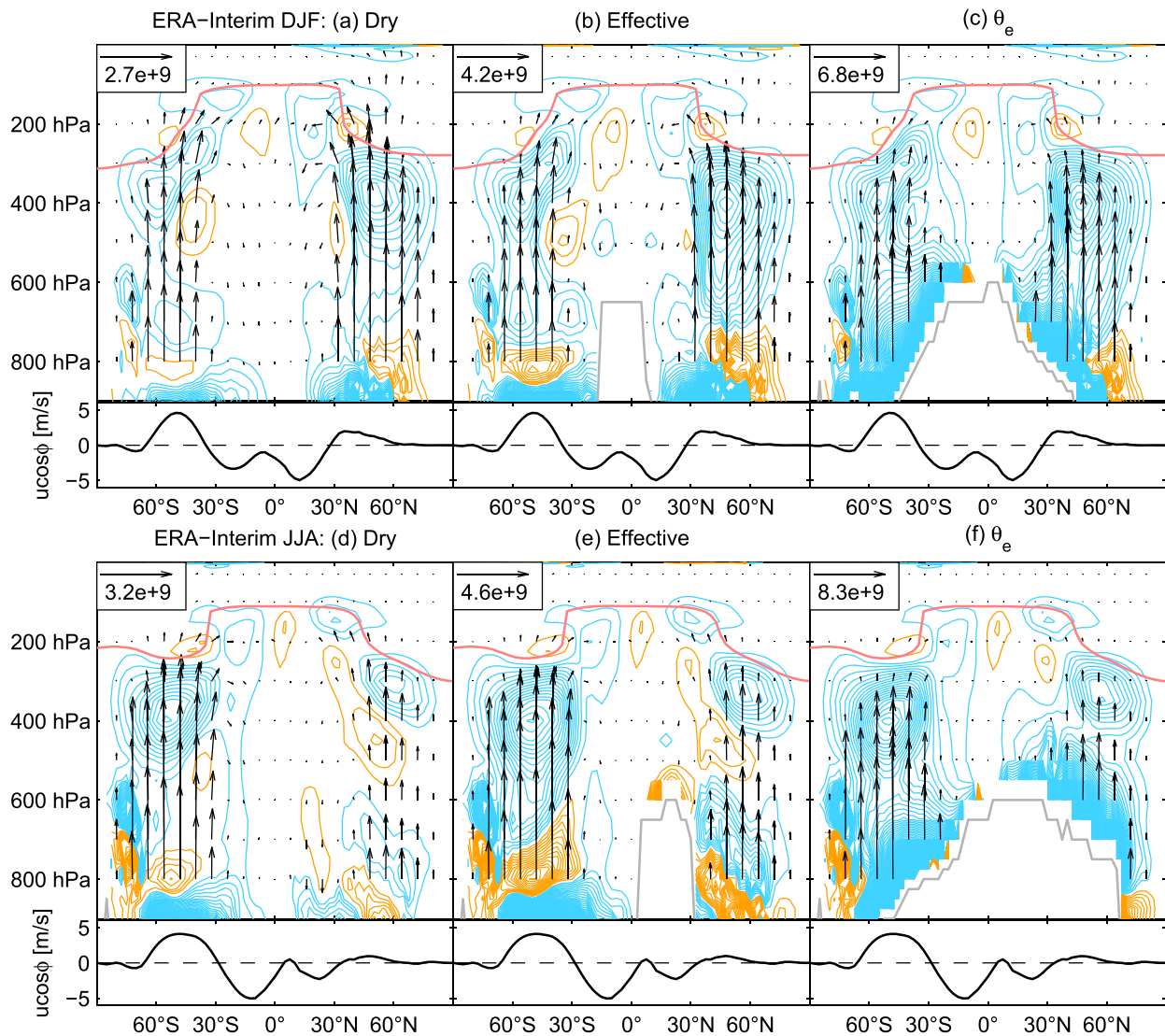
FIG. 1. The time-mean EP flux (arrows) and EP flux divergence (contours) for ERA-Interim from 1980–2013 in (top) DJF and (bottom) JJA, calculated (a),(d) with the dry theory; (b),(e) with the effective static stability; and (c),(f) with equivalent potential temperature. Contour intervals are 75 \text{ m}^2 \text{ s}^{-2} in all panels, with blue contours indicating convergence and orange contours divergence. The horizontal arrow scale varies between panels and is given in each panel ( \text{m}^3 \text{ s}^{-2} ). A vertical arrow of the same length has a flux equal to the horizontal arrow scale multiplied by 4.5 \times 10^{-3} \text{ Pa m}^{-1} . Data are not plotted below the level at which the appropriate static stability [ -\partial\theta/\partial p , -(\partial\theta/\partial p)_{\text{eff}} , or -\partial\theta_e/\partial p ] is smaller than 0.01 \text{ K hPa}^{-1} , as indicated by the gray line. The red line indicates the mean level of the tropopause using the WMO's lapse-rate definition, and the black line plot below each panel shows the zonal- and time-mean surface zonal wind as measured by u \cos\phi at 10 m above the surface.
