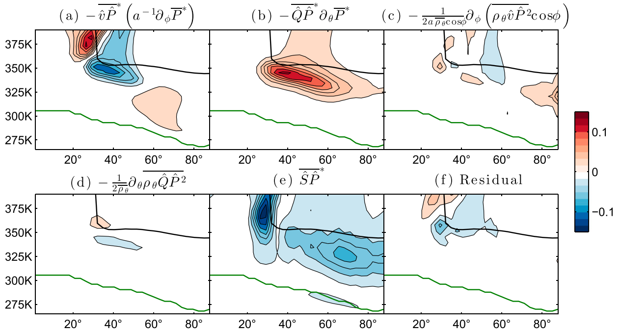
FIG. 7. The terms of the eddy enstrophy budget [Eq. (6)] for the idealized GCM with \alpha = 1.4 and \Delta_s = 1.2 in dry isentropic coordinates. All panels have contour intervals of 0.0167 \text{ PVU}^2 \text{ day}^{-1} . Shown are (a) the horizontal eddy PV flux term, (b) the cross-isentropic eddy PV flux term, (c) the horizontal eddy enstrophy flux convergence, (d) the vertical eddy enstrophy flux convergence, (e) the nonconservative term \hat{S}\hat{P}^* , and (f) the residual defined as the right- minus left-hand sides of Eq. (6). The black line denotes the WMO tropopause and the green line the median position of the surface. We do not plot values on levels that are below the surface 99% of the time or where \bar{\rho}_\theta < 10^{-6} \text{ kg K}^{-1} \text{ m}^{-2} .
