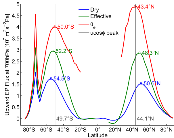
FIG. 2. The annual-mean upward EP flux at 700 hPa for ERA-Interim. The dry formulation is in blue, the effective moist formulation is in green, and the \theta_e moist formulation is in red. The gray vertical lines represent the latitude of peak surface u \cos \phi in each hemisphere. The green and red curves are only plotted where their respective static stability parameters, -(\partial\theta/\partial p)_{\text{eff}} and -\partial\theta_e/\partial p , are larger than 0.01 \text{ K hPa}^{-1} . The latitude of the peak upward EP flux is given in each hemisphere for each formulation. In the SH, the peak was calculated for latitudes equatorward of 70^\circ\text{S} to avoid the peak associated with Antarctic topography.
