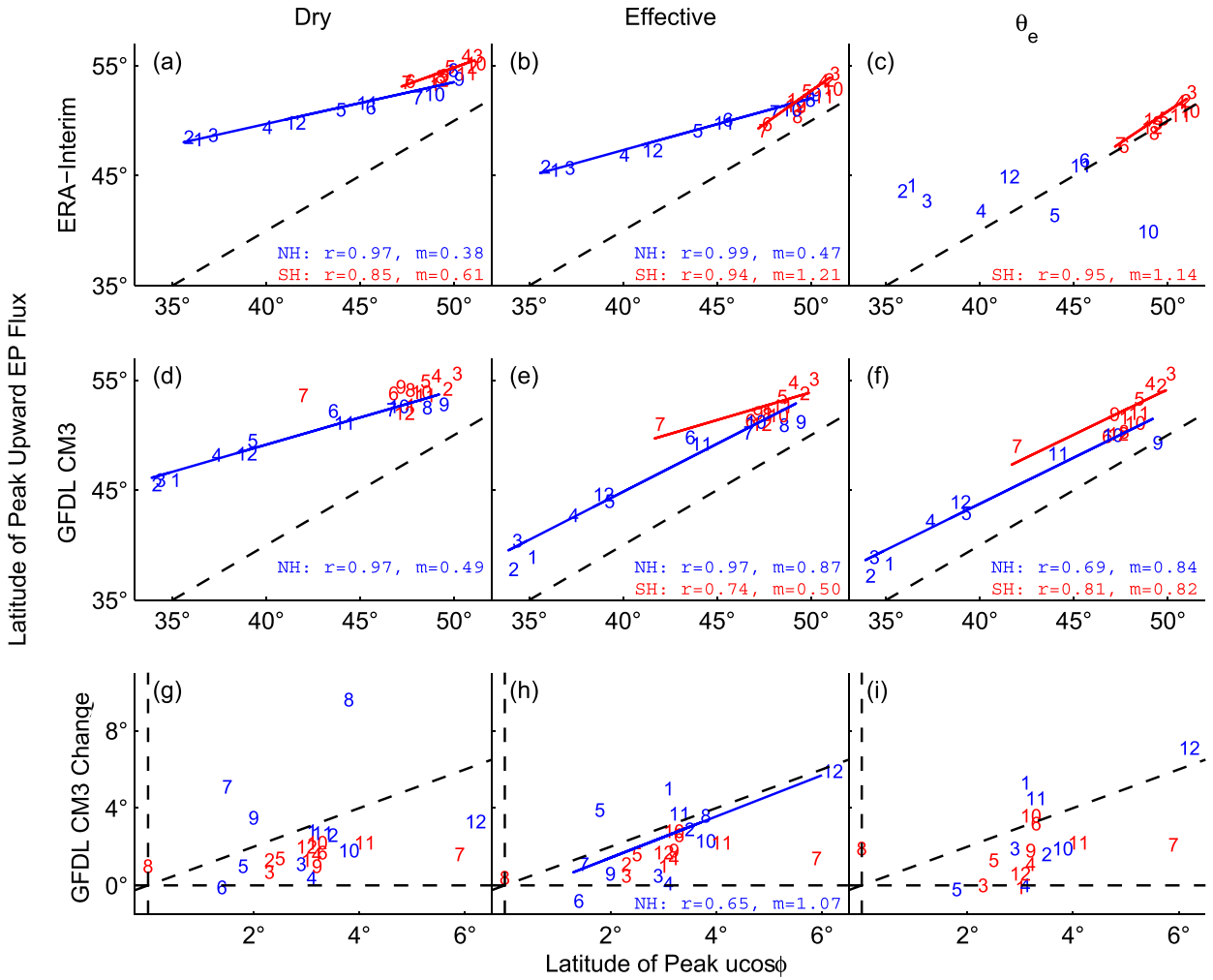
FIG. 4. Latitudes of peak upward EP flux at 700 hPa plotted against peak surface westerlies ( u\cos\phi ) for (a)–(c) ERA-Interim over 1980–2013; (d)–(f) GFDL CM3 over 1980–99; and (g)–(i) projected changes in GFDL CM3 under the RCP8.5 scenario. Latitudes are shown over the seasonal cycle in the NH (blue) and SH (red), and the EP fluxes are evaluated using (a),(d),(g) the dry; (b),(e),(h) effective; and (c),(f),(i) \theta_e formulations. Numbers represent the month (1 for January, 2 for February, etc.). Least squares regression lines are plotted, and the corresponding slopes m and correlation coefficients r are given in each panel, except where a null hypothesis of zero slope and independent monthly values cannot be rejected at the 5% level (a two-sided t test is used). In the \theta_e panels, the latitudes of peak upward EP flux for some months could not be found because of near-zero static stabilities. The dashed lines are the one-to-one and zero lines.
