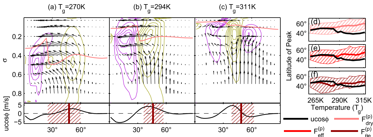
FIG. 9. (a)–(c) EP fluxes in the \theta_e formulation and contoured horizontal eddy momentum flux divergence (not EP flux divergence) for the idealized GCM with \Delta_s = 1.2 and T_g of (a) 270, (b) 294, and (c) 311 K. To emphasize horizontal wave propagation in the upper troposphere, the horizontal components of the EP flux vectors are first multiplied by a factor of 15, and then the magnitudes of the vectors are multiplied by -\log \sigma and then rescaled by a constant to have the same maximum length in each panel. Yellow contours indicate eddy momentum flux convergence and purple contours indicate eddy momentum flux divergence with contours every 75 \text{ m}^2 \text{ s}^{-2} . The black line plot below each panel shows the zonal- and time-mean surface zonal wind as measured by u\cos\phi at 10 m above the surface, and solid brown lines show the latitude of peak upward EP flux in the \theta_e formulation at \sigma = 0.67 , with hatching indicating the meridional range over which the upward EP flux is at least 70% of its peak value. (d)–(f) As in Fig. 6c, shown are the latitude of peak surface westerlies and peak upward EP flux at \sigma = 0.67 for \Delta_s = 1.2 in the (d) dry, (e) effective, and (f) \theta_e formulations, but also shown are the meridional range (hatching) over which the upward EP flux is at least 70% of its peak value.
