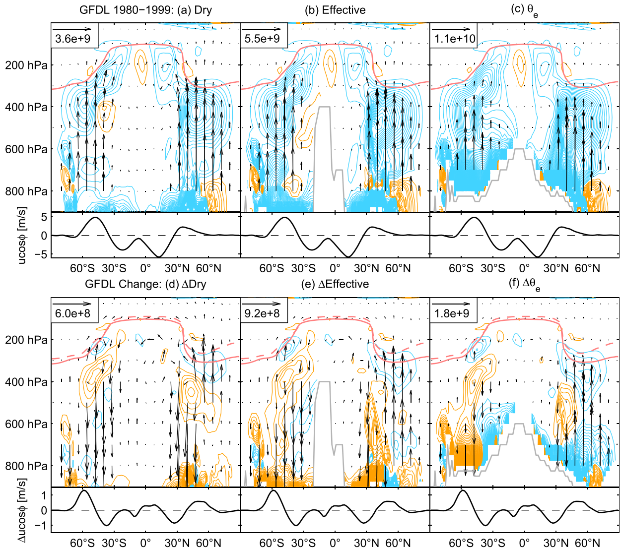
FIG. 3. As in Fig. 1, but for (top) the GFDL CM3 climatology over 1980–99 in DJF, and (bottom) the climate change for DJF defined as 2080–99 minus 1980–99 under the RCP8.5 scenario. In (bottom), the dashed red line shows the mean level of the tropopause for 2080–99.
