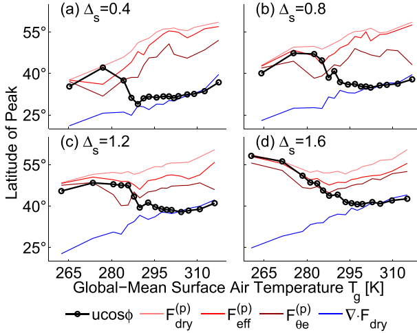
FIG. 6. Peak latitudes for various quantities as a function of global-mean surface air temperature T_g in the idealized GCM for different values of the meridional insolation gradient parameter \Delta_s . The surface westerlies are denoted by ucos\phi , F_{dry}^{(p)} is the dry upward EP flux, F_{eff}^{(p)} is the upward EP flux in the effective formulation, F_{\theta_e}^{(p)} is the upward EP flux in the \theta_e formulation, and \nabla \cdot F_{dry} is the anomalous region of dry EP flux divergence near the subtropical jet. The upward EP fluxes are evaluated at \sigma = 0.67 .
