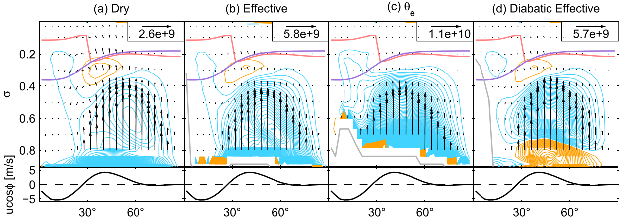
FIG. 5. As in Fig. 1, but for the idealized GCM with \alpha = 1.4 and \Delta_s = 1.2 (a relatively warm climate with a global-mean surface air temperature of 294 K). The EP flux formulations are (a) dry, (b) effective, (c) \theta_e , and (d) diabatic effective, an alternate version of the effective formulation described in the text in section 4. Vertical levels are in \sigma coordinates. The purple line shows the 350-K dry isentrope for reference.
