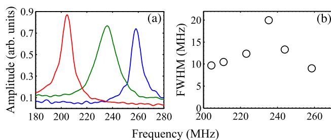
FIG. 4. (a) SAW Fourier peaks in the frequency range 200–270 MHz. (b) FWHM of Fourier peaks versus SAW frequency. Peak broadening indicates resonant absorption of SAWs centered at 235 MHz.
