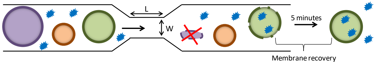
Fig. 1 Microfluidic Delivery Platform. Each microfluidic chip has 75 parallel channels, and each channel has a central constriction of 10 \mu\text{m} in length (labeled L above), and 4 to 9 \mu\text{m} in width (labeled W above). This illustration demonstrates the transit of cells through a single channel and its corresponding central constriction. As the cells pass through the constriction, there is temporary disruption of the cell membrane, and this allows for intracellular diffusion of materials (green cell). When a cell traverses a constriction whose width ( W ) is too narrow it results in cell death (purple cell). Conversely, when the constriction width is too large the mechanical deformation is insufficient to cause sufficient membrane disruption to enable delivery (brown cell).
