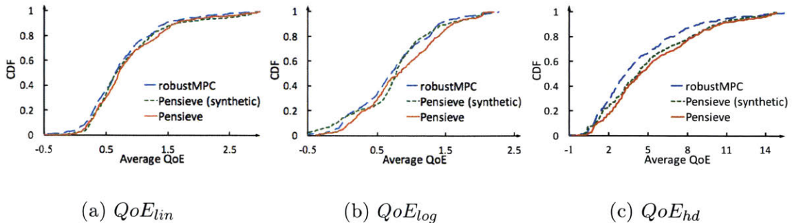
Figure 6-5: Comparing two ABR algorithms with Pensieve on the broadband and HSDPA networks: one algorithm was trained on synthetic network traces, while the other was trained using a set of traces directly from the broadband and HSDPA networks. Results are aggregated across the two datasets.
