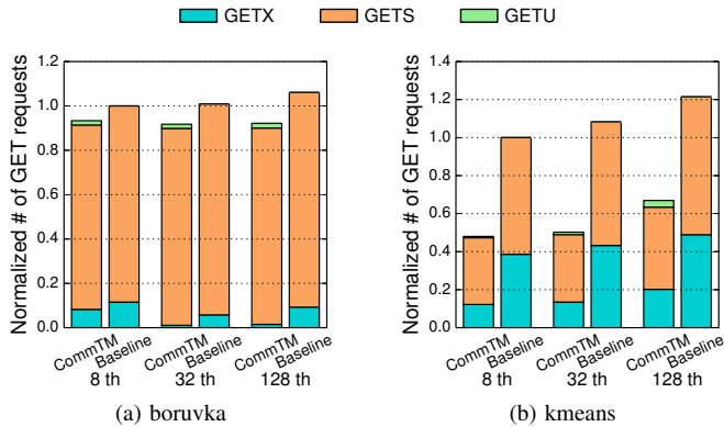
Fig. 19. Breakdown of total number of GET requests between L2s and L3 for COMMTM and conventional HTM on 8, 32 and 128 threads (lower is better).
