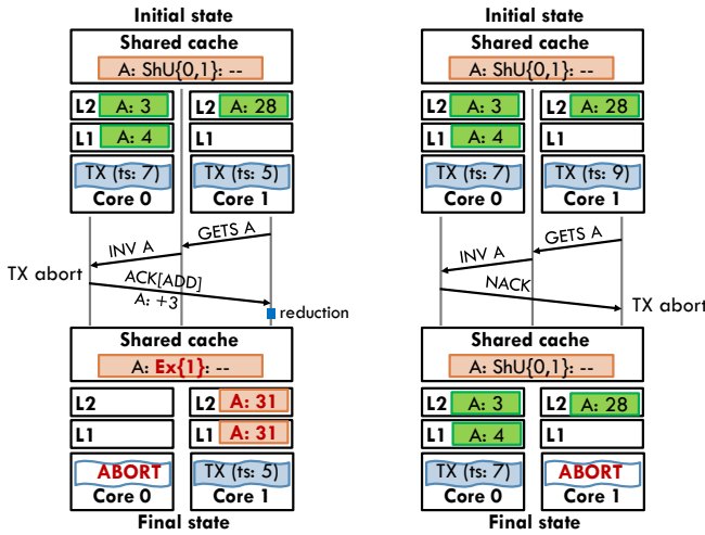
Fig. 6. Invalidation to lines in the labeled set cause a conflict. In this example, core 0 receives an invalidation request to a U-state line in its transaction’s labeled set: (a) if requester has a lower timestamp, abort and forward data; and (b) if requester has a higher timestamp, NACK invalidation.
