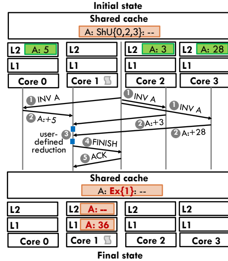
Fig. 7. Reductions are triggered by non-commutative requests. In this example, core 1 issues an unlabeled or differently-labeled request, causing a full reduction of line A’s U-state data, held in several private caches.
