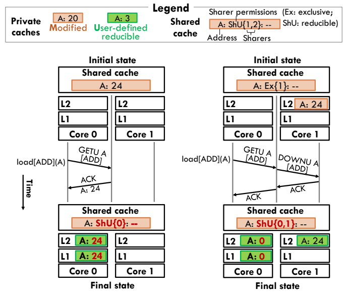
Fig. 4. Serving labeled memory accesses: (a) the first GETU requester obtains the data; and (b) another cache with the line in M is downgraded to U and retains the data, while the requester initializes the line with the identity value. Each diagram shows the initial and final states in the shared and private caches.
