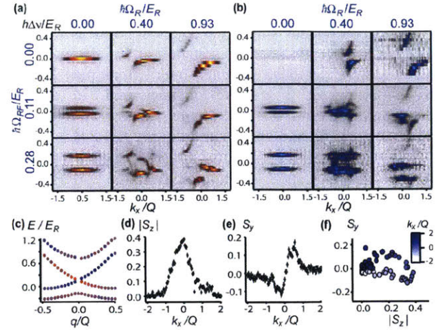
FIG. 4 (color online). Evolution of spin-textured energy bands of a spin-orbit coupled lattice. (a),(b) Experimental Raman-rf spin-injection spectra for injection from |\downarrow\rangle_R for channels |\downarrow\rangle and |\uparrow\rangle , respectively. The color map used is the same as Figs. 2(b) and 2(e) after rescaling to the maximum intensity. Interaction effects between |\uparrow\rangle with |\downarrow\rangle_R (see Fig. S4) makes only the dominant features resolvable in |\uparrow\rangle , while finer features are visible in |\downarrow\rangle . (c) Reconstructed band structure for \hbar\Omega_R = 0.93(7)E_R and \hbar\Omega_{\text{RF}} = 0.28(2)E_R . Color indicates the spin texture. (d)–(f) Experimentally measured spin components S_y and |S_z| as a function of momentum k_x for the lattice wave functions corresponding to the bottommost band in (c).
