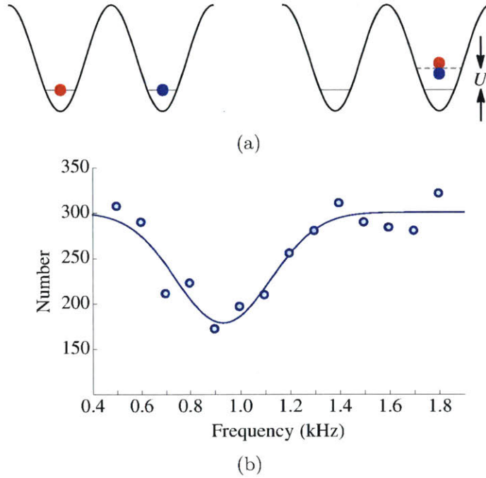
Figure 6-11: Calibrating U via lattice modulation. (a) In the atomic limit where U/t \gg 1 , the system is well-described by the occupation number of each lattice site. A double occupancy costs an additional energy of U . Therefore, in order for lattice modulation to drive a spin \sigma atom onto a neighboring site with a spin -\sigma atom, the modulation frequency must equal U/h . Note that the response is broadened by t/h , corresponding to the width of the upper Hubbard band. (b) A typical modulation spectrum. Here, \tilde{V}_0 = 10 and the scattering length is at the background value of a = 174a_0 [120].
