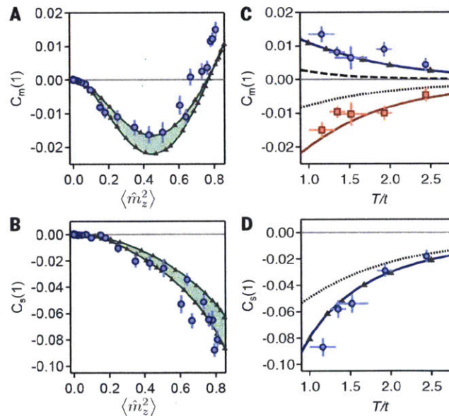
Fig. 2. Spin and moment correlators as functions of doping and temperature for U/t = 7.2(1) . (A and B) Nearest-neighbor moment correlator [ C_m(1) ] (A) and spin correlator [ C_s(1) ] (B) as functions of the local moment, denoted by blue circles. Results from NLCE (and DQMC) for temperatures T/t = 0.89 and 1.22 are shown in green lines (and gray triangles), with the intermediate temperature range indicated by green shading. (C) The maximum and minimum of the moment correlator as functions of temperature are denoted by blue circles and red squares, respectively. Corresponding results are obtained from NLCE (solid blue line and solid red line, respectively), for the noninteracting gas (black dashed and dotted lines, respectively), and from DQMC for the correlator at half-filling (gray triangles). (D) Nearest-neighbor spin correlator at half filling as a function of temperature (blue circles). Solid blue line, NLCE results; gray triangles, DQMC results; black dotted line, noninteracting gas. For all graphs, theory curves are not adjusted for the experimental imaging fidelity of 95%.
