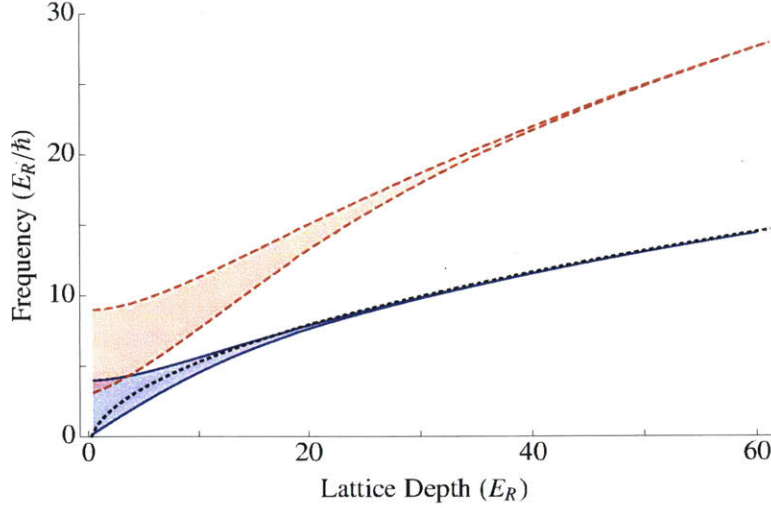
Figure 6-10: Band transition frequencies as a function of lattice depth. Shown in solid blue lines are the maximum and minimum transition frequencies versus lattice depth for transfer of atoms to the first excited band. In red dashed lines are the corresponding frequencies for transfer of atoms to the second excited band. Also shown, using the black dot-dashed line, is the harmonic approximation. The harmonic approximation \Delta E = \hbar\omega = 2E_R\sqrt{V_0} is corrected by the first order perturbation shift of -E_R . Note that for a Fermi gas, a large fraction of quasi-momentum states are occupied, which implies that the responses will cover the frequency range between the maximum and the minimum. It thus becomes difficult to calibrate the lattice at low depths. One can calibrate the lattice at higher depths where this is less of an issue, and subsequently scale the depth according to the lattice beam intensities. One also observes that although the transitions to the first excited band are suppressed at large depths, they have a smaller frequency spread. We therefore use these transitions for lattice calibration at intermediate depths.
