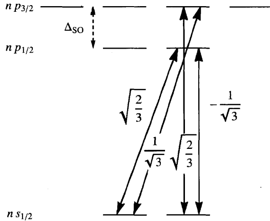
Figure 3-4: Raman coupling via p_{1/2} and p_{3/2} excited states. Shown are the Clebsch-Gordan coefficients for the relevant transitions that couple m_s = -1/2 \rightarrow m_s = 1/2 via \sigma_+ and \pi polarized light. As expected, the contributions to the two-photon transition amplitude from the p_{1/2} and p_{3/2} states are opposite and cancel at large single-photon detuning.
