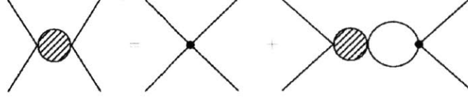
Figure 2-6: Graphical representation of the Lippmann-Schwinger equation. Here the dot denotes that interaction vertex -ig^{(\Lambda)} while the shaded circle represents the scattering amplitude i\mathcal{A}(E) . Figure reproduced from [16].
