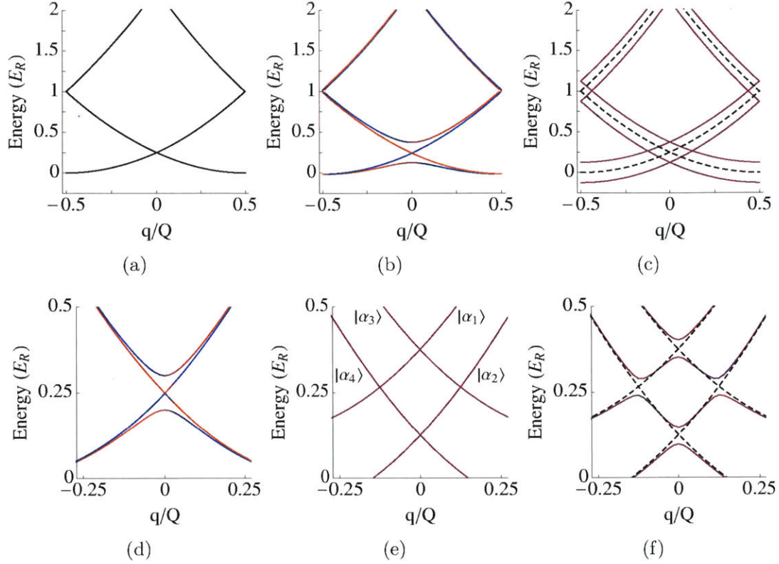
Figure 3-16: Band structure of Raman-RF lattice. The color indicates the spin composition \langle S_z \rangle , with blue and red corresponding to \langle S_z \rangle = 1 and \langle S_z \rangle = -1 respectively. (a) Band structure in the absence of Raman and RF coupling. We have chosen the spin-dependent gauge such that quasi-momentum q = 0 corresponds to real momentum of k = q + (n \pm 1)Q/2 for \uparrow and \downarrow atoms respectively. Each band is doubly degenerate with the two spin states. The point at E = 0.25E_R at q = 0 is quadruply degenerate. (b) Shown is the case with only Raman coupling, where \tilde{\Omega}_R = 0.10 . This is simply the reduced zone representation of the same Hamiltonian shown in Fig. 3-2. (c) Shown is the case with only RF coupling, where \tilde{\Omega}_{RF} = 0.25 . This splits the two degenerate bands for each spin shown in (a) by \hbar\Omega_{RF} . (d) Zoomed-in view of the initially quadruply degenerate point when \tilde{\Omega}_R = 0.1 . In this case, two of the bands are coupled, and the degeneracy is partially split. This is the only gap that opens up at all energies and all quasi-momentum, and corresponds to the two-photon resonance of the Raman beams. (e) Zoomed-in view of the case in (b), where only RF coupling is present, and \tilde{\Omega}_{RF} = 0.25 . The states labeled Eq. (3.39) are labeled. The quadruple degeneracy is lifted, and forms four pairs of degeneracies, two at q = 0 , and two at q = \pm\kappa . (f) When the Raman coupling is switched on, all the band crossings shown in (e) become avoided crossings. Shown in dashed is are the bands when \Omega_R = 0 . In general, the case of \tilde{\Omega}_R \neq 0 and \tilde{\Omega}_{RF} \neq 0 , all band crossings become gapped.
