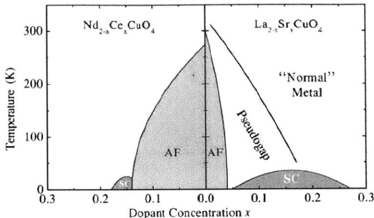
Figure 2-11: Schematic phase diagram of cuprates. Here, the dopant concentration of x corresponds to half-filling \langle \hat{n}_i \rangle = 1 . Note that unlike the phase diagrams for cuprates, the phase diagram for the Hubbard model with only nearest-neighbor tunneling is symmetric across half-filling. This symmetry is broken if a next-nearest-neighbor tunneling term is added. Figure reproduced from [28].
