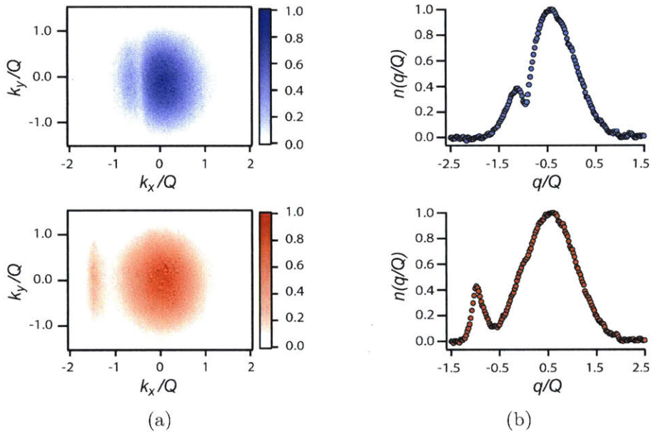
Figure 3-8: Spin and momentum-resolved images and profiles. (a) Spin and momentum-resolved images after a \pi -pulse is applied. The top (blue) and bottom (red) are the |\uparrow\rangle and |\downarrow\rangle channels respectively. Atoms in a momentum class satisfying the two-photon resonance condition are transferred from |\uparrow\rangle to |\downarrow\rangle while simultaneously receiving a momentum kick of -Q . (b) Corresponding integrated spin and momentum-resolved profiles as a function of quasi-momentum q/Q . Figures reproduced from [23].
