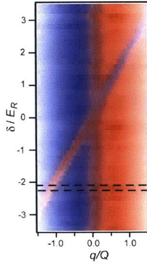
Figure 3-9: Raman transfer as a function of the two-photon detuning \delta . The Raman strength is \hbar\Omega_R = 0.035(5)E_R , and the pulse time corresponds to that of a \pi -pulse. Figures reproduced from [23].
