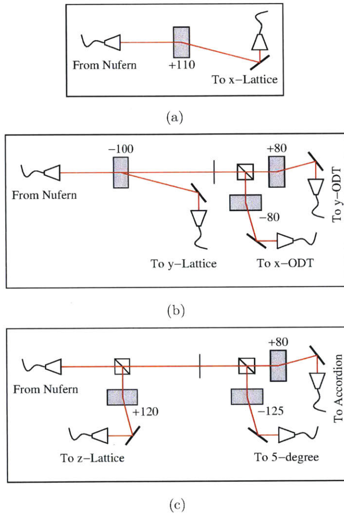
Figure B-9: 1064 nm laser system schematics.
