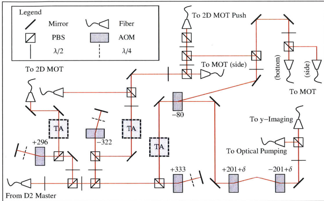
Figure B-1: Main laser table for ^{40}\text{K} D2 Light. The y -imaging light is combined with ^{23}\text{Na} D2 imaging light from the F = 2 (B) output with a dichroic mirror, before being sent to the experiment with a single fiber. Frequencies are in MHz.
