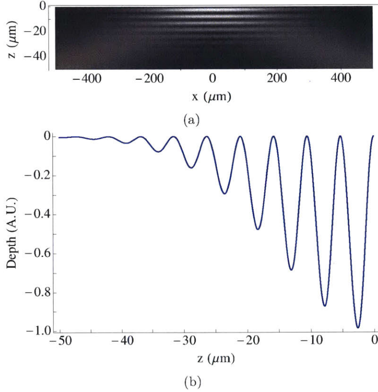
Figure 4-7: Trapping potential formed by the 5-degree beam. Shown is the case when the vertical waist of the beam is 35 \mu\text{m} . (a) Side view of the trapping potential formed by the 5-degree beam, viewed along \hat{y} . The reflection from the substrate interferes with the incoming beam to form a vertical lattice along \hat{z} . The trapping depth is indicated by the brightness. (b) A cut of the trapping potential along the z -axis.
