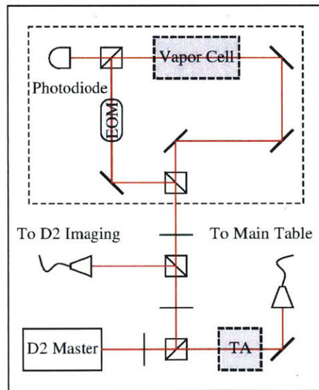
Figure B-2: Sub-system for ^{40}\text{K} master laser. The master laser is locked to the cross-over feature of the D2 line of ^{39}\text{K} via modulation transfer spectroscopy. Frequencies are in MHz.
