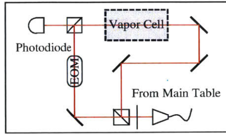
Figure B-5: Locking sub-system for ^{23}\text{Na} . The master laser is locked to the F = 2 \rightarrow F' = 3 feature of the D2 line of ^{23}\text{Na} via modulation transfer spectroscopy.
