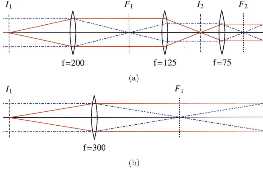
Figure 4-9: x and y crossed ODT beams. The atoms are at I_1 ; focal lengths are in units of mm. (a) x ODT beam path. The AOD is placed in the Fourier plane F_2 . This beam is combined with the accordion lattice beam at a polarizing beamsplitter placed near F_1 . (b) y ODT beam path. The AOD is placed in the Fourier plane F_1 . The beam is pre-shaped to be elliptical before reaching F_1 .
