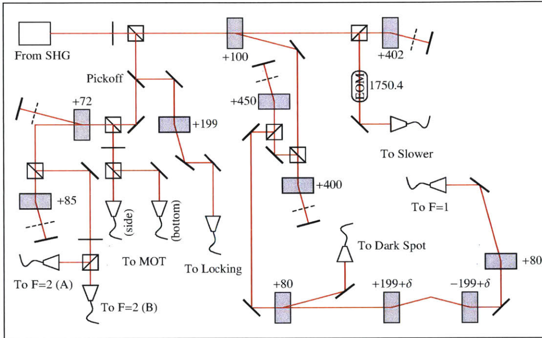
Figure B-4: Main laser table for ^{23}\text{Na} D2 light. Frequencies are in MHz. The F = 2 (A) is sent to the optical pumping axis along \hat{x} , while the F = 2 (B) is sent to both the y imaging axis, and a free-space multiplexer that combines with ^{40}\text{K} D2 imaging light. The outputs of the multiplexer are sent to the x and y bouncing imaging paths, and also to the vertical imaging path along \hat{z} . A single fiber brings the y -imaging light to the experiment.
