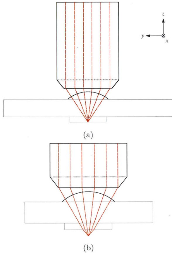
Figure 4-5: High-resolution imaging system. The high-resolution imaging system consists of a solid immersion lens that is integrated with the vacuum window, along with a high-NA (NA=0.6) EDMUND OPTICS 20X PLAN HR INFINITY CORRECTED OBJECTIVE. Specifically, the solid immersion lens, consisting of a 9 mm radius spherical cap, 5 mm thick fused silica vacuum window, and a 1.8 mm thick super-polished substrate, is shown. (a) Shown in dashed red lines are light rays originating from the surface of the super-polished substrate, at the center of the imaging axis. Light rays originating from the center propagate orthogonal to the air-glass interface of the solid immersion lens, thus avoiding imaging aberrations. (b) Shown is the case where the light still originates from a point on the imaging axis, but below the surface. For our experiments, the atoms are situated 7 \mu\text{m} below the surface. In addition to reducing aberrations, the solid immersion lens increases the effective NA. Since the atoms are displaced from the surface, the refraction at the vacuum-substrate interface increases the collection angle.
