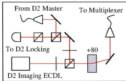
Figure B-3: Sub-system for D2 imaging laser. The D2 imaging laser is offset-locked to the D2 master laser. Frequencies are in MHz. The multiplexer combines ^{40}\text{K} D2 imaging light with ^{23}\text{Na} imaging light, and has outputs to the bouncing imaging and vertical imaging paths.
