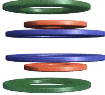
Figure 4-4: Coils used for generating magnetic fields. Shown is a view of the three relevant pairs of coils used. Shown in green are the MOT coils, which are displaced 12 mm along \hat{x} relative to the high-resolution imaging axis. Shown in red are the curvature coils, which are run in anti-Helmholtz configuration and used to generate a quadrupole field for the plugged quadrupole trap and for “slicing.” Concentric to the curvature coils are a pair of Feshbach coils, shown in blue, which are run in Helmholtz configuration and are used to generate a uniform bias field. In combination with the curvature coils, they can be used to move the center of the quadrupole trap.
