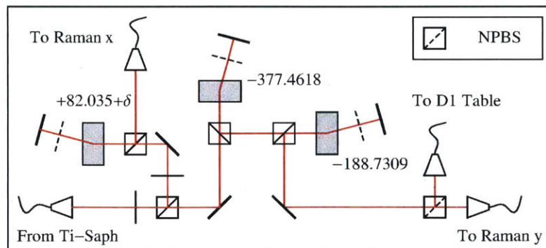
Figure B-8: Laser system for Raman light for ^{40}\text{K} . The light is detuned \sim 50 GHz to the red of the ^{40}\text{K} D2 line. \delta denotes the detuning from the carrier transition at the Raman imaging magnetic field of 4.2 G. Frequencies are in MHz.
