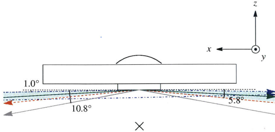
Figure 4-3: Side view along \hat{y} of the solid immersion lens and various beams. The intersection of the vertical center of the chamber and the high-resolution imaging axis is marked by the cross. The solid gray arrow indicates the direction of the “bouncing” imaging beam along \hat{x} , and also the direction of the incoming x lattice beam. The dashed red arrow indicates the direction of the 5-degree beam. The dot-dashed blue arrow indicates the direction of the x arm of the movable cross dipole trap. Two cases are shown: 1) when the beam is aligned to the center of the substrate; 2) when the beam is aligned to intersect the high-resolution imaging axis at 2 mm below the substrate. The green solid arrow indicates the direction of the accordion beam. The green shaded area indicates the range of angles ( \sim 1.0^\circ to \sim 5.0^\circ ) achievable with the accordion beam.
