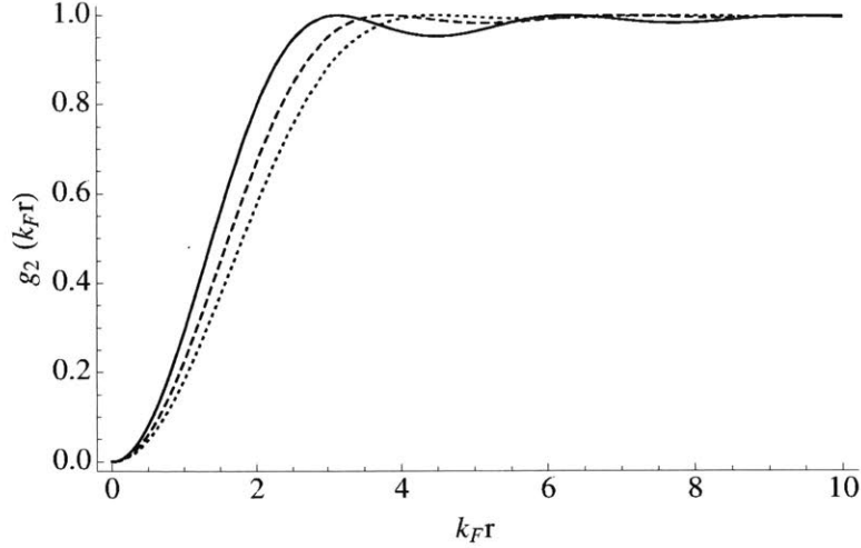
Figure 2-1: Friedel oscillations at T = 0 . The two-point density correlation function g_2(k_F r) for a 1D (solid), 2D (dashed), and 3D (dotted) Fermi gas at T = 0 . Friedel oscillations occur at spatial frequency of 2k_F . The Pauli exclusion principle results in g_2(k_F r) vanishing as r approaches 0, and consequently produces the “Pauli hole” at short separations.
