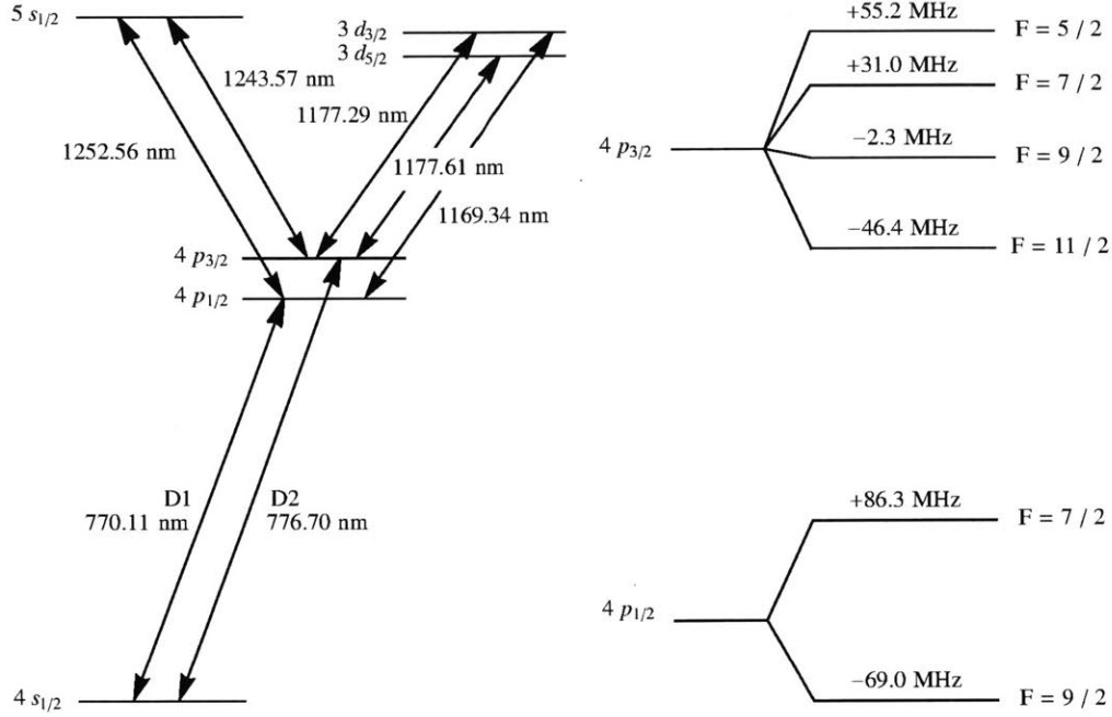
(a) Relevant levels and transition wavelengths for the 4p levels of ^{40}\text{K} . Values from [7]. (b) Hyperfine structure of 4p levels in ^{40}\text{K} .
