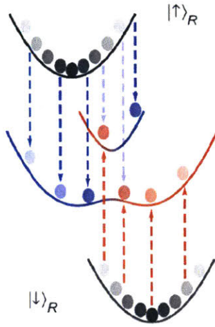
Figure 3-12: Spin-Injection Spectroscopy. The spin-orbit coupled system involves states |\uparrow\rangle and |\downarrow\rangle shown in blue and red respectively. In spin-injection spectroscopy, we make use of two reservoir states |\uparrow\rangle_R and |\downarrow\rangle_R , indicated by the gray parabolas shown above and below the spin-orbit coupled states. The reservoir states do not experience spin-orbit coupling. Their dispersion relation is that of free particles. Using RF pulses, selection rules allow for two transitions, |\uparrow\rangle_R \rightarrow |\uparrow\rangle and |\downarrow\rangle_R \rightarrow |\downarrow\rangle . Due to the long wavelength of RF radiation, the RF pulses do not impart any momentum. The two gray parabolas corresponding to the energy bands of the reservoir states are shifted in quasi-momentum by the spin-orbit momentum transfer Q . Figure reproduced from [23].
