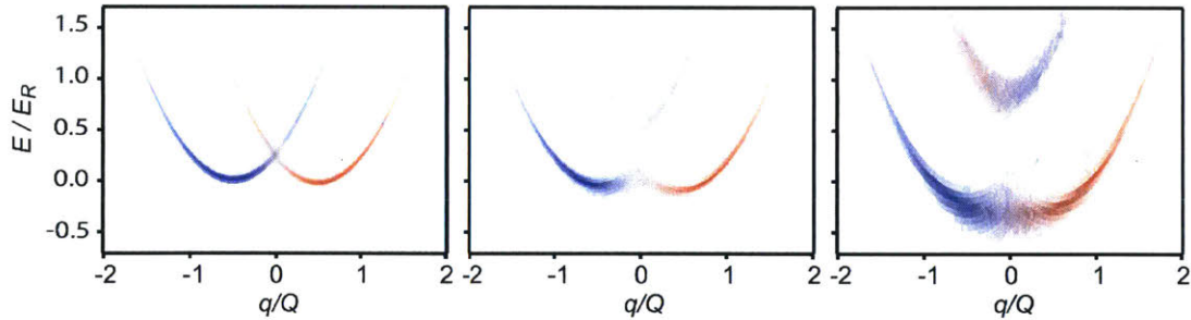
Figure 3-14: Spin-orbit bands reconstructed from spin-injection spectroscopy spectra. Shown from left to right are cases corresponding to \tilde{\Omega}_R = 0, 0.43(5) and 0.9(1) , respectively. The opening of the spin-orbit gap with increasing \tilde{\Omega}_R is seen. For the rightmost case, the merging of the two minima in the lower spin-orbit gap is evident. Figures reproduced from [23].
