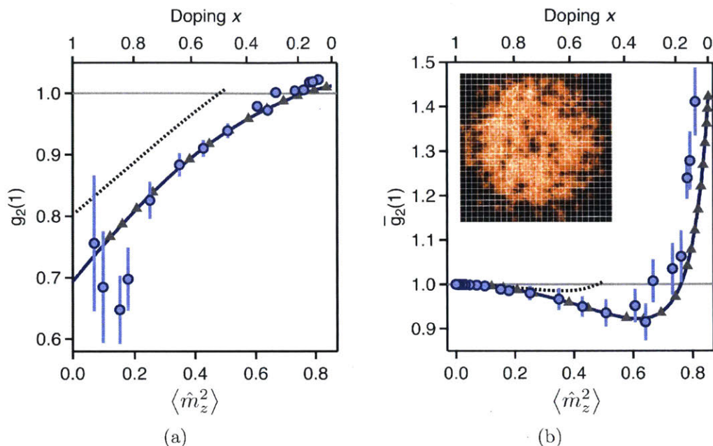
Figure 6-15: g_2(1) and \bar{g}_2(1) as a function of doping. (a) Shown is g_2(1) , the 2-point correlation function for moments at a separation of one lattice site, as a function of moment and filling. Shown in dashed is the result for the non-interacting Fermi gas as a function of filling. The suppression at low fillings can be interpreted as a direct observation of an interaction-enhanced Pauli hole. (b) Shown is \bar{g}_2(1) , the 2-point correlation function for anti-moments at a separation of one lattice site, as a function of moment and filling. \bar{g}_2(1) emphasizes the bunching property of anti-moments near half-filling. Shown in the inset is an exemplary image that shows pairs of neighboring anti-moments, which arise due to doublon-holon bunching near half-filling. Figures reproduced from [20].
