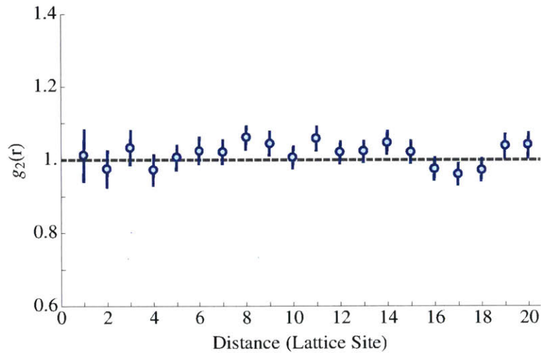
Figure 5-19: Bounding distance-dependent losses with g_2(r) . Shown in dashed is the uncorrelated value of g_2 = 1 . At low temperatures, one expects that g_2(r) < 1 at short distances, reflecting the Pauli exclusion principle. Correlation measurements showing this Pauli blocking effect is discussed in Chapter 6. Figure adapted from [22].
