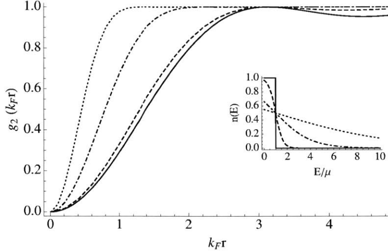
Figure 2-2: Friedel Oscillations in 1D at Finite Temperature. The two-point density correlation function g_2(k_F r) for 1/\beta\mu = 0 (solid), 1/\beta\mu = 0.3 (dashed), 1/\beta\mu = 1.5 (dot-dashed), and 1/\beta\mu = 5.0 (dotted) Fermi gas. At temperatures where \lambda_{dB} \sim 2\pi/k_F , Friedel oscillations are washed out, and the extent of the Pauli hole is now set by \lambda_{dB} .
