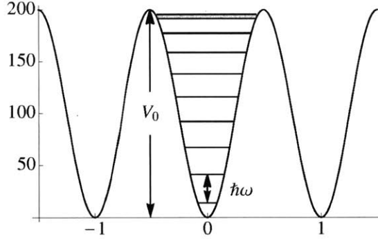
Figure 5-1: Energy levels in a deep lattice. In a deep lattice ( V_0 \gg E_R ), the spacing between the lowest and second lowest bands is approximately given by the \hbar\omega , where \omega = 2\sqrt{\tilde{V}_0}E_R/\hbar is the frequency of the harmonic oscillator that approximates the potential near the minimum of a single lattice well.
