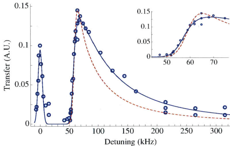
Figure 2-7: Dissociation Spectrum of Bound Molecules in 2D. The blue solid line indicates the fit to the lineshape taking into account logarithmic corrections from final state interactions, and finite frequency resolution of the experiment. The red dashed line shows a fit to the line shape without final state interactions. The peak on the left corresponds to response from free atoms. A convolution with a Gaussian response with width determined from the free atom peak is applied. The inset shows a zoomed-in view of the near-threshold response.
