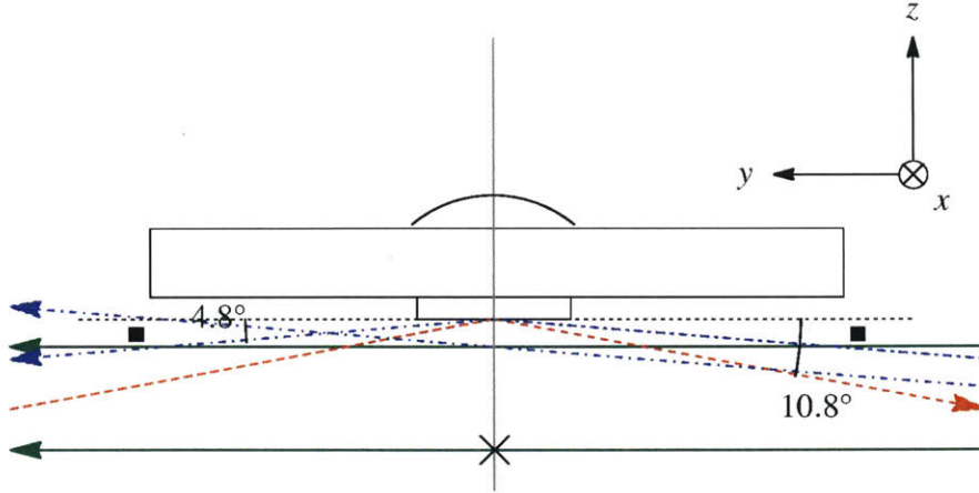
Figure 4-2: Side view along \hat{x} of various beams. The high-resolution imaging axis is shown in gray. The intersection of the vertical center of the chamber with the high-resolution imaging axis is marked by the cross, and is 9.5 mm below the substrate. The dashed red arrow indicates the direction of the “bouncing” imaging beam along -\hat{y} , and also the direction of the incoming y lattice beam. The dot-dashed blue arrow indicates the direction of the y arm of the movable cross dipole trap. Two cases are shown: 1) when it is aligned to the center of the substrate; 2) when it is aligned to intersect the high-resolution imaging axis 2 mm below the substrate. The black squares indicate the location of the in-vacuum RF antenna. The green solid arrows indicate the direction of the optical plug. The upper arrow corresponds to the case when the magnetic trap is \sim 2 mm below the substrate, while the lower arrow corresponds to the case when the magnetic trap is at the center of the chamber. The first scenario applies to Chapter 5, while the second applies to Chapter 6.
