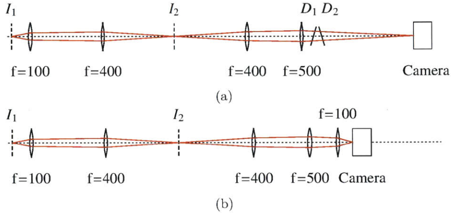
Figure 4-10: Vertical imaging paths z_1 and z_2 . The atoms are at I_1 ; a secondary imaging plane I_2 is formed 400 mm from the second lens, away from I_1 . Focal lengths are in units of mm. (a) Path z_1 . This path is used for single site imaging. The first lens on the right represents the combined objective and solid immersion lens system. The distances between the subsequent lenses are 620 mm, 800 mm and 300 mm. The distance from the last lens to the camera is 604 mm. These parameters are optimized for the smallest spot size through simulations with OSLO. Two SEMROCK LL01-780-25 dichroic filters are placed at positions D_1 and D_2 , 50 mm from the last lens. They are angled-tuned to pass 770 nm light resonant with the D1 transition of ^{40}\text{K} , and have a bandwidth of 3 nm. They are angled at opposite angles to minimize aberrations. The dimple beam, which has wavelength \sim 830 nm, is sent into the objective with the dichroic at D_1 . The dichroic at D_1 also allows absorption imaging on the D2 line of ^{40}\text{K} (path z_2 ). (b) Path z_2 . This path is used for absorption imaging, and is used for alignment of the 5-degree beam and all three lattice beams. This path is split from z_1 at dichroic D_1 , and has effective magnification of \sim 51 .
