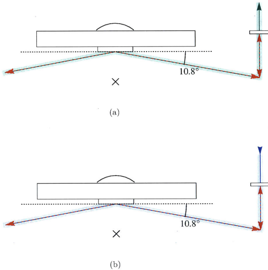
Figure 4-6: Side view of lattice, imaging and Raman cooling beams. (a) Side view of the lattice beams and the bouncing imaging beams along \hat{x} or -\hat{y} . The lattice beam path is indicated by the dashed red arrow. The “bouncing” imaging beam, indicated by the thick green arrow is transmitted through the retro mirror. (b) Side view of lattice and Raman cooling beams. For the case where one is looking down \hat{x} , the thick blue arrow indicates the path of the Raman beam along \hat{y} . The dashed red arrow indicates the path of the y lattice. For the case of looking down -\hat{y} , the thick blue arrow indicates the path of the Raman beam along -\hat{x} , and also the optical pumping beam used for Raman imaging. The Raman beams and the optical pumping beam are partially transmitted through the lattice retro-reflection mirror.
