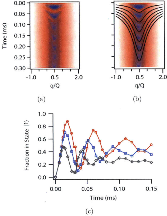
Figure 3-10: Momentum-dependent Rabi oscillations at \hbar\Omega_R = 0.78(2)E_R and detuning \delta = 0.25(1)E_R . (a) Spin and momentum-resolved profiles as a function of time after spin-orbit coupling is turned on suddenly. Here, \hbar\Omega_R = 0.71(2)E_R and \hbar\delta = -0.25(1)E_R . (b) Profiles with contours indicating minima of |\downarrow\rangle . (c) In circles, squares and diamonds are the |\uparrow\rangle fraction of as a function of time for \tilde{q} = 0.5, 0.25 , and 0.05 respectively. Figures reproduced from [23].
