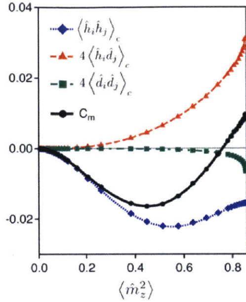
Figure 6-16: Various contributions to the nearest-neighbor moment-moment correlator C_m(1) . As expected, the holon-holon correlator \langle \hat{h}_i \hat{h}_j \rangle_c and the doublon-doublon correlator \langle \hat{d}_i \hat{d}_j \rangle_c are both negative, due to Pauli blocking and repulsive interactions. However, the doublon-holon correlator \langle \hat{h}_i \hat{d}_j \rangle_c is positive due to super-exchange. Figure reproduced from [20].
