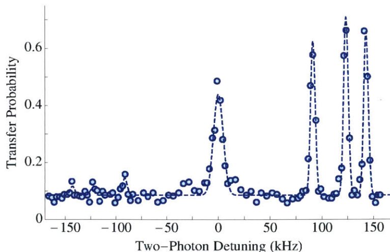
Figure 5-20: Sideband spectra after cooling. The sideband asymmetry indicates a ground state population in |9/2, -9/2\rangle of 72(3)%, even after imaging. Figure adapted from [22].
