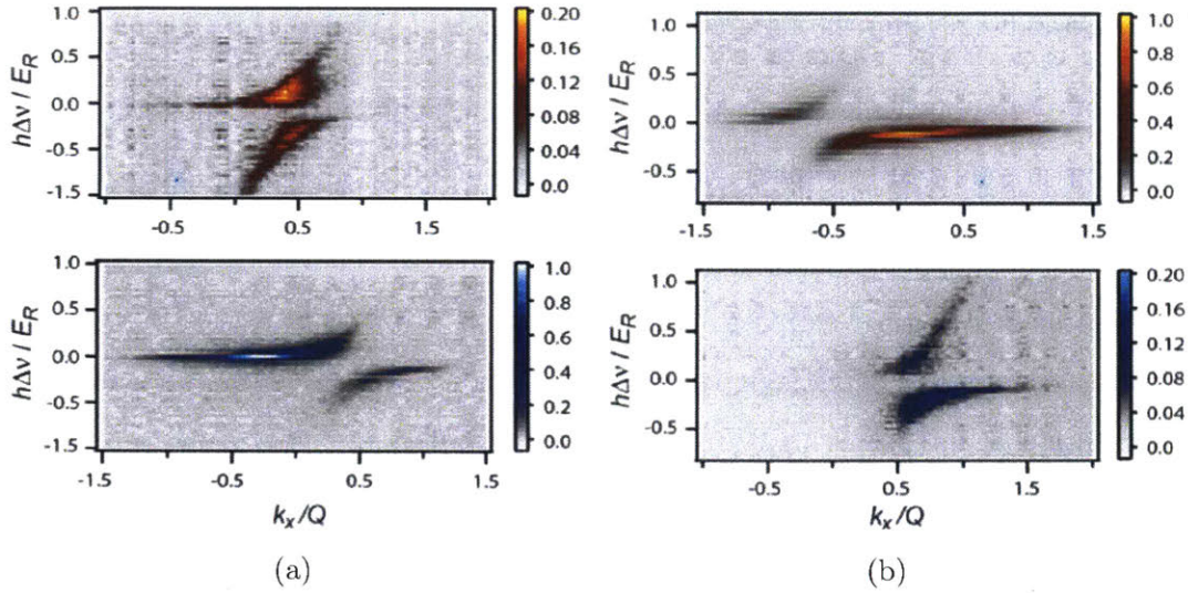
Figure 3-13: Bare spectra from spin-injection spectroscopy of spin-orbit coupled fermions. Here, \Delta\nu is the detuning in the RF frequency from the bare transition. (a) Shown are the spectra in the two channels |\downarrow\rangle (top) and |\uparrow\rangle (bottom), with atoms prepared in reservoir state |\uparrow\rangle_R . (b) Same as (a), except atoms are initially prepared in |\downarrow\rangle_R . Figures reproduced from [23].
