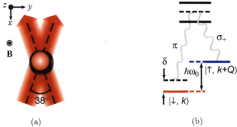
Figure 3-7: Raman beam geometry and polarizations. (a) Geometry of the two Raman Beams. (b) Schematic Diagram showing transitions and levels for Raman coupling. Figures reproduced from [23].
