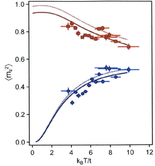
FIG. 4. Local moment \langle m_z^2 \rangle as a function of temperature at U/8\bar{t} = 2.6(1) for \mu/U = 0.5 (red squares) and \mu/U = -0.25 (blue circles). The local moments are extracted from 117 samples. For each sample, the temperature and global chemical potential are determined by fitting to HTSE in the outer regions where n_{\text{det}} < 0.25 . NLCE data at U/t = 21 with and without adjustment for imaging fidelity are shown in solid and dotted lines, respectively.
