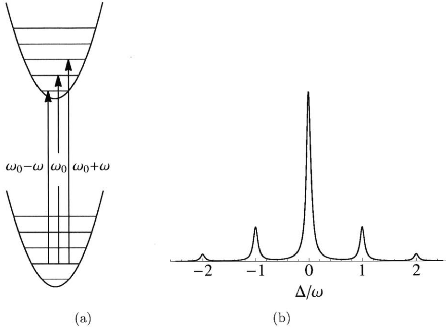
Figure 5-4: The sideband-resolved regime. (a) The vibrational changing transitions are spaced from the carrier frequency \omega_0 by the trap frequency \omega . Shown are the transitions that change the vibrational number by -1, 0 and 1 respectively. (b) Fluorescence as a function of transition frequency detuning \Delta from the carrier \omega_0 , normalized to the trap frequency \omega . When \Gamma \ll \omega , the sidebands can be resolved. Shown is the case where \Gamma = 0.1\omega , with Lamb-Dicke parameter of 0.2, for an atom in vibrational level \gg 1 .
