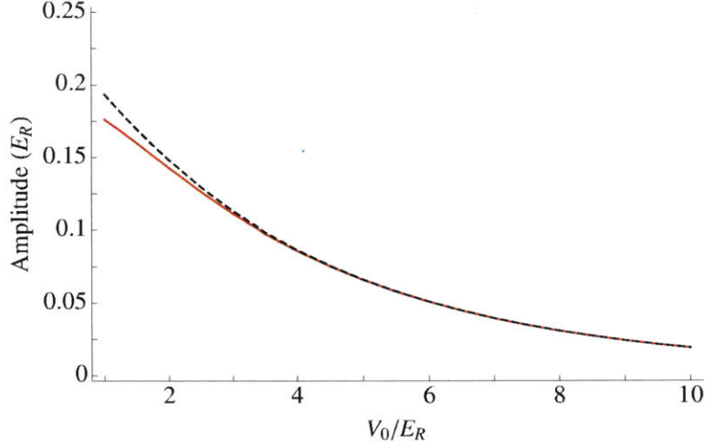
Figure 2-4: Nearest-neighbor hopping amplitude comparison. Shown in red solid line is the nearest-neighbor hopping amplitude t computed from Eq. (2.21); in black dashed line is t determined from the bandwidth of the lowest band.
