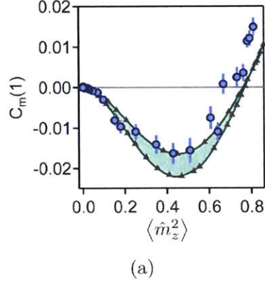
Figure 6-14: Nearest-neighbor moment correlator C_m(1) as a function of moment \langle \hat{m}_{z,i}^2 \rangle at U/t = 7.2 . For comparison, NLCE results are shown by the green lines while DQMC results are shown by the gray triangles, for two temperatures k_B T/t = 0.89 and 1.22. A sign change is observed around \langle \hat{m}_{z,i}^2 \rangle = 0.7 . Figure from [20].
