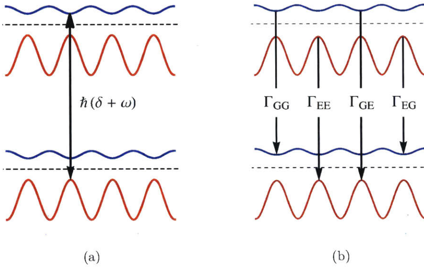
Figure 5-7: Dressed States at Non-Zero Detuning. (a) At \Omega = 0 , the dressed states |G, N\rangle and |E, N\rangle are now split by an additional \pm\hbar\delta/2 . (b) Even when \Omega \neq 0 , the admixture of |e\rangle ( |g\rangle ) into |G, N\rangle ( |E, N\rangle ) can be small. Shown here is the case for \Omega/\delta = 2/3 . The color indicates the admixture of |g\rangle (blue) and |e\rangle (red). When \Omega \neq 0 , four decay channels are possible. These are labeled and indicated by the arrows.
