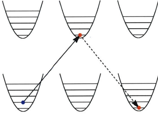
Figure 5-5: Sideband Cooling. An atom starts in |g, 1\rangle . Light resonant on the \omega_0 - \omega cooling sideband excites the atom to |e, 0\rangle . The atom subsequently decays into |g, 0\rangle preferentially, and its vibrational number remains unchanged. Overall, the energy decreases by \hbar\omega .
