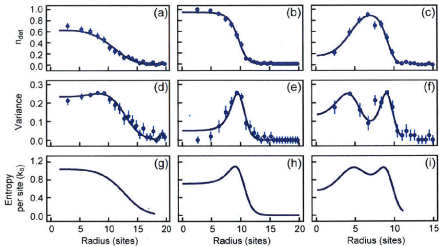
FIG. 2. Radially averaged detected site occupation [(a)–(c)], variance [(d)–(f)], and entropy [(g)–(i)], with theoretical curves. [(a), (d), and (g)] Metallic state, with \mu_0/h = 280 (40) Hz and k_B T/U = 1.46 (18); average entropy per particle S/N = 1.7 (1) k_B . [(b), (e), and (h)] Mott-insulating central region, with \mu_0/h = 624 (22) Hz and k_B T/U = 0.09 (1); S/N = 1.23 (6) k_B . [(c), (f), and (i)] Band-insulating center and Mott-insulating annular region, with \mu_0/h = 1450 (40) Hz and k_B T/U = 0.18 (2); S/N = 0.99 (6) k_B . The profiles were fitted to numerical linked cluster expansion (NLCE) data with U/\bar{t} = 3 for (a), (d), and (g) and to high-temperature series expansion (HTSE) for (b), (e), and (h). For (c), (f), and (i), profiles were fitted to NLCE data with U/\bar{t} = 21 , shown in solid.
