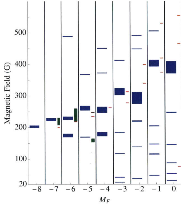
Figure C-1: Some Feshbach resonances of ^{40}\text{K} . The positions and widths of Feshbach resonances for M_F \leq 0 . The lowest channel l = 0, 1 resonances are shown in blue and dark red, respectively; the second lowest channel l = 1 resonances for M_F \leq -4 are shown in green. The l = 1 resonance widths are for a collision energy of 1 \mu\text{K} above threshold. Widths less than 0.1 \text{ G} are shown as 0.1 \text{ G} .
