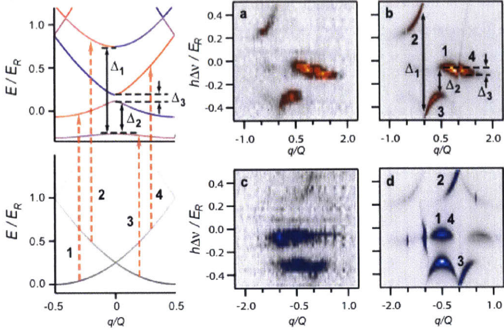
Figure 3-17: Spin-injection spectroscopy on a Raman-RF lattice. Shown on the left are the Raman-RF bandstructure (top), and the bandstructure (bottom) of the reservoir states. The experimental bare spectra corresponding to starting in reservoir state |\downarrow\rangle_R is shown in panels (a) and (c) on the right. The corresponding theoretical spectra is shown in panels (b) and (d). The transitions 1 to 4, and gaps \Delta_1 , \Delta_2 and \Delta_3 are identified on the theoretical spectra. By selecting certain features, the dispersions and spin compositions of various bands can be reconstructed.
