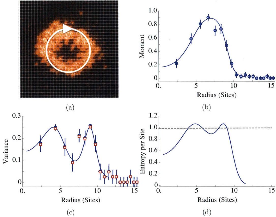
Figure 6-12: Radially averaged profile of a sample with coexisting metallic, Mott insulating and band-insulating regions. The Hubbard parameters are U/8t = 2.6(1) . (a) The bare image overlaid with the underlying lattice; a radial averaging contour is shown schematically. (b) The radially averaged local moment versus radius. Shown in the solid blue line is a fit of to profile to NLCE data. The fit yields a global chemical potential of \mu_0 \approx 1.4U and a temperature of k_B T/t = 3.7 . (c) Variance of the local moment. Shown in blue circles is the experimentally measured variance, which assumes that sites at equal radii are equivalent. Shown in red squares is the variance computed from the average moment. The error bars for the second method are not shown. (d) Entropy per site as a function of radius, obtained from NLCE theory using the fitted parameters. The average entropy per particle, 0.99(6) k_B , is shown by the dashed black line.
