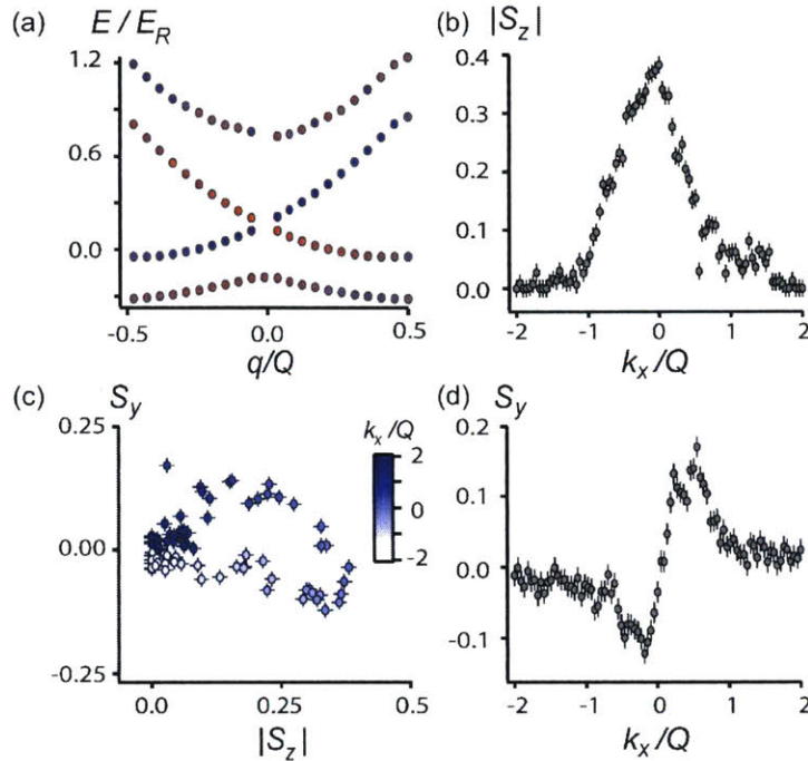
Figure 3-18: Extracting spin composition for the Raman-RF Lattice, with \tilde{\Omega}_R = 0.93 and \tilde{\Omega}_{RF} = 0.28 . (a) Reconstructed spin composition and dispersion for the lowest four bands, for \tilde{\Omega}_R and \tilde{\Omega}_{RF} . (b,d) Extracted spin composition of the lowest band in the basis of free space momentum states labeled by k_x . Here, a spin-dependent gauge is applied such that the k_x is shifted from the laboratory frame momentum by \pm Q/2 , for \uparrow and \downarrow atoms respectively. (c) The extracted spin as a function of momentum k_x . Figures reproduced from [23].
