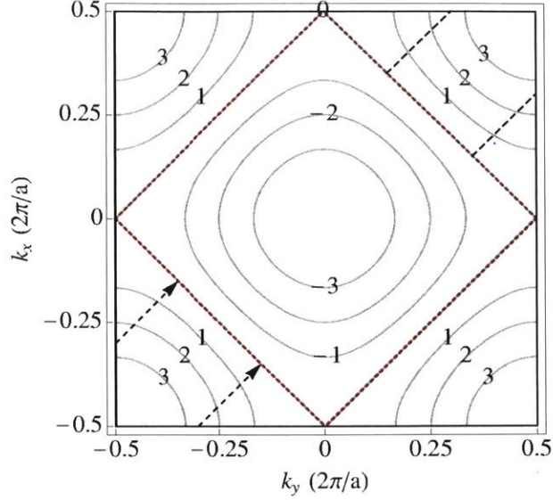
Figure 2-10: Nesting on the half-filled square lattice. Solid lines mark the Fermi surfaces for difference energies. The energy contours are marked in units of the tunneling amplitude t . The red dotted lines indicates the Fermi surface ( E = 0 ) for the half-filled square lattice. The nesting wavevector (1, 1) shown by the dashed arrows connect two edges of the Fermi sea.
