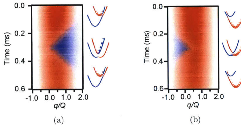
Figure 3-11: Adiabatic loading of spin-orbit bands at \hbar\Omega_R = 0.53(5)E_R . (a) Starting with detuning \delta = -8.5\Omega_R , \delta is swept linearly at a rate of |\dot{\delta}| = 0.27(5)\Omega_R^2 to \delta = 0 , and swept back. The atoms remain in the upper spin-orbit band at all times. A diagram indicating the population along in the spin-orbit bands is shown on the right. (b) Starting with detuning \Delta = 8.5\Omega_R , \delta is swept linearly at a rate of |\dot{\delta}| = 0.27(5)\Omega_R^2 towards \delta = 0 , and swept back. The atoms are loaded into the lower spin-orbit band. A diagram indicating the population along in the spin-orbit bands is shown on the right. Figures reproduced from [23].
