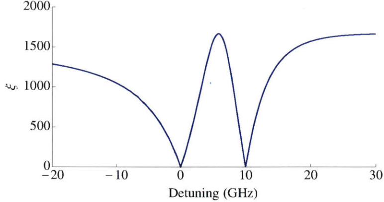
Figure 3-5: Figure-of-merit \xi of Raman coupling in {}^6\text{Li} ignoring hyperfine structure. Shown is \xi as a function of red detuning \Delta from the p_{3/2} level. The optimal ratio \xi is obtained 4.0 GHz to the blue of the D1 line.
