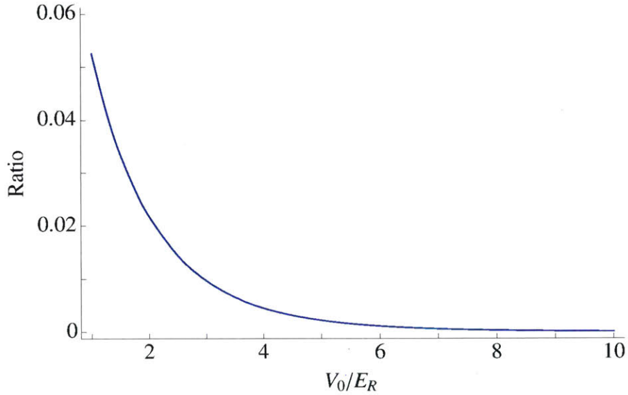
Figure 2-8: Ratio of on-site interaction to nearest-neighbor interaction U_0/U_1 .
