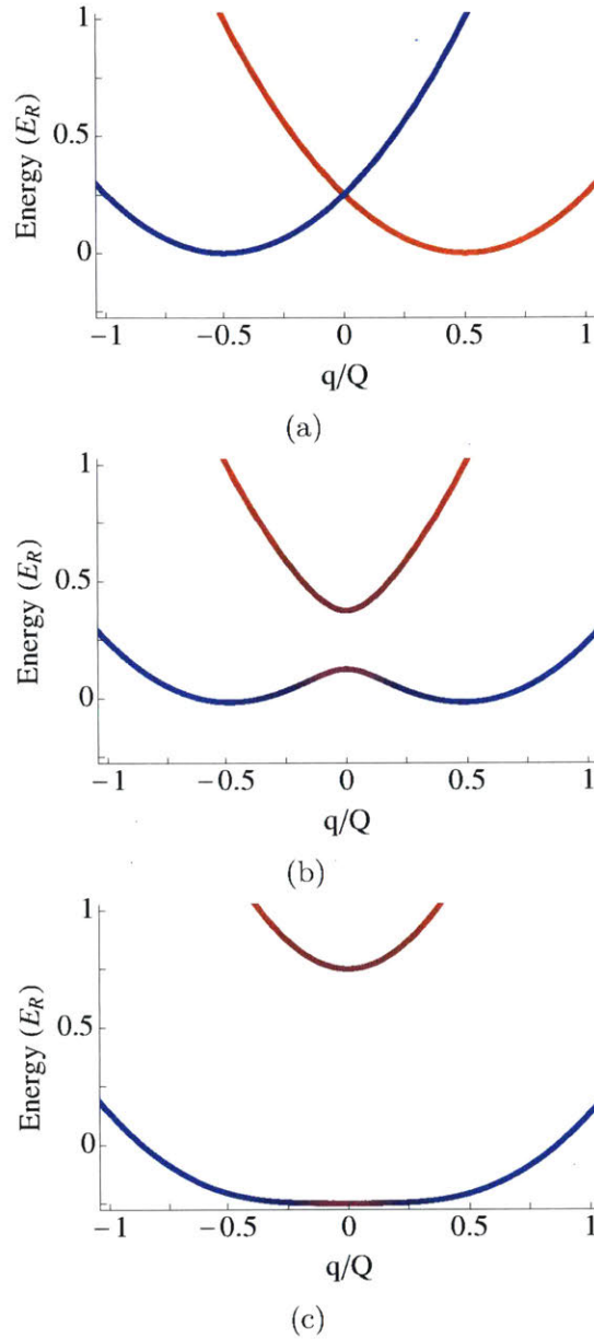
Figure 3-2: Spin-orbit bands. Here, the color denotes the spin composition, with blue (red) indicating |\uparrow\rangle ( |\downarrow\rangle ). (a) With only the spin-orbit coupling term, we obtain two free particle dispersions shifted by momentum Q = E_R/\lambda_{SO} , with E_R = \hbar^2 Q^2/(2m) . (b) In the presence of a transverse Zeeman field of amplitude \hbar\Omega/2 , the crossing at Q = 0 becomes an avoided crossing. A spin-orbit gap emerges with size \hbar\Omega_R . (c) When \hbar\Omega_R = E_R , the bottom band changes from having two minima at Q \neq 0 to having a single minimum at Q = 0 .
