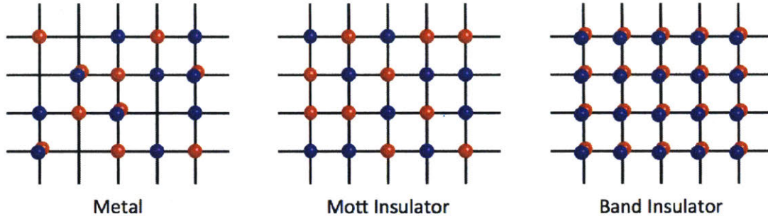
Figure 2-9: States of the Fermi-Hubbard Model. Shown are the real space pictures of the metallic state, the Mott-insulating state, and the band-insulating state.
