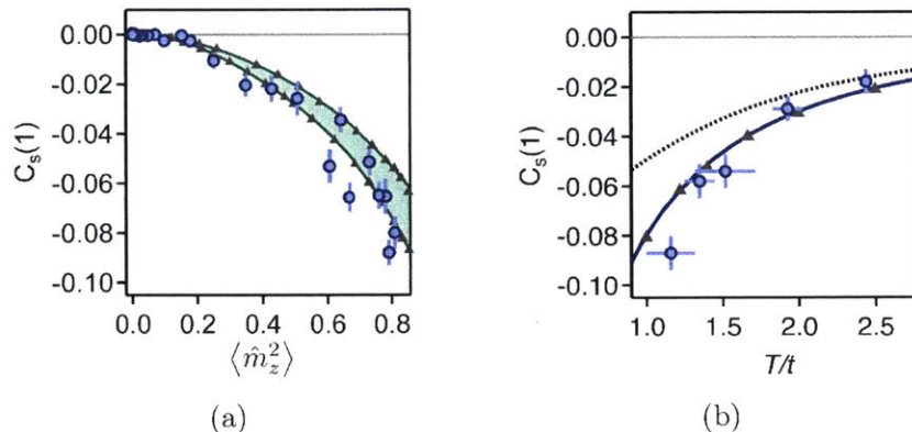
Figure 6-13: Nearest-neighbor spin correlator C_s(1) . (a) C_s(1) as a function of the moment \langle \hat{m}_{z,i}^2 \rangle at U/t = 7.2 . For comparison, NLCE results are shown by the green lines while DQMC results are shown by the gray triangles, for two temperatures k_B T/t = 0.89 and 1.22 . (b) C_s(1) as a function of temperature k_B T/t . The results for the non-interacting gas is shown by the gray dotted line. The solid blue line shows NLCE results, while the gray triangles show DQMC results. Figures reproduced from [20].
