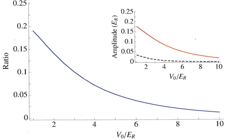
Figure 2-3: Ratio of nearest neighbor hopping amplitude to next-nearest neighbor hopping amplitude, |t'/t| , as computed from Eq. (2.21). The inset shows |t| and |t'| in dashed black and solid red lines respectively.
