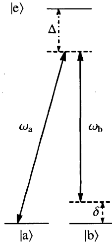
Figure 3-3: Raman coupling two ground states with two photons via an intermediate excited state.
