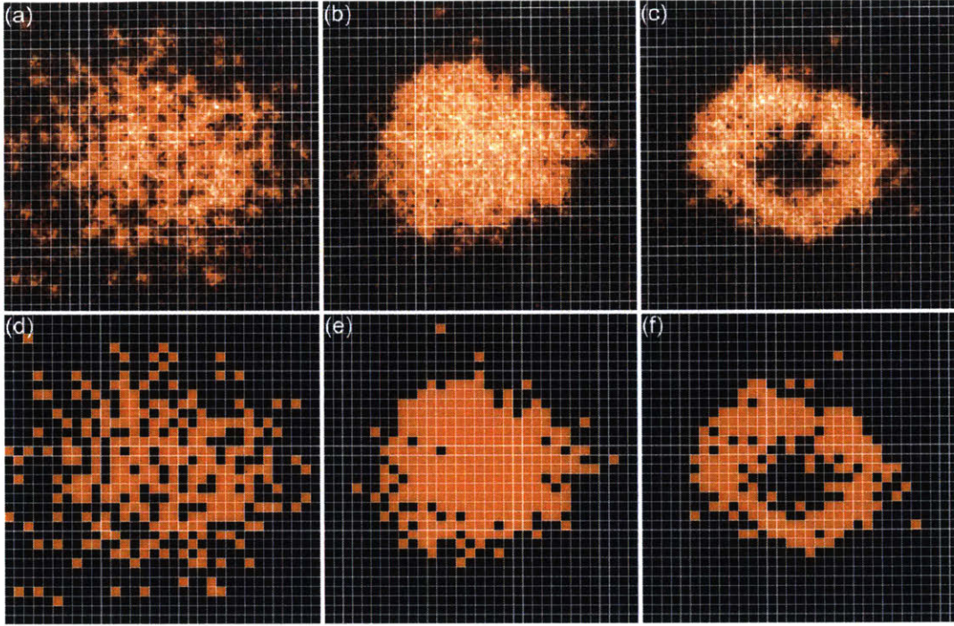
Figure 6-9: Site-resolved images of metals and insulators. Shown in (a), (b) and (c) are site-resolved images of ^{40}\text{K} atoms trapped in a 2D square lattice. (d), (e) and (f) are the corresponding reconstructed site occupations. In (a,d), U/8t = 0.33 , \mu_0/U = 0.52 , and k_B T/U = 1.46 . A metallic state is observed. In (b,e), U/8t = 12.3 , \mu_0/U = 0.46 , and k_B T/U = 0.09 . A Mott insulator is observed. In (c,f), U/8t = 2.6 , \mu_0/U = 1.43 , and k_B T/U = 0.18 . A band insulating region is observed in the center of the trap. Here, \mu_0 denotes the chemical potential in the center of the trap. Temperatures and chemical potentials are obtained from fits of the radially averaged profiles to NLCE data for the metallic and band-insulating cases, and from a fit to HTSE data for the Mott-insulating case. Figures reproduced from [21].
