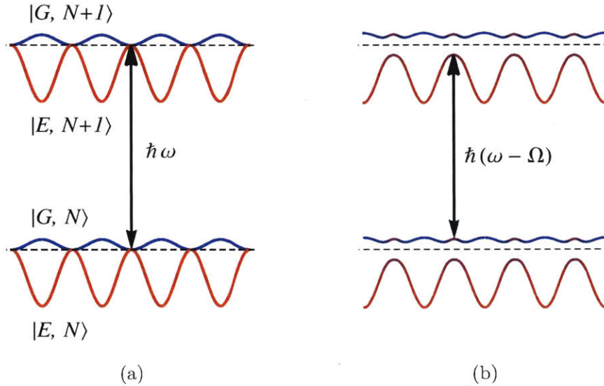
Figure 5-6: Dressed States at Zero Detuning. (a) When \Omega = 0 , the state |G, N\rangle ( |E, N\rangle ) coincides with |g, N\rangle ( |E, N - 1\rangle ). Dressed state |G, N\rangle is predominantly ground state, and is shown in blue, while |E, N\rangle is shown in red. As shown, |g\rangle experiences a trapping lattice potential, while |e\rangle is anti-trapped with 5.5 times the ground state trap depth. The arrow indicates the Stark-shifted resonance. (b) At \Omega \neq 0 , mixing of |g, N\rangle and |e, N - 1\rangle states occur. The admixture of |g\rangle and |e\rangle is shown by the color of the dressed state, and varies spatially. At the locations where the light is resonant, the dressed states are equal admixtures of |g\rangle and |e\rangle , and |G, N\rangle and |E, N\rangle forms a doublet that is split by \hbar\Omega . In this plot, \hbar\Omega = 2V_0 , where V_0 is the lattice depth experienced by the ground state |g\rangle .
