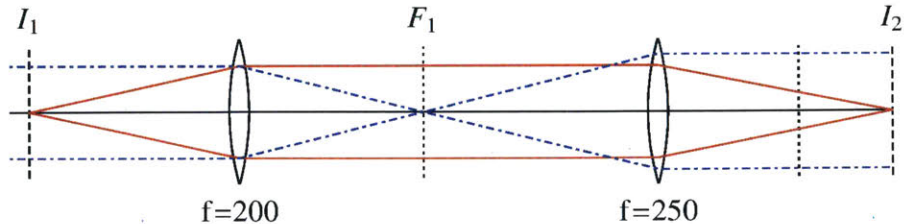
Figure 4-8: The “accordion” beam. The atoms are at I_1 ; focal lengths are in units of mm. The galvo mirror is placed in the image plane I_2 . An additional galvo with a 3 mm glass plate is placed \sim 30 mm after the galvo mirror.
