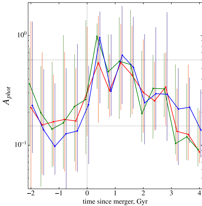
Figure 2. Evolution of A_{\text{phot}} for 26 simulated clusters over the course of a major ( M_1/M_2 > 0.5 ) merger. The solid colored lines show the median value of A_{\text{phot}} as a function of time since the merger for all 26 clusters along three different sight lines (blue and green are in the plane of the sky, while red is along the line of sight), while the vertical bars show the 1\sigma scatter. Horizontal lines at 0.15 and 0.6 show our divisions for relaxed and disturbed clusters, respectively. The vertical dotted line corresponds to the start of the merger. We find that, within 1 Gyr of the merger, \sim 70\% of the simulated images (over all three projections) have A_{\text{phot}} > 0.6 , while < 15\% of the pre- or post-merger systems have such high values, making A_{\text{phot}} > 0.6 a reasonable proxy for ongoing mergers.
