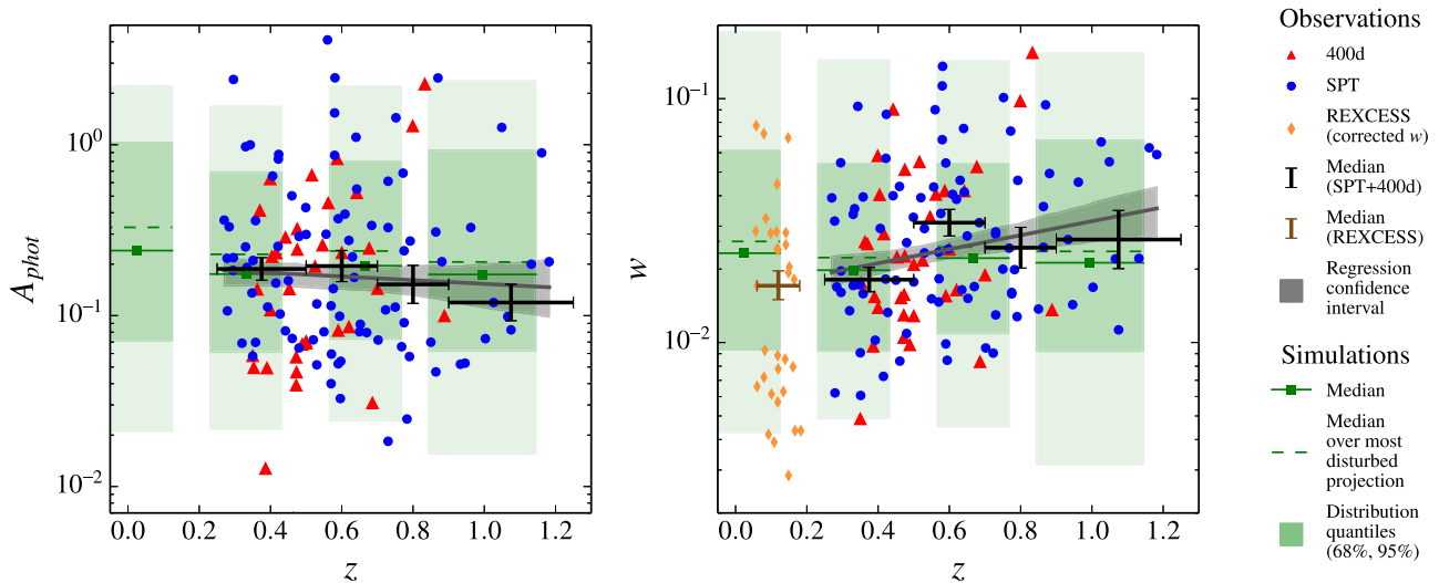
Figure 4. Redshift evolution of A_{\text{phot}} and w . Red triangles and blue circles represent 400d and SPT clusters respectively. Black error bars show the median values in four redshift bins ( [0.25-0.5] , [0.5-0.7] , [0.7-0.9] , [0.9-1.2] ). We measure Pearson R coefficients for the left and right panels of 0.02 and 0.19, respectively, indicating a lack of a statistically significant correlation. The error bars on the median value are obtained by the Median Absolute Deviation method and demonstrate that there is no significant difference in the median value between bins. The slopes, derived by a simple linear regressions of A_{\text{phot}} and w with z , are consistent with no redshift evolution at \sim 0.5\sigma and \sim 2\sigma respectively. The shaded green regions show the 68% and 95% ranges for A_{\text{phot}} and w in simulated clusters, with the medians shown as green squares. The orange circles in the right panel show the values of w for the REXCESS sample presented in Böhringer et al. (2010), accordingly corrected for the different w definition used in this study.
