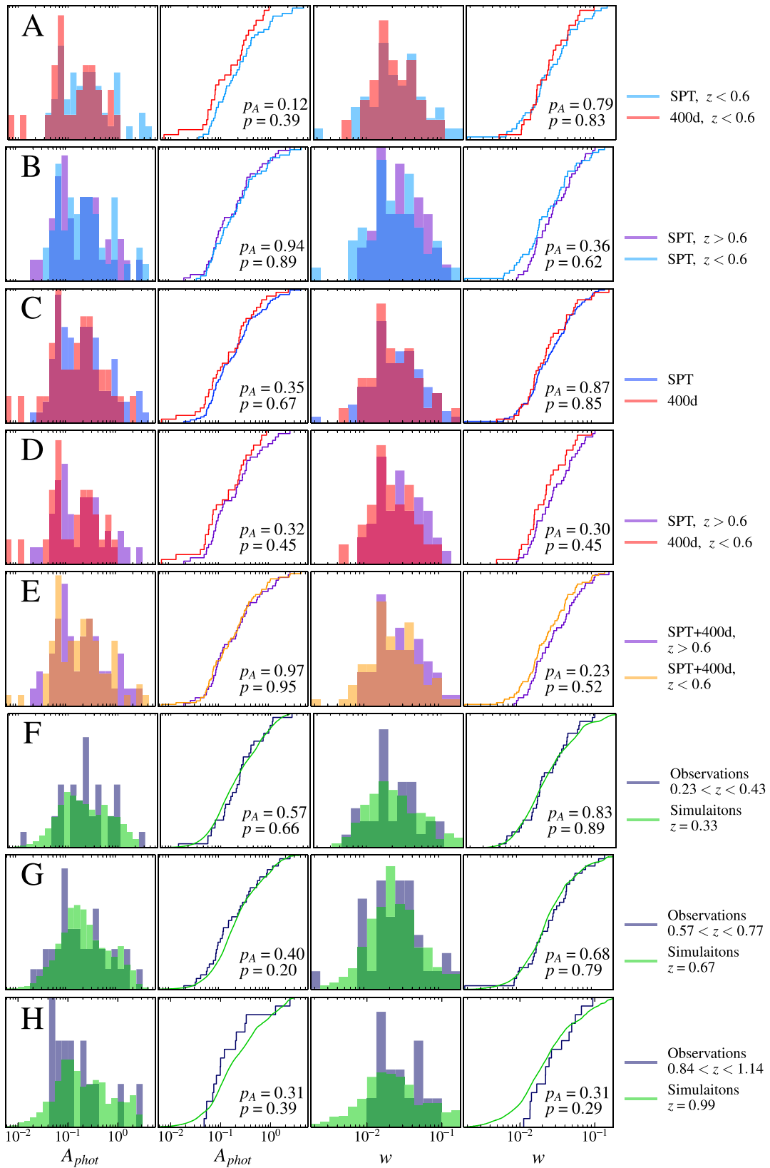
Figure 3. Distribution of morphological statistics for various partitions of clusters in the 400d and SPT catalogs. In each row, the left two plots show the histograms and cumulative distribution functions for A_{\text{phot}} , and the right two plots show the same for w . The p -value, based on the KS and AD tests, of the hypothesis that the substructure statistic values come from the same distribution are shown in each plot. High values of p indicate that the distributions are similar, low values of p indicate that the distributions are different. It is a common practice to exclude the null hypothesis at p < 0.05/(\text{number of tests being conducted}) . The rightmost column explains what samples are being compared. See Section 3 for the motivation of the subsamples to be compared and Section 4 for the description of the results.
