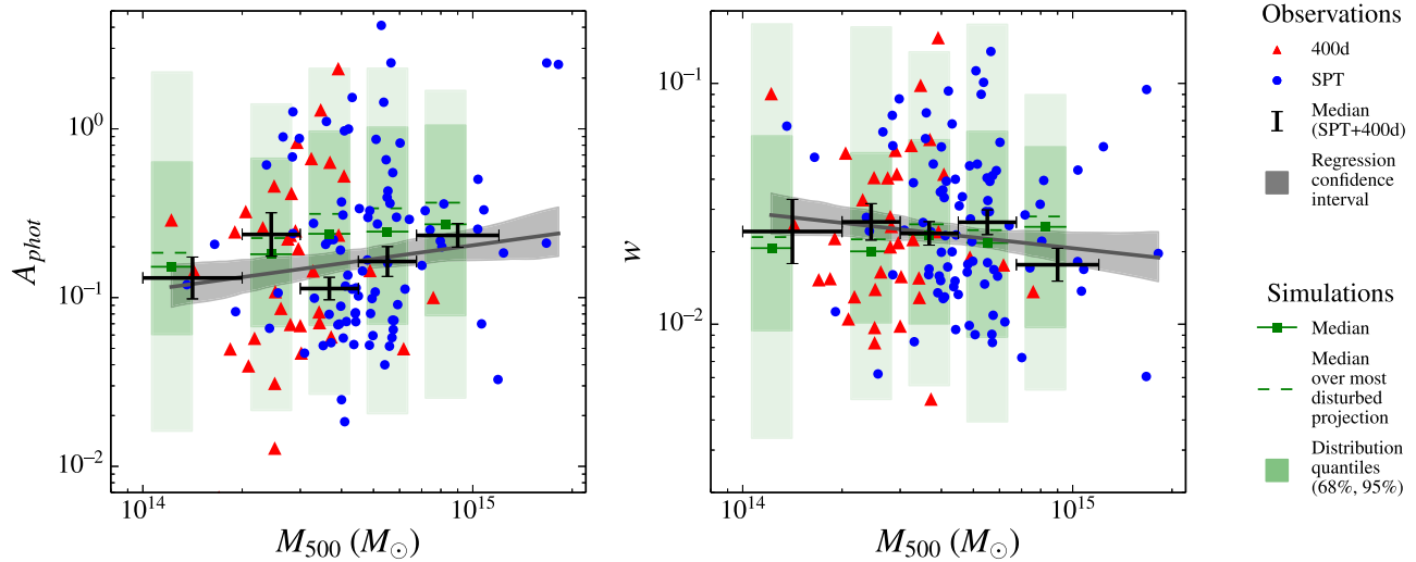
Figure 5. Similar to Figure 4, but now considering cluster mass rather than redshift. We measure Pearson R coefficients for the left and right panels of 0.19 and -0.11 , respectively, indicating a lack of a statistically significant correlation. There is no significant correlation between cluster asymmetry and mass, regardless of the asymmetry estimator used or whether we consider real or simulated clusters.
