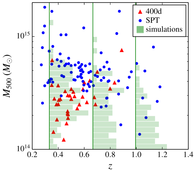
Figure 1. Masses and redshifts for SPT, 400d, and simulated samples. Red and blue dots show individual objects in the 400d and SPT samples, respectively. Green histograms show the distributions of masses for simulated clusters in three arbitrarily chosen redshifts bins—there are a total of 85 simulated clusters used for comparison to the data. The SPT and 400d samples have a reasonable overlap for z < 0.6 ; simulated clusters have a reasonable overlap with the observed clusters at all redshifts. We will show in Section 4.2 that the slightly different mass range for these samples should not significantly bias the distribution of observed morphologies.
