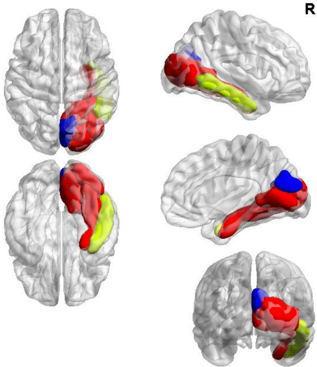
Figure 2. Modular organization differences between-groups with common affiliations within right fusiform and lingual gyri as well as lateral occipital and pericalcarine cortices (in red) with a higher degree of modular integration with heteromodal regions of the ventral visual processing stream in anchorers (right inferior temporal cortex in yellow) compared to the unimodal integration within right cuneus seen in non-anchors (in blue).
