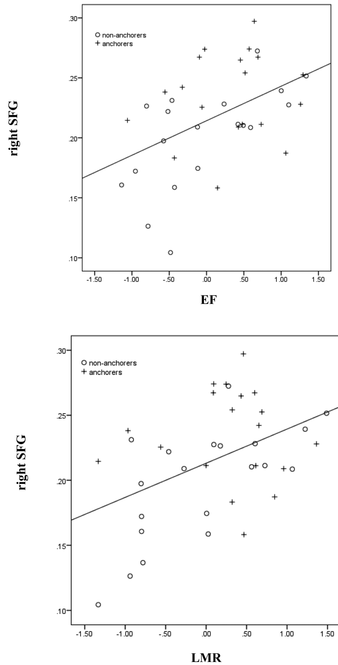
Figure 1. Scatterplots with trend lines of 2-tailed correlations between local efficiency metrics within the right superior frontal gyrus (rightSFG) and composite z-scores of executive functioning (EF; r(38)=.47 , p=.003 ) and learning/memory/recognition (LMR; r(39)=.45 , p=.005 ) stratified by group (anchorers labeled '+'; non-anchorers labeled 'o').
