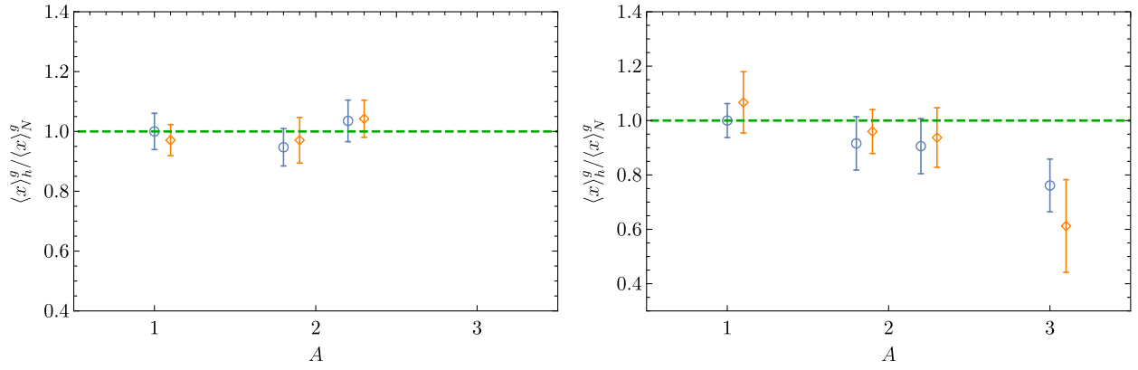
FIG. 5. Ratios of the gluon momentum fraction in the nucleon and light nuclei h = N, d, nn, {}^3\text{He} from left to right, to the central value of this quantity in the nucleon with SP source-sink smearing. The left and right panels show results for Ensemble A (with m_\pi \sim 450 MeV), and Ensemble B (with m_\pi \sim 806 MeV), respectively. The blue circles and orange diamonds denote results obtained using SP and SS source-sink smearing combinations. The green dashed line is at 1, shown to guide the eye.
