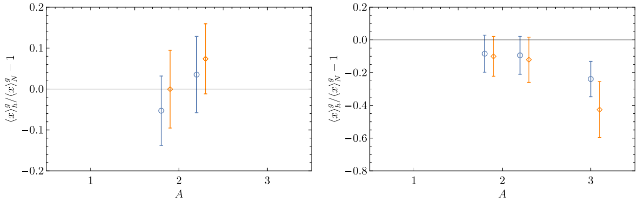
FIG. 6. Differences from unity of the ratios of the gluon momentum fraction in the nucleon and light nuclei h = N, d, nn, {}^3\text{He} from left to right, to the nucleon with the same source-sink smearing. The left and right panels show results for Ensemble A (with m_\pi \sim 450 MeV), and Ensemble B (with m_\pi \sim 806 MeV), respectively. The blue circles and orange diamonds denote results obtained using SP and SS source-sink smearing combinations.
