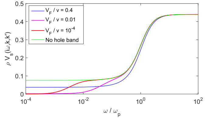
FIG. 9. The averaged interaction (18) vs frequency for three values of \delta_v = V_F/v = 0.4, 0.01, 10^{-4} and the case where the hole band is absent. Here we took |k - k'| = 0.25k_F . As can be seen, T_c goes down smoothly with increasing \delta_v around this point. In the case of \delta_v = 0.01 and 10^{-4} , the retardation effect of the acoustic plasmon is clearly seen at \omega \sim 0.1 and 10^{-2} \omega_p , respectively.
