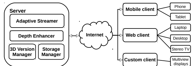
Figure 1: Design of the proposed 3D streaming system. The Depth Enhancer customizes the depth based on display sizes and viewing conditions. The creation of multiple versions of each 3D video is managed by the 3D Version Manager, and the storage of these versions is handled by the Storage Manager. The Adaptive Streamer uses DASH to serve segments of different versions to various clients.
