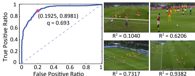
Figure 8: Left: ROC curve for our binary shot classifier. Right: Four examples of shots with corresponding R^2 values. Top two have low R^2 value, therefore, their depth will be unchanged. On the other hand, bottom two are long shots and due to the high R^2 value (above the threshold) their depth will be modified.
