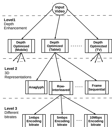
Figure 2: 3D Version Tree. It serves as an execution or master plan to create different versions of each 3D video.
