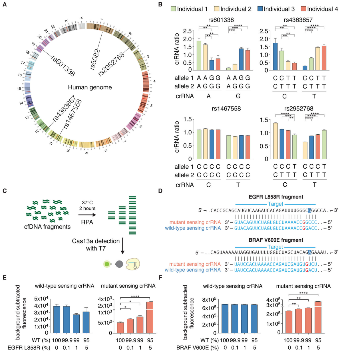
Figure 4. SHERLOCK can discriminate SNPs for human genotyping and cell-free allele DNA detection
