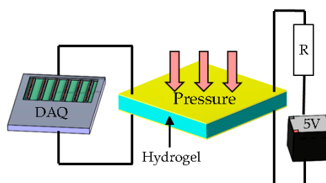
Figure 1. A schematic showing the experimental set up of hydrogel capacitive pressure sensor.
