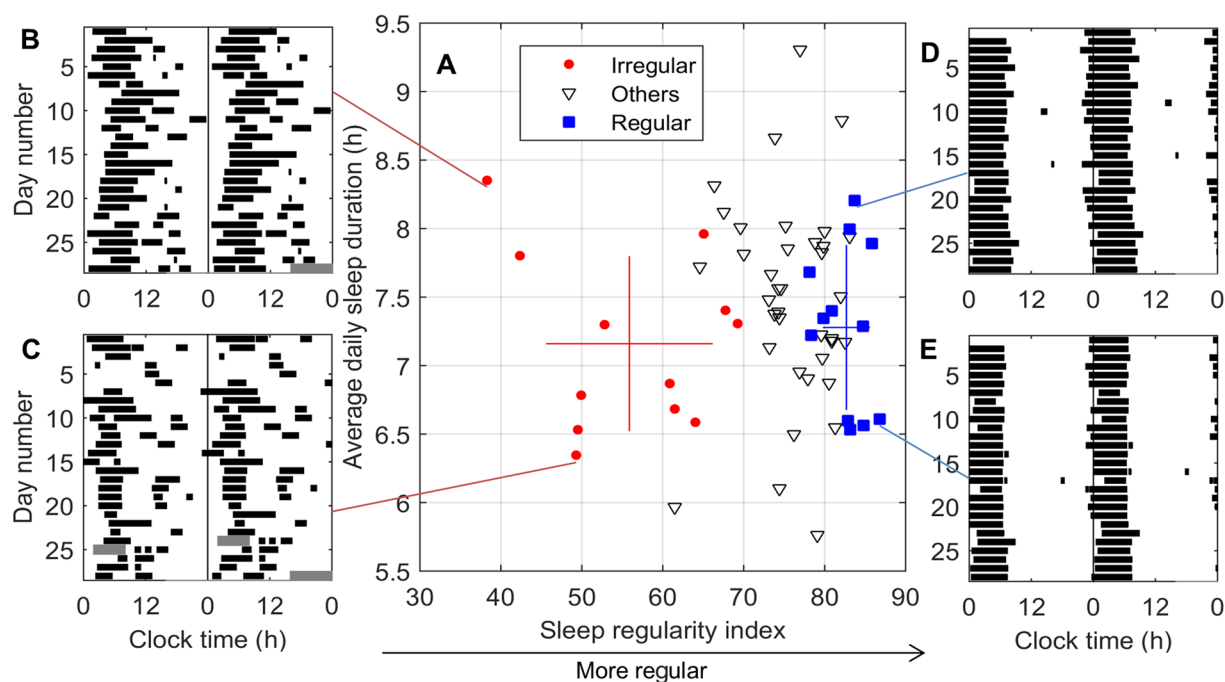
Figure 1. Two dimensions of sleep: duration and regularity. (A) Average daily sleep duration vs. sleep regularity index (SRI) for all participants ( n = 61 ) assessed across the whole study interval. Participants identified for the Irregular ( n = 12 ) and Regular ( n = 12 ) groups at the study mid-point are red circles and blue squares, respectively. Other individuals are white triangles. As explained in the Methods, the SRI values differed slightly by end of study, so those identified as most extreme at the study midpoint did not necessarily remain most extreme at end of study; however, the differences between Regular and Irregular groups remained highly significant (see Results). Error bars indicate mean and standard deviation for Regular and Irregular groups in both SRI and sleep duration. Sleep patterns for four participants collected using daily diaries are shown using double-plotted raster diagrams, where black bars indicate episodes of sleep and gray bars indicate missing data. Four examples are displayed: (B) an Irregular long sleeper, (C) an Irregular short sleeper, (D) a Regular long sleeper, and (E) a Regular short sleeper.
