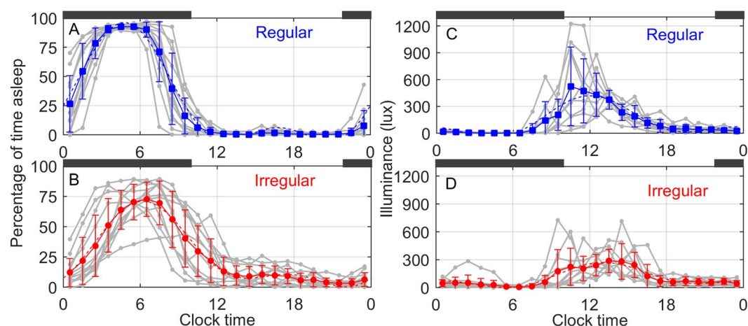
Figure 2. Sleep/wake and light/dark cycles differ between Regular and Irregular groups. Gray lines show individual data ( n = 12 for each sleep/wake panel and n = 11 for each light/dark panel). Colored lines show group mean and standard deviation in one-hour bins, with data for each individual averaged across the whole study interval (i.e., multiple days). Dark gray bars indicate clock night (22:00 to 10:00). Left panels: Sleep/wake rhythm (percentage of time asleep) for (A) Regular and (B) Irregular sleepers. Right panels: Normalized light levels for (C) Regular and (D) Irregular sleepers.
