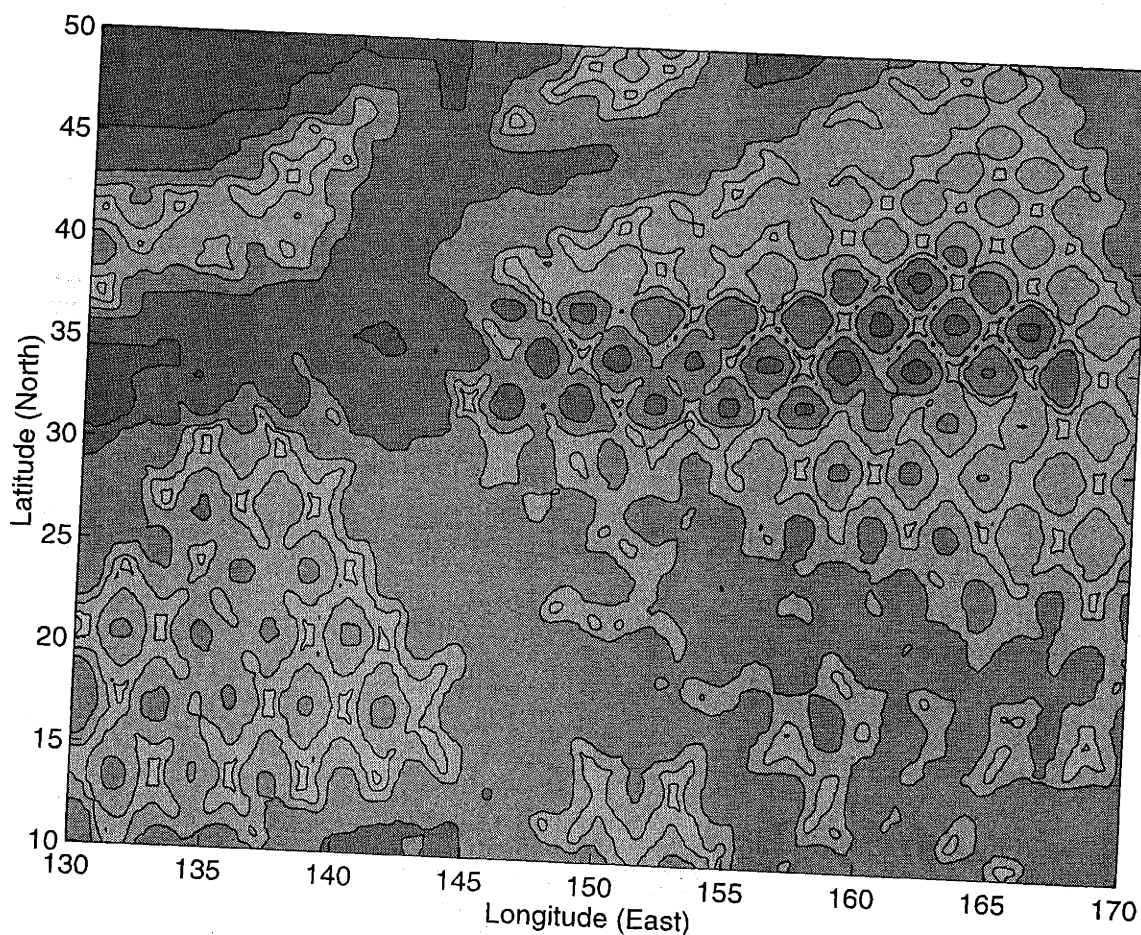
Figure 3-14: Estimation error variances corresponding to the elevation estimates of Figure 3-13. Darker regions represent greater uncertainty.
