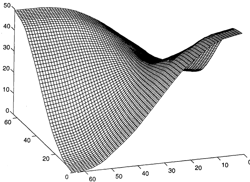
Figure 7-12: The multiscale reconstruction from the height measurements in Figure 7-7 (b), plus regularly sampled measurements (4% measurement density) of the surface gradients.
