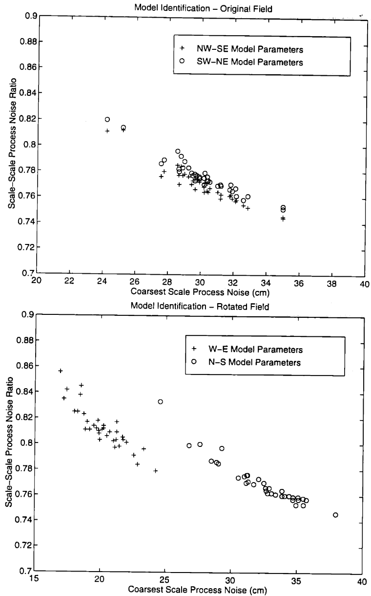
Figure 4-4: Two examples of isotropic oceanographic spectrum identification. In each example one set of spectral parameters ( B_1, \gamma_1, B_2, \gamma_2 ) was identified for each of 37 ten-day TOPEX/POSEIDON data sets. Top Figure: spectral identification results along NW-SE and SW-NE directions. Bottom Figure: spectral identification results along W-E and N-S directions.
