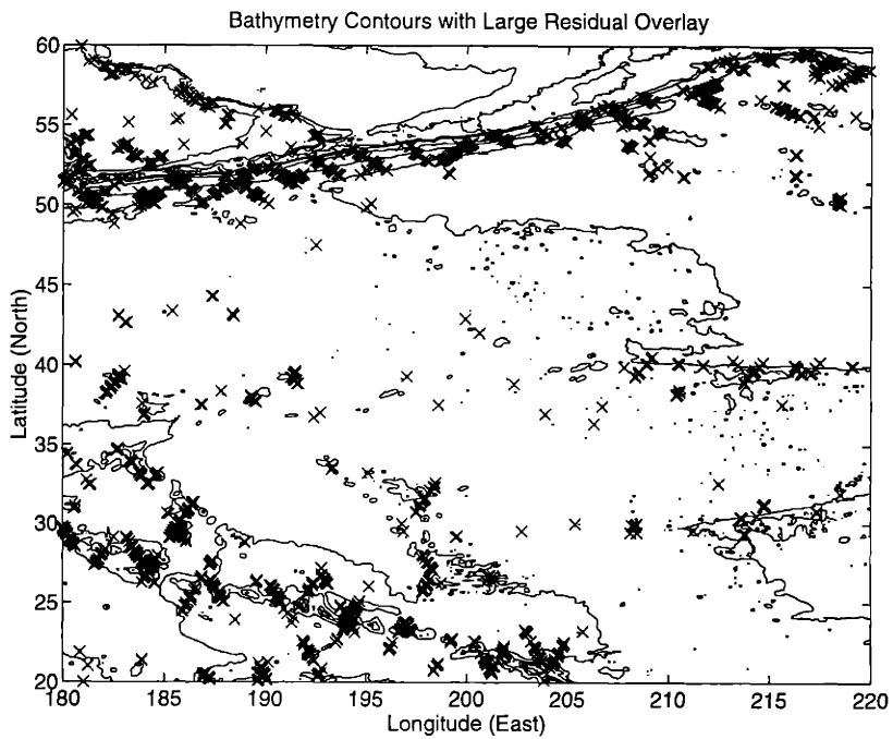
Figure 3-16: Overlay of geoid gradient map (in (a)) and of ocean bathymetry contours (in (b)) with the distribution of locations of large residuals; regions of lighter shading represent steeper geoid gradient. The striking correlation exhibited in these figures motivates the correction of Figure 3-17.
