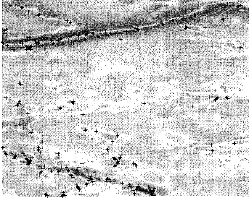
Figure 5-8: A plot showing the distribution of those measurement residuals (each marked with a '+' sign) in excess of 1.5\sigma superimposed on \Delta G_{ANOM} — a function which we believe to be strongly correlated with errors in the OSU91A geoid estimates. Darker regions represent larger values of \Delta G_{ANOM} .
