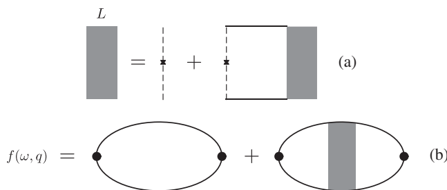
FIG. 3. (a) Resummation of disorder rungs. (b) Relation between L(\omega, \mathbf{q}) and f(\omega, \mathbf{q}) .
