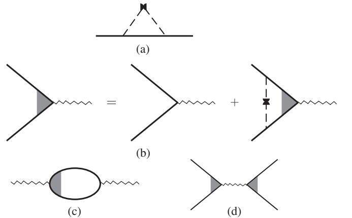
FIG. 2. (a) The impurity self-energy leading to the elastic lifetime in Eq. (2.3). (b) Disorder correction to the electron interaction vertex in Eq. (2.6); here and henceforth, the electron lines contain the effect of the impurity self-energy. (c) Dynamical screening of the interaction by the disorder-corrected polarization bubble in Eq. (2.7). (d) The 2-in, 2-out process that provides the inelastic electron lifetime; here and henceforth, the interaction line is the dynamically screened interaction.
