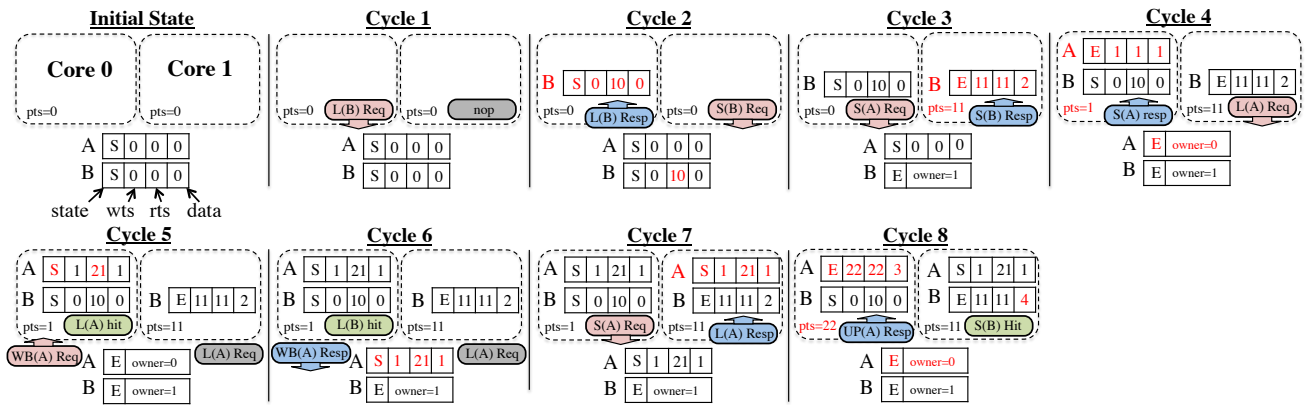
Fig. 3. Execution of the case study program with Tardis protocol.
