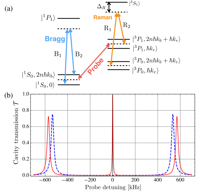
FIG. 3. (a) Level diagram for the generation of squeezed momentum states enhanced by induced transparency via the ^3P_0 state. The Bragg laser beams are indicated as B_1 and B_2 . The effective control field that couples the states ^3P_0 and ^3P_1 is obtained by two-photon Raman coupling via the ^3S_1 intermediate state. The two Raman beams R_1 and R_2 operate at the wavelengths 679 nm ( ^3P_0 – ^3S_1 ) and 688 nm ( ^3P_1 – ^3S_1 ), respectively, and are detuned from the transition to the ^3S_1 state by \Delta_R . (b) Cavity transmission spectrum with (red solid line) and without (blue dashed line) Raman coupling to the ^3P_0 state for \Omega_{\text{eff}} = 2\pi \times 400 kHz, N\eta = 3 \times 10^3 , and n = 1 . The two lateral peaks correspond to the vacuum Rabi splitting for \kappa = 2\pi \times 50 kHz. The population measurement is performed at the frequency of the transparency region (at probe detuning \delta = 0 ), which corresponds to a linewidth of \kappa_{\text{EIT}} = 2\pi \times 6 kHz.
