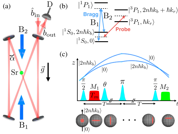
FIG. 1. (a) Schematic setup with the probe field \hat{b}_{\text{in}} coupled to the optical cavity and interacting with the atoms (green circle) through the oblique beam with angle \alpha with respect to gravity. The reflected field \hat{b}_{\text{out}} is measured by the detector D . The atomic states are manipulated through the Bragg beams B_1 and B_2 . (b) Level diagram for probing on the ^1S_0 - ^3P_1 transition (red arrow) and for momentum-state manipulation through Bragg diffraction on the ^1S_0 - ^1P_1 transition (blue arrows). (c) Interferometer trajectories and measurement sequence. The interferometer is formed by a \pi/2 - \pi - \pi/2 Mach-Zehnder sequence with interrogation time T . The cavity-enhanced squeezing measurement with duration T_m is indicated as M_1 . The Bragg pulse \theta induces a phase-sensitive state for the interferometer, and the final readout measurement is performed ( M_2 ). Lower part: Bloch sphere representation of the state evolution.
