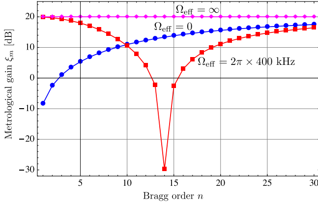
FIG. 2. Expected metrological gain \xi_m as a function of the Bragg diffraction order n , assuming perfect detection efficiency \epsilon_d = 1 , and for N\eta = 10^4 . The blue circles refer to the scheme shown in Fig. 1(b). Values shown as red squares and magenta diamonds refer to the scheme in Fig. 3(a), where electromagnetically induced transparency (EIT) is present with \Omega_{\text{eff}} = 2\pi \times 400 kHz and with perfect transparency \Omega_{\text{eff}} = \infty , respectively.
