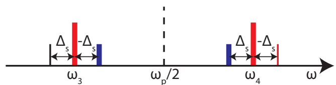
FIG. 5. Frequency diagram of the four-mode amplification. The dashed line is the parametric pump, the thick red lines are the parametric oscillations, the thin black line is the coherent signal, the thin red line is the primary idler, and the thick blue lines are the secondary idlers.
