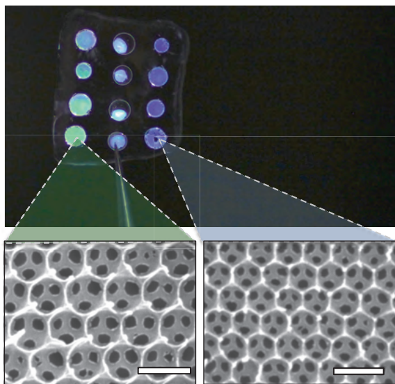
Fig. 3. Silk inverse opals showing structural color. Reprinted by permission from [109], Copyright 2012, Macmillan Publishers Ltd.
