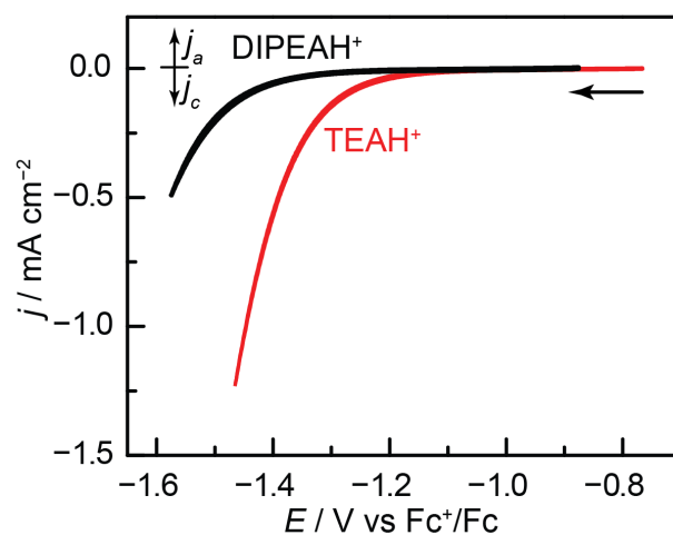
Figure 1. Cyclic voltammograms (20 mV s -1 ) of polycrystalline Au recorded in acetonitrile containing 0.1 M TBA PF 6 , 20 mM DIPEAH + OTf - (black) and 20 mM TEAH + OTf - (red).
