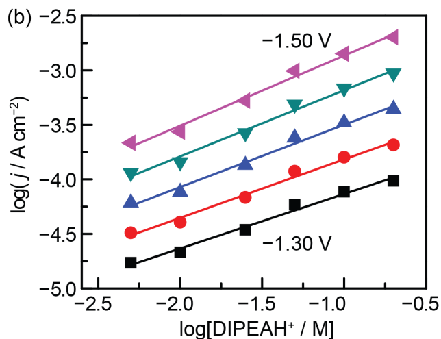
Figure 3. Hydrogen evolution catalytic current density vs concentration of TEAH + (a) and DIPEAH + (b). Traces correspond to potentials spaced in 50 mV increments ranging between -1.30 and -1.45 V for TEAH + and -1.30 and -1.50 V for DIPEAH + . Current densities were recorded on polycrystalline Au in acetonitrile containing 0.5 M TBA PF 6 . The slopes range from 0.45 to 0.63 for TEAH + and from 0.50 to 0.64 in DIPEAH + .
