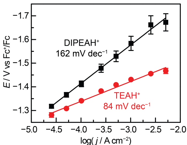
Figure 2. Potential vs activation controlled current density for hydrogen evolution catalysis on polycrystalline Au recorded in acetonitrile containing 0.5 M TBA PF 6 , 25 mM DIPEAH + OTf - (black) and 25 mM TEAH + OTf - (red). Both electrolytes contained 2.5 mM of the corresponding conjugate base. Tafel slopes were 162 mV dec -1 and 84 mV dec -1 , respectively.
