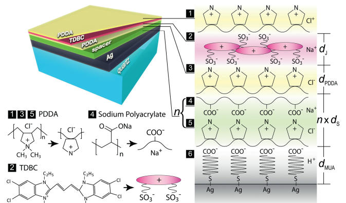
Fig. 2. Schematics of the grown molecular multilayer structure. The layers are formed one by one by the adsorption between positively and negatively charged molecules. From the bottom to the top, it consists of 100 nm Ag, a MUA bonding layer, a (PDDA/PolyArc) _n spacer layer, and a (PDDA/TDBC/PDDA) cyanine layer encapsulated in PDDA.
