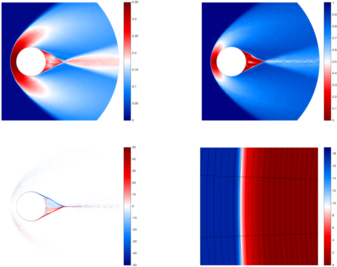
Figure 5: Snapshot of the non-dimensional temperature c_p T / \gamma u_\infty^2 (top left), velocity magnitude |\mathbf{v}| / u_\infty (top right) and vorticity d(\nabla \times \mathbf{v}) / u_\infty (bottom left) fields for the hypersonic cylinder. A zoom of the Mach number field around the center of the shock is shown in the bottom right image. Despite the high incident Mach number M_1 = 17.6 , the shock is non-oscillatory and resolved within three elements.
