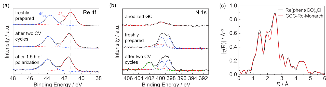
Figure 1. (a) High-resolution Re 4f XPS spectra of freshly prepared GCC-Re (top), GCC-Re following two CV cycles (middle) and GCC-Re following 1.5 h of cathodic electrolysis at 1.0 \text{ mA/cm}^2 (bottom). (b) High-resolution N 1s XPS spectra of an oxidized GC electrode (top), freshly prepared GCC-Re (middle), and GCC-Re following two CV cycles (bottom). (c) k^2 -weighted magnitude of the Fourier transform of the extended X-ray absorption fine structure ( \Delta k = 2.6\text{-}11.9 \text{ \AA}^{-1} ) of \text{Re}(\text{phen})(\text{CO})_3\text{Cl} (black) and GCC-Re modified Monarch 1300 (Red). The imaginary parts of the Fourier transform (not shown) of \text{Re}(\text{phen})(\text{CO})_3\text{Cl} and GCC-Re modified Monarch carbon powder are also identical.
