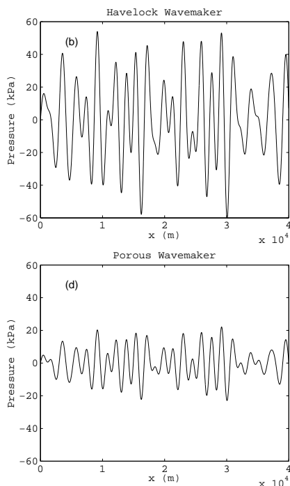
Fig. 4 Acoustic-gravity waves generated by a \delta -function wavemaker in the ocean placed at z = -12.5 m for f = 1 Hz. The ocean is h = 4000 m deep and the speed of sound is c = 1500 m/s. (a), (c) Vertical distribution of the velocity amplitude at x = 15 m, 9525 m, and 14985 m away from the wavemaker. (b), (d) Horizontal distribution of the pressure amplitude at the bottom of the flume. (a), (b) Havelock's wavemaker theory; (c), (d) porous wavemaker theory.
