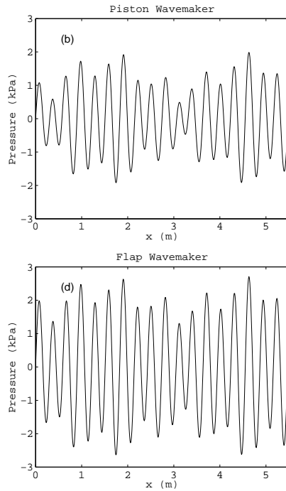
Fig. 2 Acoustic-gravity waves generated by a wavemaker in a wave flume for f = 5 kHz based on the Havelock's wavemaker theory; L = 5.5 m, h = 0.5 m, b = 1 m, c = 1500 m/s. The motion of the plate is limited by the constraint that, the horizontal movement \leq 2.1 m, the horizontal velocity \leq 3.8 m/s, horizontal acceleration \leq 19.6 m/s 2 (parameters come from the unidirectional wavemaker in O.H. Hinsdale Wave Research Laboratory, Oregon State University). (a), (c) Vertical distribution of the velocity amplitude at x = 0.04 m, 0.39 m, and 0.79 m away from the wavemaker. (b), (d) Horizontal distribution of the pressure amplitude at the bottom of the flume. (a), (b) piston wavemaker; (c), (d) flap wavemaker.
