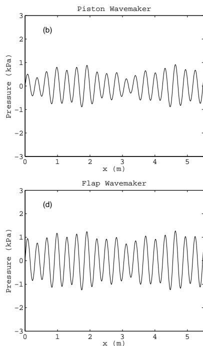
Fig. 3 Acoustic-gravity waves generated by a wavemaker in a wave flume for f = 5 kHz based on the porous wavemaker theory; L = 5.5 m, h = 0.5 m, b = 1 m, c = 1500 m/s. The motion of the plate is limited by the constraint that, the horizontal movement \leq 2.1 m, the horizontal velocity \leq 3.8 m/s, horizontal acceleration \leq 19.6 m/s 2 (parameters come from the unidirectional wavemaker in O.H. Hinsdale Wave Research Laboratory, Oregon State University). (a), (c) Vertical distribution of the velocity amplitude at x = 0.04 m, 0.39 m, and 0.79 m away from the wavemaker. (b), (d) Horizontal distribution of the pressure amplitude at the bottom of the flume. (a), (b) piston wavemaker; (c), (d) flap wavemaker.
