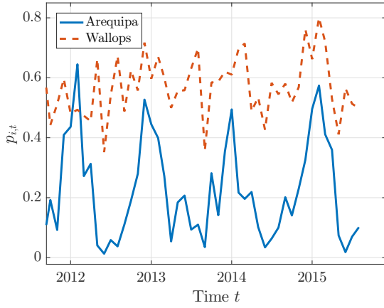
Figure 5: Cloud Fraction Time Series
