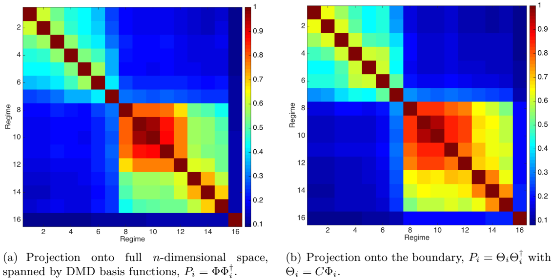
Figure 10. The subspace alignment measure \gamma_{ij} from (32).
