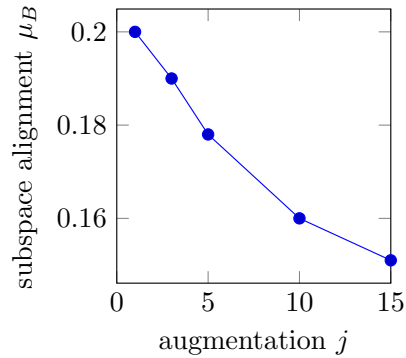
Figure 13. Block coherence measure \mu_B as a function of augmentation j using only sensors on the boundary.
