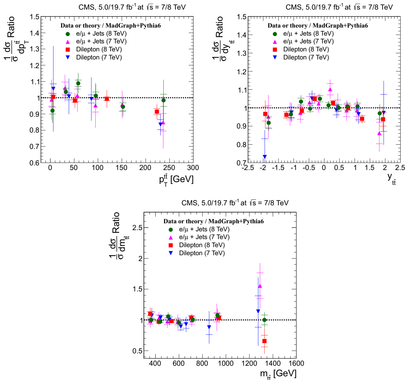
Fig. 19 Comparison of normalized differential t\bar{t} production cross section in the dilepton and \ell +jets channels at 7 TeV [5] and 8 TeV, as a function of the p_T^{\bar{t}} (top left), y_{t\bar{t}} (top right), and m_{t\bar{t}} (bottom) of the t\bar{t} system. The measurements are presented relative to the corresponding MADGRAPH+PYTHIA6 predictions. A horizontal bin-centre correction
