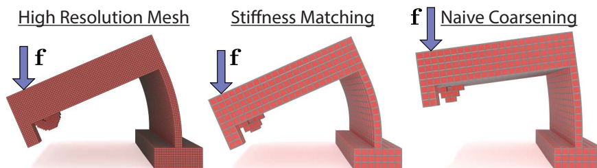
Figure 4-7: Static Deformation Test. We apply an identical load to three meshes with the same model geometry. With the same material parameters, a high-resolution mesh (left) is effectively 2.5x softer than the corresponding coarse mesh (right). Applying our captured numerical Young's modulus to the coarse mesh (middle) regains the correct deformation of the original, high-resolution mesh on the left.
