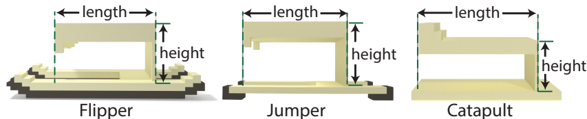
Figure 4-18: Design geometries and parameters.
