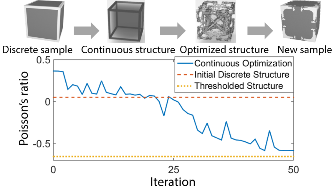
Figure 3-3: The continuous sampling step uses topology optimization to expand the gamuts by refining existing structures. A good starting point is necessary for the optimization to find better solutions. We use discrete microstructures near the boundary to initialize topology optimization. At convergence, we threshold the values to obtain a new discrete sample.
