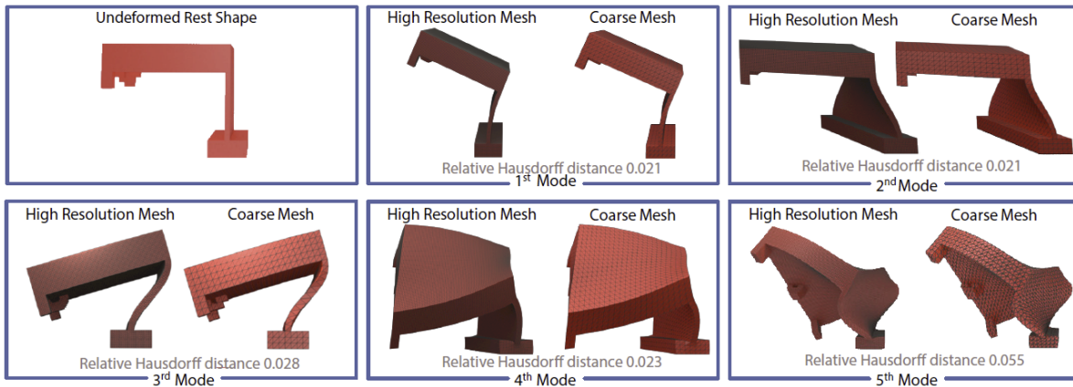
Figure 4-6: Dynamics-aware coarsening (DAC) coarsens meshes to capture deformation with calibrated stiffness. We observe FE meshes capture accurate deformation modes up to a quite coarse resolution. However, these same coarse meshes suffer from numerical stiffening (see Figure 4-7). We design coarse mesh FE models by matching both significant deformation modes (above) and their captured material response (see Figures 4-10 and 4-20) to obtain efficient and predictive coarse-mesh FEM simulations of dynamics.
