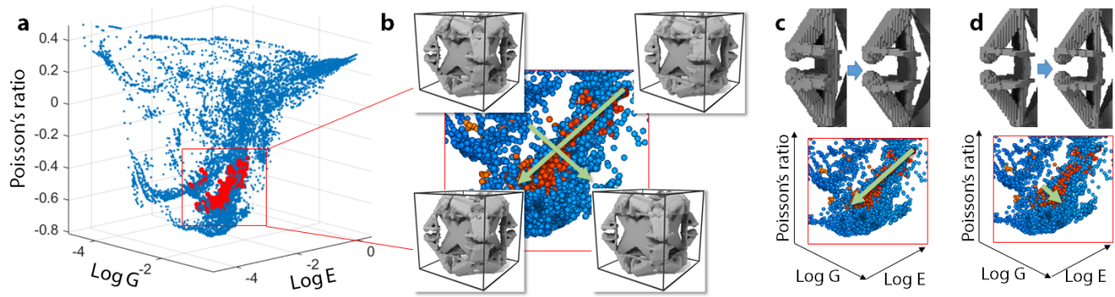
Figure 3-11: Reduced parameters for Family 4. The distribution of the parameters corresponding to Family 4 is shown as red points in (a). The two principal directions are shown as green arrows in (b). The first direction reduces the Young’s modulus and Poisson’s ratio by decreasing the joint thickness (c). The second direction increases the shear modulus by slightly rotating the triangle joints outward (d).
