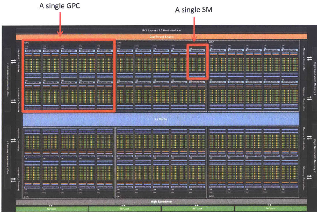
Figure 2-15: Overall architecture of the NVIDIA Pascal GP100 GPU [34].
