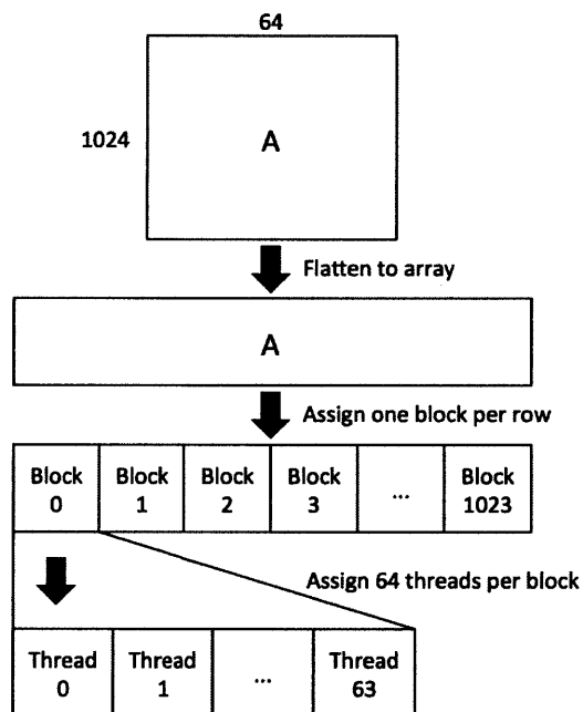
Figure 4-7: Mapping matrix A as a 1D grid of 1024 1D blocks, each containing 64 threads. Matrices B and C would be similarly mapped.
