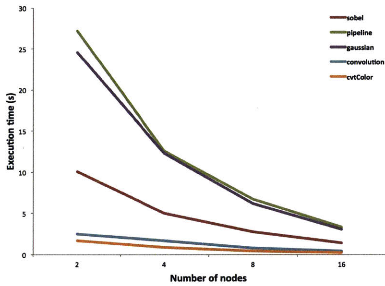
Figure 5-5: The performance of our distributed system across 2, 4, 8, and 16 CPU nodes.
