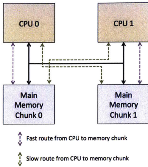
Figure 2-2: NUMA (non-uniform memory access) configuration.
