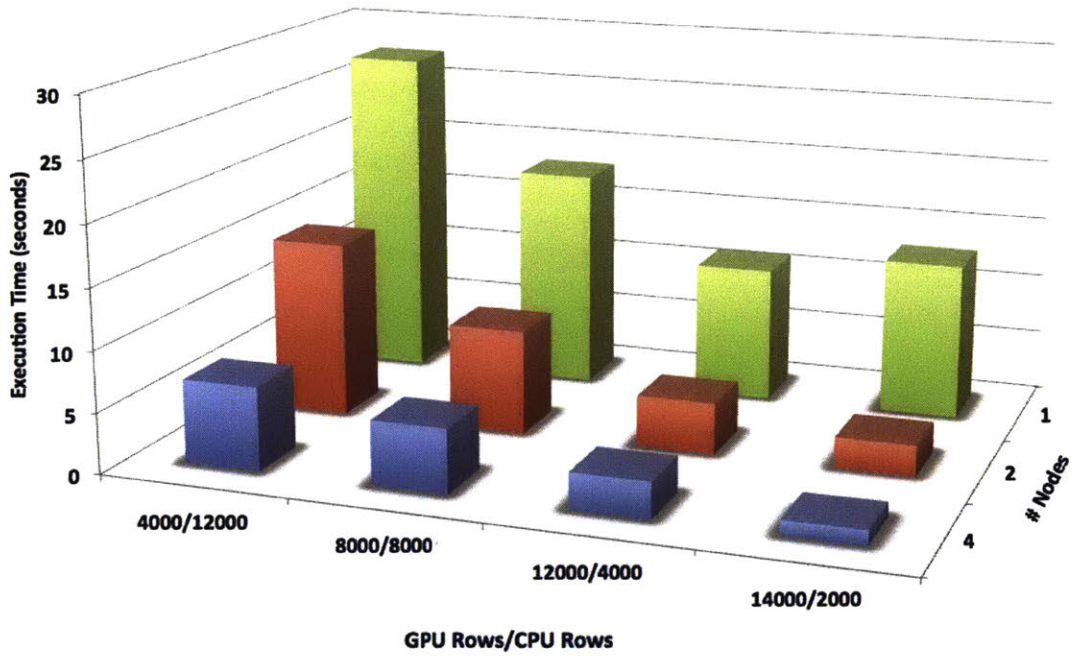
Figure 5-3: 3D chart for blur with cooperative execution using asynchronous execution and communication.
