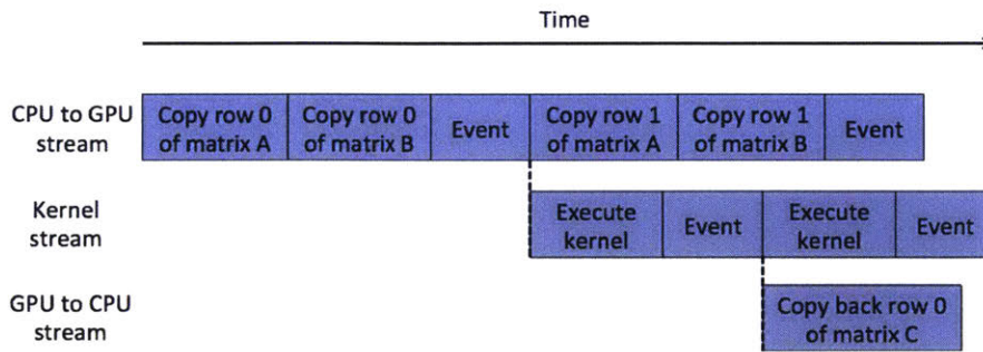
Figure 2-22: Timeline for kernel execution and communication using a combination of synchronous and asynchronous CUDA operations.
