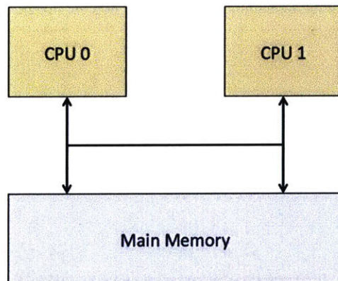
Figure 2-3: UMA (uniform memory access) configuration.
