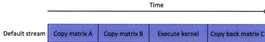
Figure 2-20: Timeline for kernel execution and communication using only synchronous CUDA operations.
