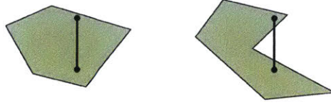
Figure 3-2: A convex (left) vs non-convex polyhedron.
