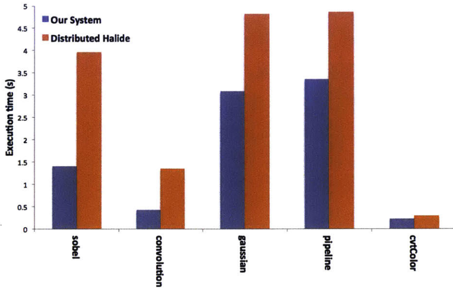
Figure 5-4: Results comparing the performance of our distributed system versus Distributed Halide on 16 CPU nodes.
