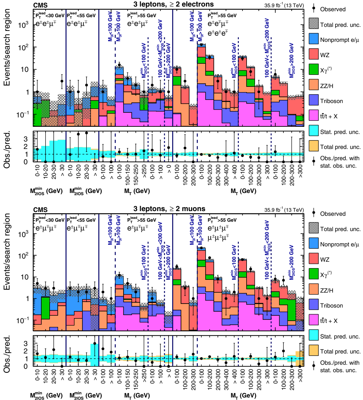
FIG. 1. Observed and expected event yields as a function of M_{2\ell OS}^{min} and M_T for events with at least two electrons (upper), and with at least two muons (lower). The contribution of each background source is shown. The first 8 bins of each figure correspond to the low-mass region, while the rest display the high-mass region.
