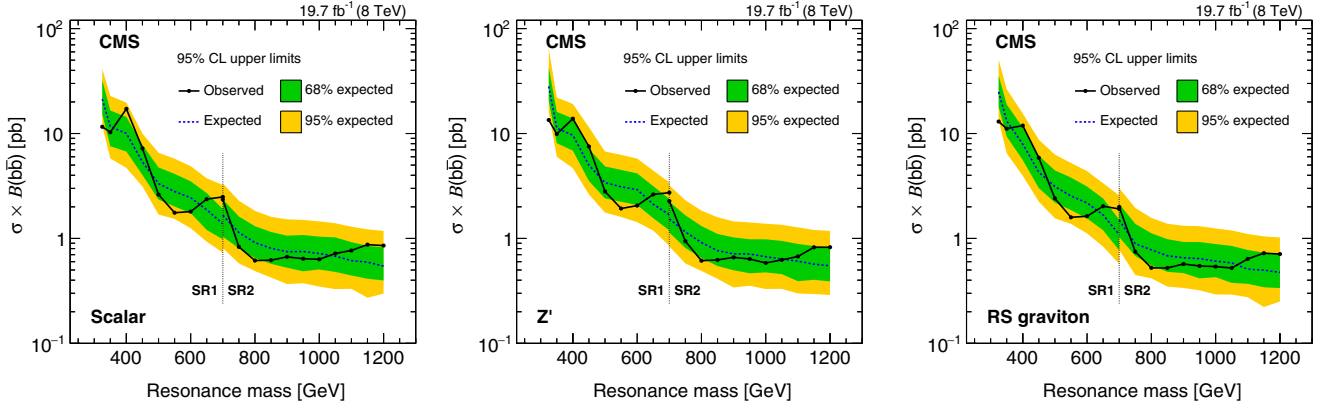
FIG. 3. Observed and expected 95% CL upper limits on the product of cross section and branching fraction to bottom quark-antiquark pairs for a scalar resonance (left), Z' boson (middle), and RS graviton (right) signal models, as functions of resonance mass. The discontinuity in the limits at 700 GeV is associated with a change in the acceptance from SR1 to SR2.
