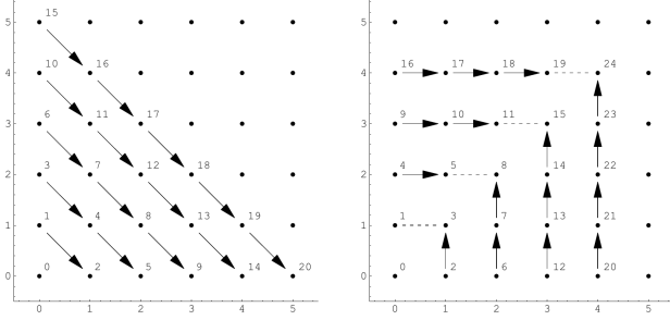
Figure 6: Cantor and Szudzik pairing functions
