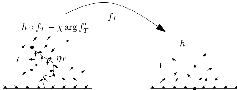
Figure 2.3: Forward coupling with arrows in e^{ih/\chi} direction (sketch), illustrating the constant angle gap between the two sides of the curve \eta , constant angles along the positive and negative real axes, and random angles (not actually point-wise defined if h is the GFF) in \mathbb{H} \setminus \eta .
