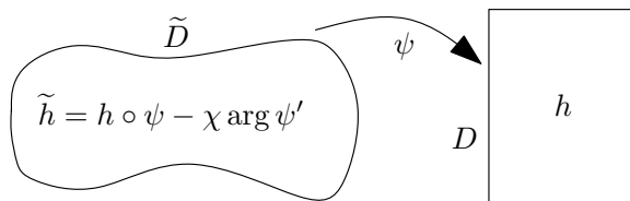
Figure 1.2: An AC surface coordinate change.
