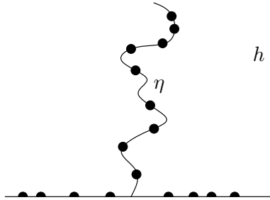
Figure 1.5: Sketch of \eta with marks spaced at intervals of the same \nu_h length along \partial D_1 and \partial D_2 . Here (-\infty, 0] and [0, \infty) are the two open strands of the “zipper” while \eta is the closed (zipped up) strand. Semicircular dots on \mathbb{R} are “zipped together” by f_t^h . Circular dots on \eta are “pulled apart” by f_t^\eta . (Recall that under the reverse Loewner flow f_t^h , the center of a semicircle on the negative real axis will reach the origin at the same time as the center of the corresponding semicircle on the positive real axis.) The law of ((D_1, h^{D_1}), (D_2, h^{D_2})) is invariant under “zipping up” by t capacity units or “zipping down” by t capacity units.
