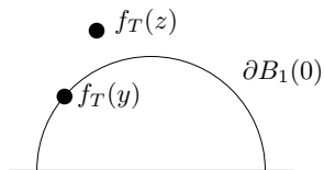
Figure 5.2: Assume that |f_T(y)| = 1 and |f_T(z)| > 1 + C and consider the reverse Loewner flow driven by W_t = \sqrt{\kappa}B_t . Claim: for some C_1, C_2 > 0 (depending only on C ) there is at least a C_1 probability that \mathfrak{h}_t(z) - \mathfrak{h}_t(y) changes by at least C_2 after time T .
