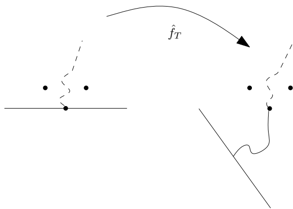
Figure 5.1: The map \hat{f}_T is first normalized so that \hat{f}_T(i-1) = (i-1) and \hat{f}_T(i+1) = i+1 . (Here i \pm 1 are shown as dots; a curve \eta and its image under \hat{f}_T is also shown.) The limit \hat{f}_\infty(z) := \lim_{t \rightarrow \infty} \hat{f}_t(z) a.s. exists as a conformal map from \mathbb{H} to the complement in \mathbb{C} of a semi-infinite path from some starting point to \infty .
