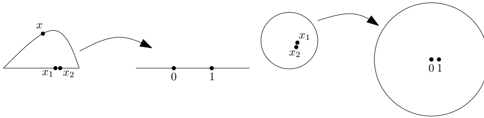
Figure 6.1: Constructing unit area/length quantum disc (left) or unit area quantum sphere (right). When C is large, we expect x_1 and x_2 to be close with high probability, and for most quantum area to be near those points.
