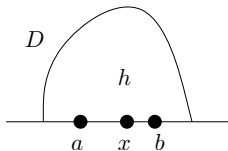
Figure 1.6: Point x sampled from \nu_h (restricted to [a, b] ).
