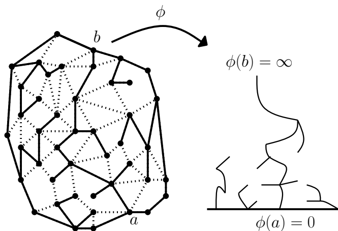
Figure 2.4: Planar map with a distinguished outer-boundary-plus-one-chord-rooted spanning tree (solid black edges), with chord joining marked boundary points a and b , plus image of tree under conformally uniformizing map \phi to \mathbb{H} (sketch).
