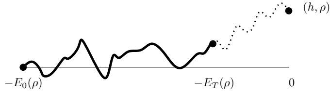
Figure 4.1: The pair (-E_t(\rho), (\mathfrak{h}_t, \rho)) traces the graph of a Brownian motion (solid curve) as t ranges from 0 to T . Conditioned on this, the difference between (h, \rho) and (\mathfrak{h}_T, \rho) is a centered Gaussian of variance E_T(\rho) . Choosing (h, \rho) to be (\mathfrak{h}_T, \rho) plus a Gaussian of this variance is equivalent to continuing the Brownian motion parameterized by -E_t(\rho) time (solid curve) all the way to time zero (dotted curve) and letting (h, \rho) be its value at time zero.
