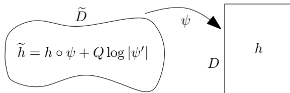
Figure 1.1: A quantum surface coordinate change.
