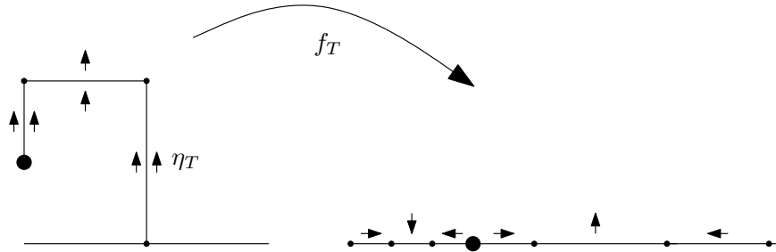
Figure 2.2: Winding number along \eta_T determines \arg f'_T , which is the amount a small arrow near \eta_T is rotated by f_T .
