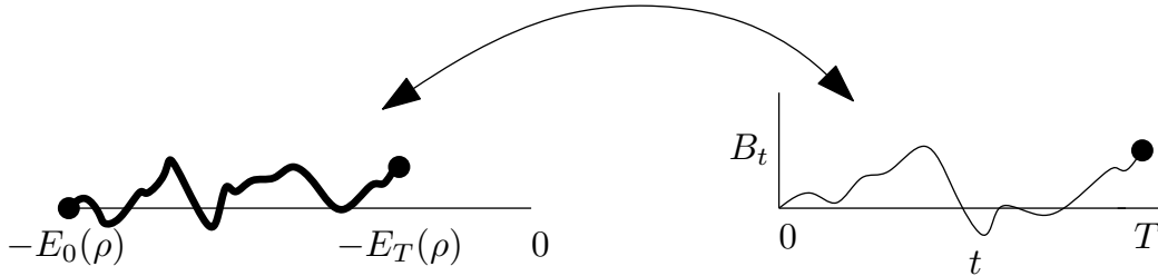
Figure 4.2: The graph traced by (-E_t(\rho), (\mathfrak{h}_t, \rho)) as t ranges from 0 to T (left) and the graph traced by (t, B_t) (right), where W_t = \sqrt{\kappa}B_t . The left graph uniquely determines the right graph, and vice versa, almost surely. Each has the law of a standard Brownian motion (up to a stopping time).
