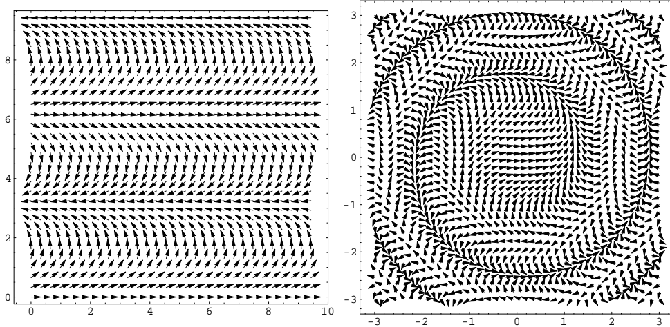
Figure 2.1: The complex vector flow e^{ih} : h(x, y) = y , h(x, y) = x^2 + y^2 .
