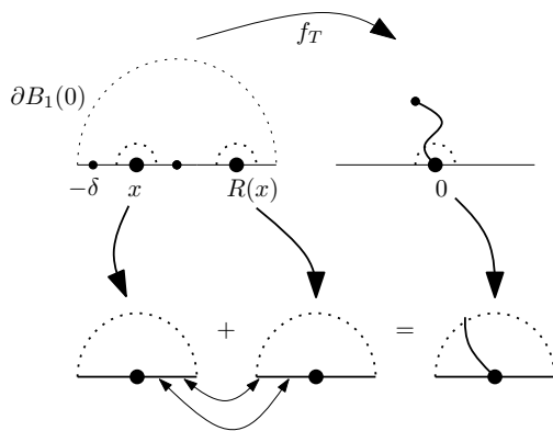
Figure 1.7: Choose h as in Theorem 1.2 (normalized by h_1(0) = 0 ) except with the law of h weighted by \nu_h([- \delta, 0]) for some fixed \delta \in (0, 1) . Then conditioned on h , sample x from \nu_h restricted to [- \delta, 0] (normalized to be a probability measure). Take T so that f_T is the map zipping up [x, 0] with [0, R(x)] . Consider the three random surfaces obtained by choosing a semi-disc of quantum area \tilde{\varepsilon} centered at each of x and R(x) (on the left side) and 0 (on the right side), and multiplying areas by 1/\tilde{\varepsilon} (zooming in) so that all three balls have quantum area 1. In the \tilde{\varepsilon} \rightarrow 0 limit, the left two quantum surfaces become independent \gamma -quantum wedges, and the right is the conformal welding of these two.
