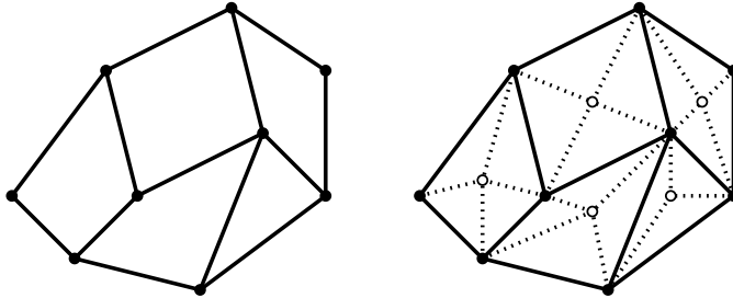
Figure 2.5: An arbitrary planar map can be used to construct a collection of stitched-together unit squares and half unit squares. The result is viewed as a two dimensional manifold with boundary.
