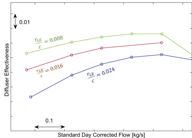
Fig. 17 Impact of diffuser leading edge thickness on diffuser effectiveness. Thicker leading edges lead to more pronounced area reduction at diffuser channel inlet, reducing diffuser effectiveness.
