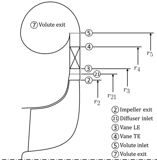
Fig. 1 Meridional view of centrifugal compressor
